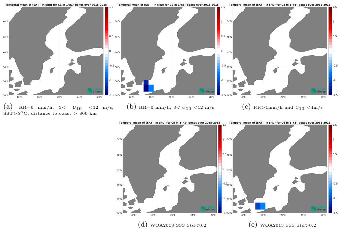
Figure 14: Temporal mean gridded over spatial boxes of size 1^\circ \times 1^\circ of \Delta\text{SSS} (SMOS SSS L4 Baltic v1 - Daily (BEC) - TSG (GOSUD-Research-vessel)) for 5 different subdatasets corresponding to:RR=0 mm/h, 3 < U_{10} < 12 m/s, SST>5°C, distance to coast > 800 km (a), RR=0 mm/h, 3 < U_{10} < 12 m/s (b), RR>1mm/h and U_{10} < 4 m/s (c), WOA2013 SSS Std<0.2 (d), WOA2013 SSS Std>0.2 (e).
