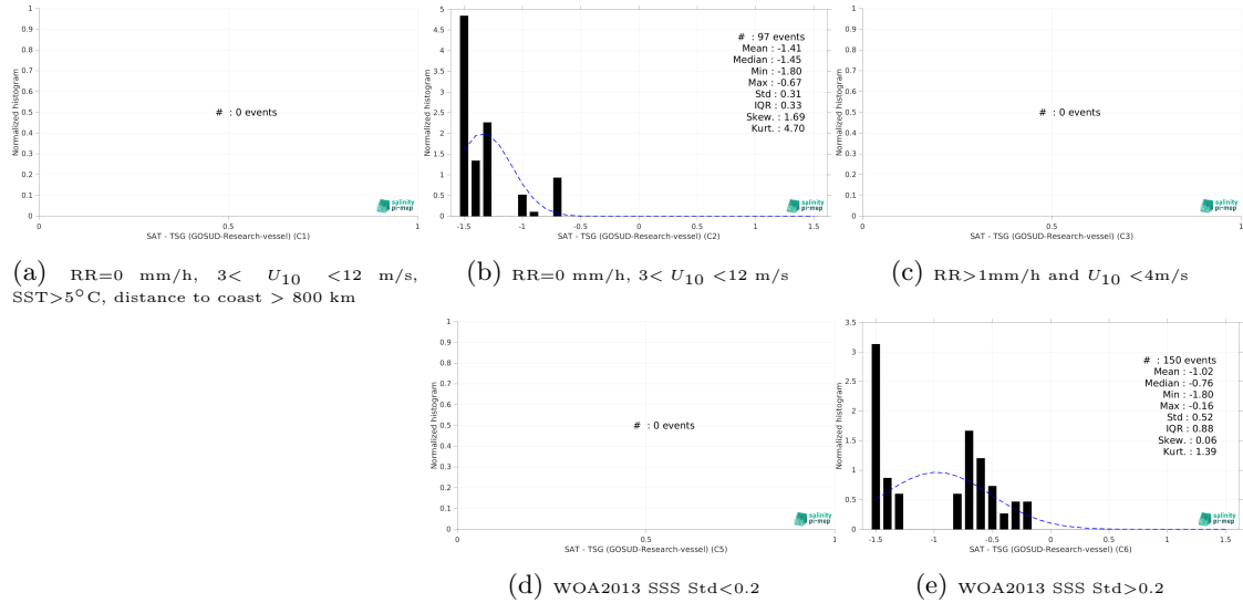
Figure 15: Normalized histogram of \Delta SSS (SMOS SSS L4 Baltic v1 - Daily (BEC) - TSG (GOSUD-Research-vessel)) for 5 different subdatasets corresponding to: RR=0 mm/h, 3 < U_{10} < 12 m/s, SST > 5°C, distance to coast > 800 km (a), RR=0 mm/h, 3 < U_{10} < 12 m/s (b), RR > 1mm/h and U_{10} < 4 m/s (c), WOA2013 SSS Std < 0.2 (d), WOA2013 SSS Std > 0.2 (e).
