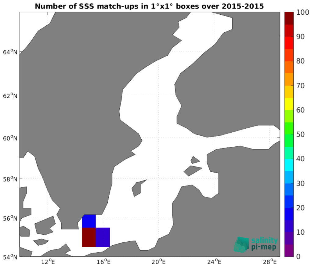
Figure 5: Number of SSS match-ups between TSG (GOSUD-Research-vessel) SSS and the SMOS SSS L4 Baltic v1 - Daily (BEC) SSS product for the Baltic Sea Pi-MEP region over 1°×1° boxes and for the full satellite product period.
