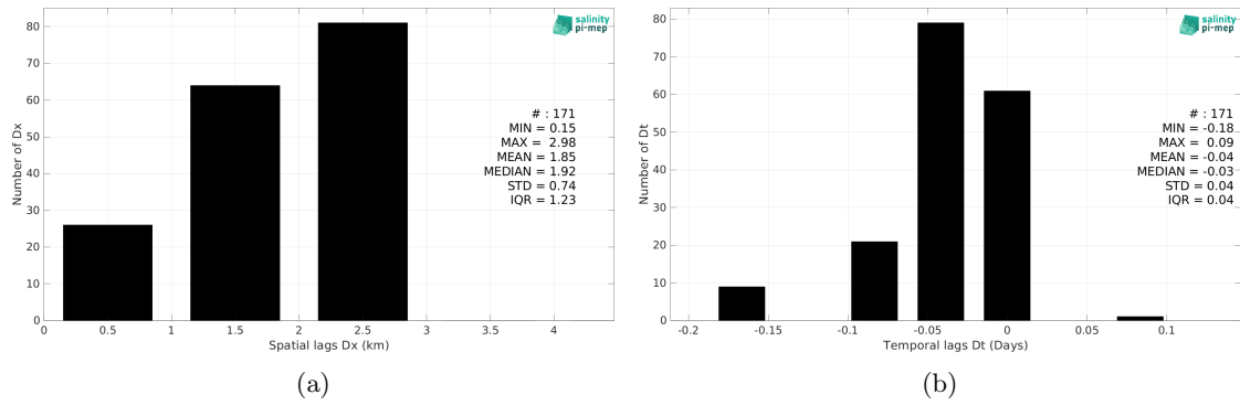
Figure 6: Histograms of the spatial (a) and temporal (b) lags between the location/time of the TSG (GOSUD-Research-vessel) measurement and the date of the corresponding SMOS SSS L4 Baltic v1 - Daily (BEC) SSS pixel.
