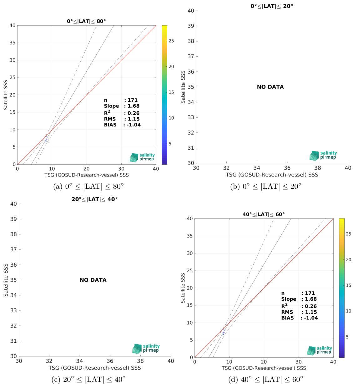
Figure 10: Contour maps of the concentration of SMOS SSS L4 Baltic v1 - Daily (BEC) SSS (y-axis) versus TSG (GOSUD-Research-vessel) SSS (x-axis) at match-up pairs for different latitude bands. For each plot, the red line shows x=y . The black thin and dashed lines indicate a linear fit through the data cloud and the \pm 95\% confidence levels, respectively. The number match-up pairs n , the slope and R^2 coefficient of the linear fit, the root mean square (RMS) and the mean bias between satellite and in situ data are indicated for each latitude band in each plots.
