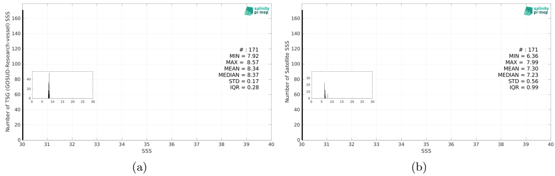
Figure 3: Histograms of SSS from TSG (GOSUD-Research-vessel) (a) and SMOS SSS L4 Baltic v1 - Daily (BEC) (b) considering all match-up pairs per bins of 0.1 over the Baltic Sea Pi-MEP region and for the full satellite product period.
