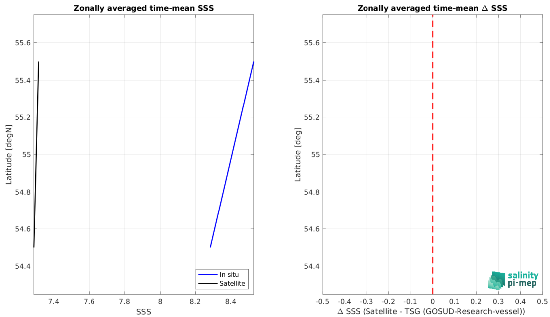
Figure 9: Left panel: Zonal mean SSS from SMOS SSS L4 Baltic v1 - Daily (BEC) satellite product (black) and from TSG (GOSUD-Research-vessel) (blue). Right panel: Zonal mean of \Delta SSS (Satellite - TSG (GOSUD-Research-vessel)) for all the collected Pi-MEP match-up pairs estimated over the full satellite product period.
