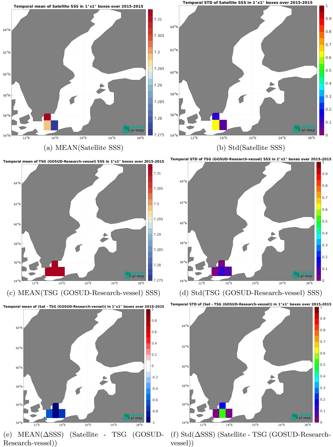
Figure 7: Temporal mean (left) and Std (right) of SSS from SMOS SSS L4 Baltic v1 - Daily (BEC) (top), TSG (GOSUD-Research-vessel) (middle), and of \Delta SSS (Satellite - TSG (GOSUD-Research-vessel)). Only match-up pairs are used to generate these maps.
