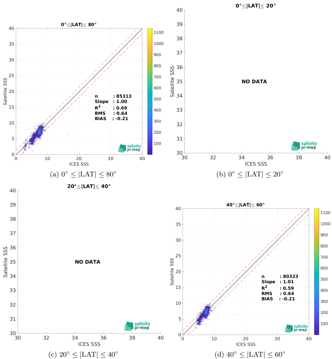
Figure 10: Contour maps of the concentration of SMOS SSS L4 Baltic v1 - Daily (BEC) SSS (y-axis) versus ICES SSS (x-axis) at match-up pairs for different latitude bands. For each plot, the red line shows x=y . The black thin and dashed lines indicate a linear fit through the data cloud and the \pm 95\% confidence levels, respectively. The number match-up pairs n , the slope and R^2 coefficient of the linear fit, the root mean square (RMS) and the mean bias between satellite and in situ data are indicated for each latitude band in each plots.
