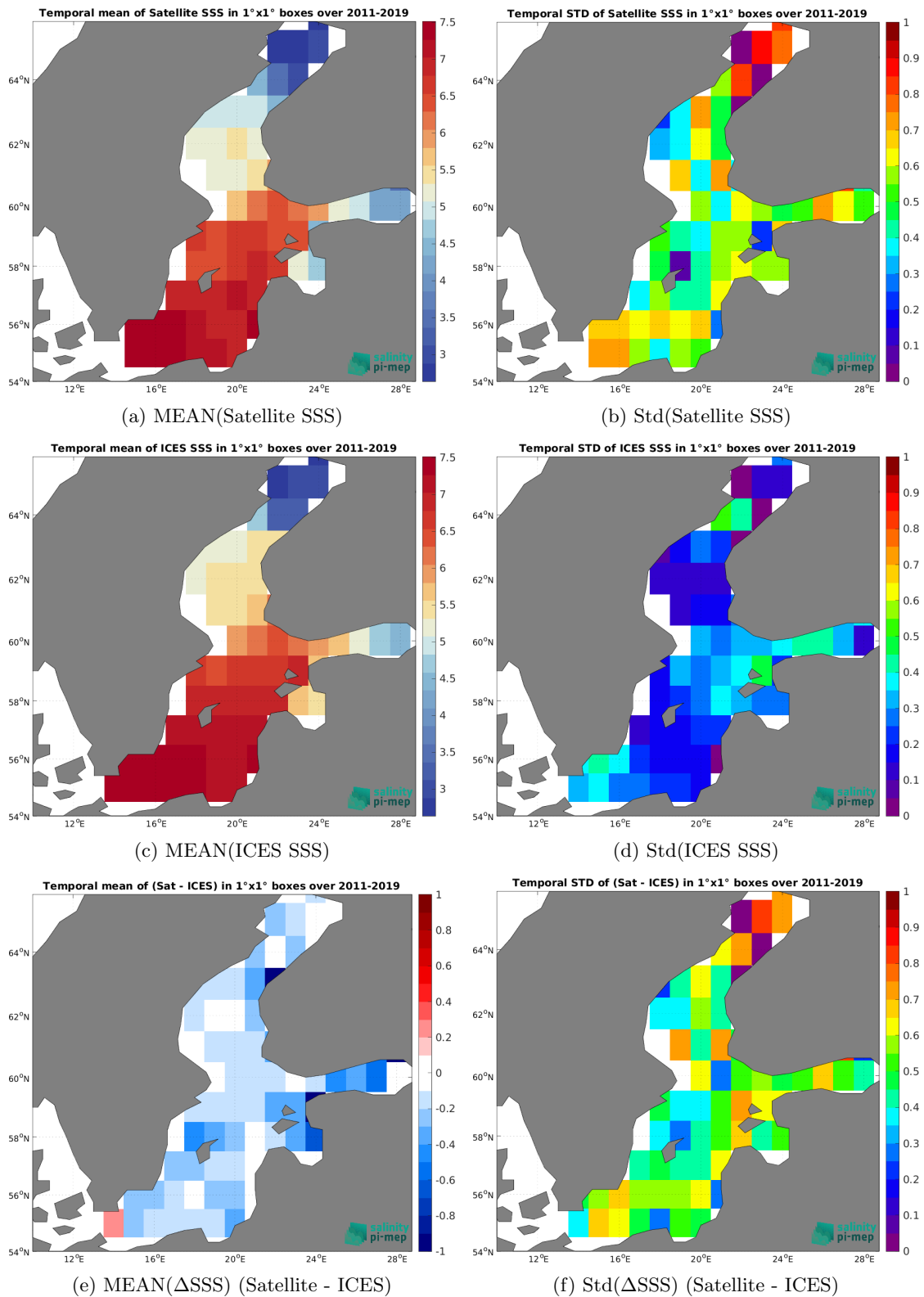
Figure 7: Temporal mean (left) and Std (right) of SSS from SMOS SSS L4 Baltic v1 - Daily (BEC) (top), ICES (middle), and of \Delta SSS (Satellite - ICES). Only match-up pairs are used to generate these maps.
