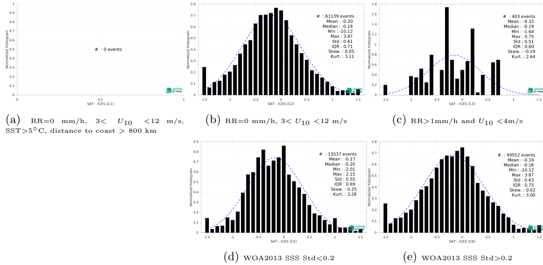
Figure 15: Normalized histogram of \Delta SSS (SMOS SSS L4 Baltic v1 - Daily (BEC) - ICES) for 5 different subdatasets corresponding to: RR=0 mm/h, 3 < U_{10} < 12 m/s, SST > 5°C, distance to coast > 800 km (a), RR=0 mm/h, 3 < U_{10} < 12 m/s (b), RR > 1mm/h and U_{10} < 4 m/s (c), WOA2013 SSS Std < 0.2 (d), WOA2013 SSS Std > 0.2 (e).
