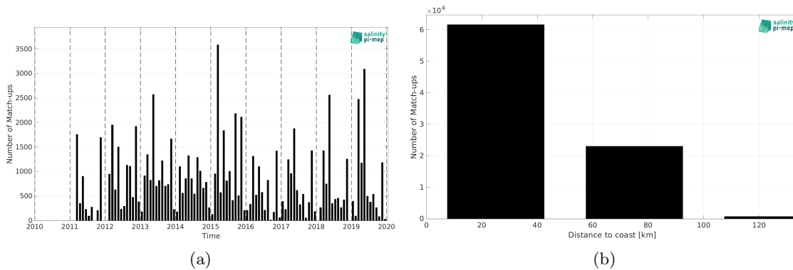
Figure 2: Number of match-ups between ICES and SMOS SSS L4 Baltic v1 - Daily (BEC) SSS as a function of time (a) and as function of the distance to coast (b) over the Baltic Sea Pi-MEP region and for the full satellite product period.
