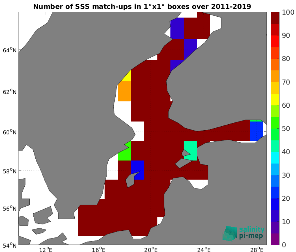
Figure 5: Number of SSS match-ups between ICES SSS and the SMOS SSS L4 Baltic v1 - Daily (BEC) SSS product for the Baltic Sea Pi-MEP region over 1°x1° boxes and for the full satellite product period.
