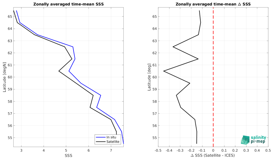
Figure 9: Left panel: Zonal mean SSS from SMOS SSS L4 Baltic v1 - Daily (BEC) satellite product (black) and from ICES (blue). Right panel: Zonal mean of \Delta SSS (Satellite - ICES) for all the collected Pi-MEP match-up pairs estimated over the full satellite product period.
