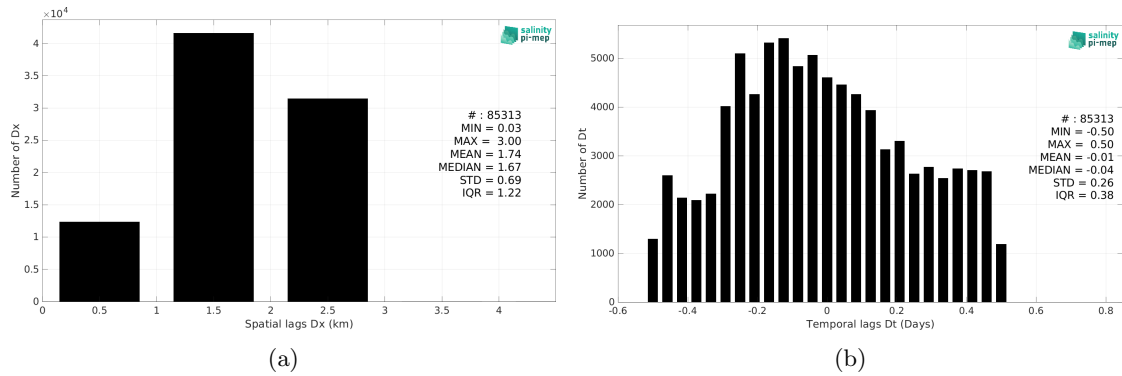
Figure 6: Histograms of the spatial (a) and temporal (b) lags between the location/time of the ICES measurement and the date of the corresponding SMOS SSS L4 Baltic v1 - Daily (BEC) SSS pixel.
