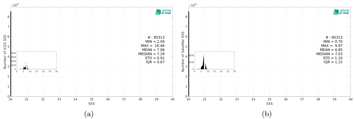
Figure 3: Histograms of SSS from ICES (a) and SMOS SSS L4 Baltic v1 - Daily (BEC) (b) considering all match-up pairs per bins of 0.1 over the Baltic Sea Pi-MEP region and for the full satellite product period.
