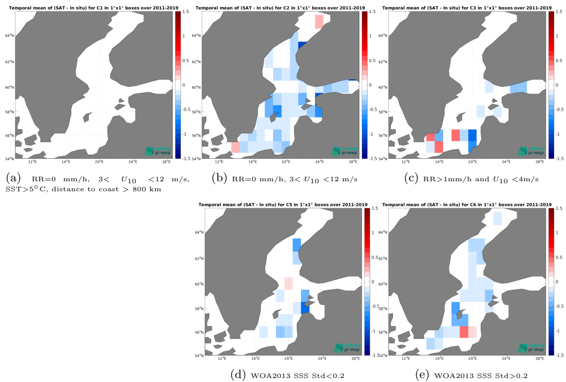
Figure 14: Temporal mean gridded over spatial boxes of size 1^\circ \times 1^\circ of \Delta SSS (SMOS SSS L4 Baltic v1 - Daily (BEC) - ICES) for 5 different subdatasets corresponding to:RR=0 mm/h, 3 < U_{10} < 12 m/s, SST >5^\circ\text{C} , distance to coast > 800 km (a), RR=0 mm/h, 3 < U_{10} < 12 m/s (b), RR >1 mm/h and U_{10} < 4 m/s (c), WOA2013 SSS Std <0.2 (d), WOA2013 SSS Std >0.2 (e).
