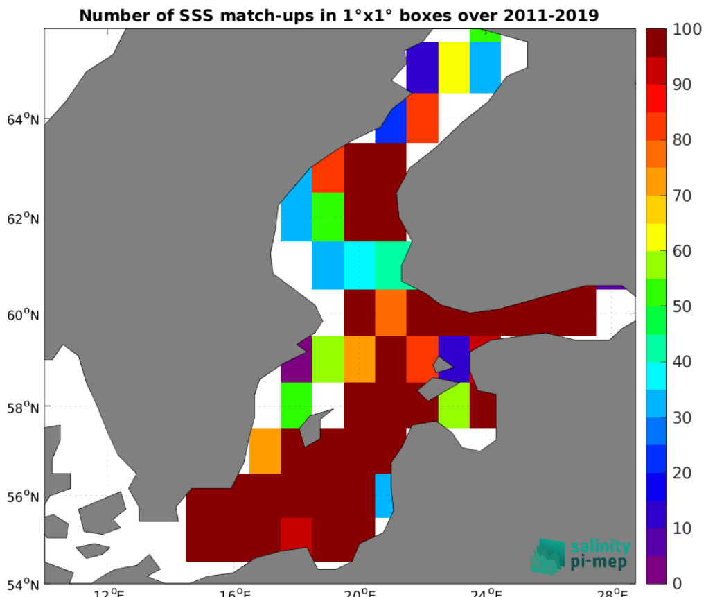
Figure 4: Number of SSS match-ups between ICES SSS and the SMOS SSS L4 Baltic v1 - Daily (BEC) SSS product for the Baltic Sea Pi-MEP region over 1^\circ \times 1^\circ boxes and for the full satellite product period.
