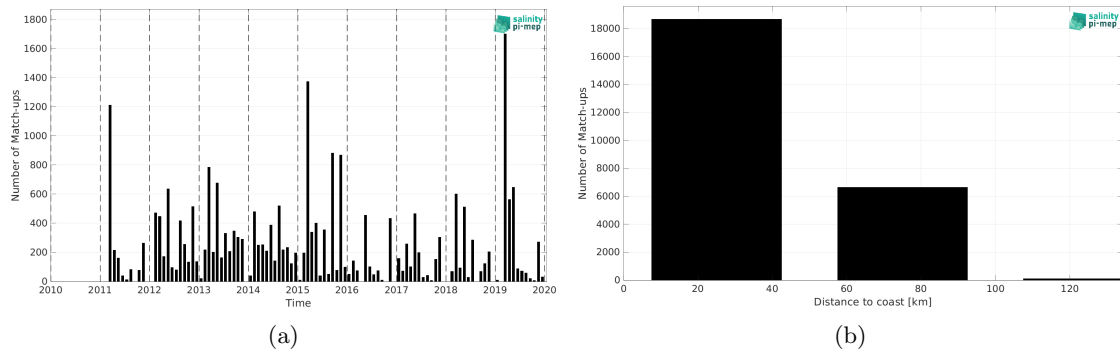
Figure 1: Number of match-ups between ICES and SMOS SSS L4 Baltic v1 - Daily (BEC) SSS as a function of time (a) and as function of the distance to coast (b) over the Baltic Sea Pi-MEP region and for the full satellite product period.
