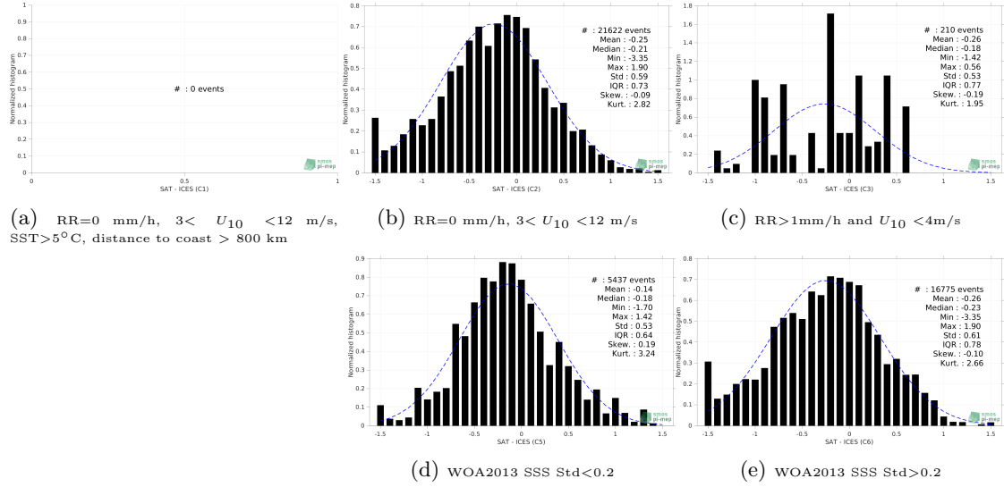
Figure 13: Normalized histogram of \Delta SSS (SMOS SSS L4 Baltic v1 - Daily (BEC) - ICES) for 5 different subdatasets corresponding to: RR=0 mm/h, 3 < U_{10} < 12 m/s, SST > 5°C, distance to coast > 800 km (a), RR=0 mm/h, 3 < U_{10} < 12 m/s (b), RR > 1mm/h and U_{10} < 4 m/s (c), WOA2013 SSS Std < 0.2 (d), WOA2013 SSS Std > 0.2 (e).
