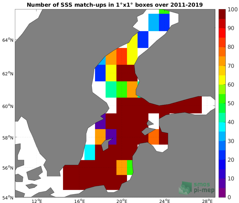
Figure 4: Number of SSS match-ups between ICES SSS and the SMOS SSS L4 Baltic v1 - Daily (BEC) SSS product for the Baltic Sea Pi-MEP region over 1°×1° boxes and for the full satellite product period.
