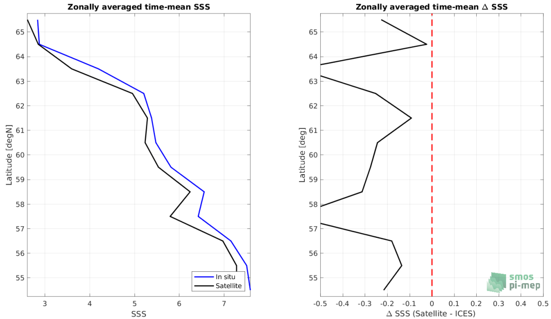
Figure 8: Left panel: Zonal mean SSS from SMOS SSS L4 Baltic v1 - Daily (BEC) satellite product (black) and from ICES (blue). Right panel: Zonal mean of \Delta SSS (Satellite - ICES) for all the collected Pi-MEP match-up pairs estimated over the full satellite product period.
