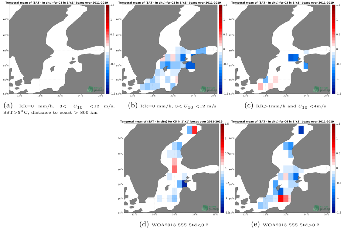
Figure 12: Temporal mean gridded over spatial boxes of size 1^{\circ}\times 1^{\circ} of \Delta\text{SSS} (SMOS SSS L4 Baltic v1 - Daily (BEC) - ICES) for 5 different subdatasets corresponding to:RR=0 mm/h, 3 < U_{10} < 12 m/s, SST >5^{\circ}\text{C} , distance to coast > 800 km (a), RR=0 mm/h, 3 < U_{10} < 12 m/s (b), RR >1 mm/h and U_{10} < 4 m/s (c), WOA2013 SSS Std <0.2 (d), WOA2013 SSS Std >0.2 (e).
