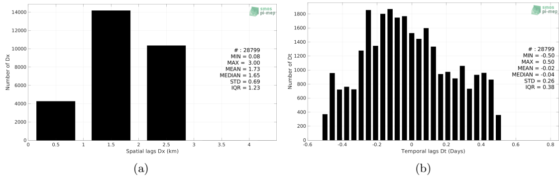
Figure 5: Histograms of the spatial (a) and temporal (b) lags between the location/time of the ICES measurement and the date of the corresponding SMOS SSS L4 Baltic v1 - Daily (BEC) SSS pixel.
