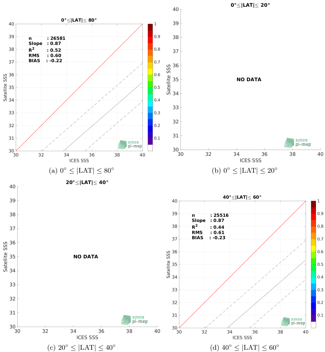
Figure 9: Contour maps of the concentration of SMOS SSS L4 Baltic v1 - Daily (BEC) SSS (y-axis) versus ICES SSS (x-axis) at match-up pairs for different latitude bands. For each plot, the red line shows x=y . The black thin and dashed lines indicate a linear fit through the data cloud and the \pm 95\% confidence levels, respectively. The number match-up pairs n , the slope and R^2 coefficient of the linear fit, the root mean square (RMS) and the mean bias between satellite and in situ data are indicated for each latitude band in each plots.
