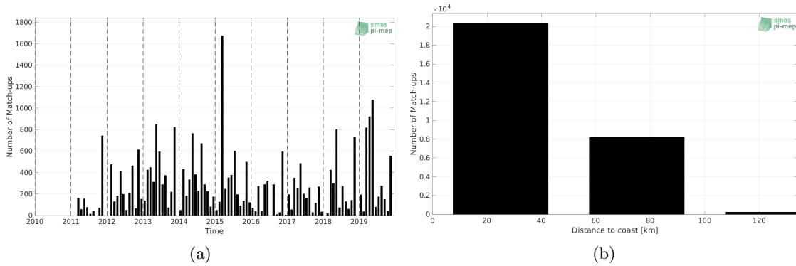
Figure 1: Number of match-ups between ICES and SMOS SSS L4 Baltic v1 - Daily (BEC) SSS as a function of time (a) and as function of the distance to coast (b) over the Baltic Sea Pi-MEP region and for the full satellite product period.
