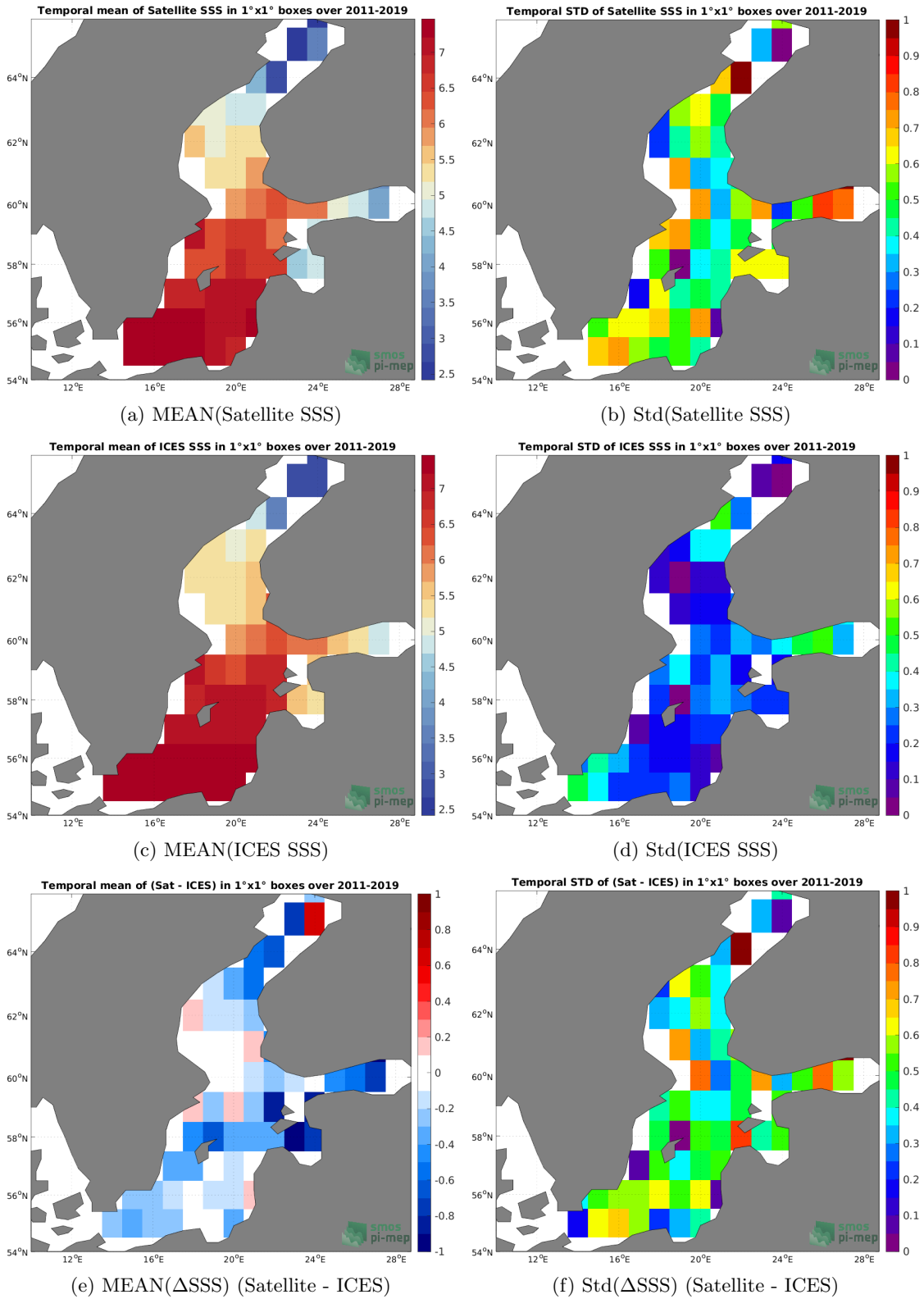
Figure 6: Temporal mean (left) and Std (right) of SSS from SMOS SSS L4 Baltic v1 - Daily (BEC) (top), ICES (middle), and of \Delta SSS (Satellite - ICES). Only match-up pairs are used to generate these maps.
