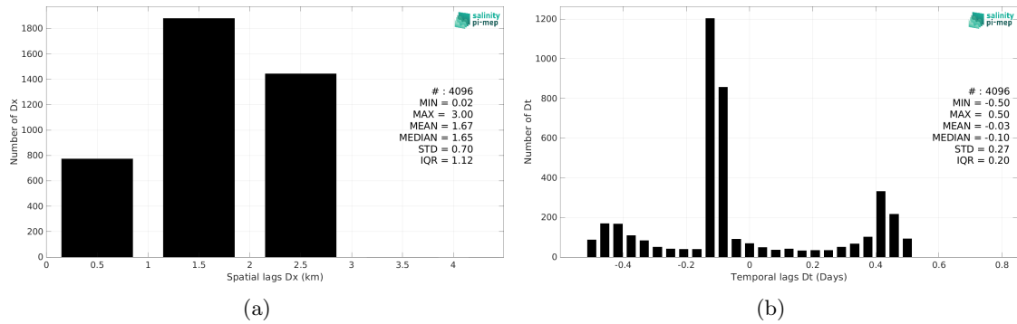
Figure 6: Histograms of the spatial (a) and temporal (b) lags between the location/time of the Argo measurement and the date of the corresponding SMOS SSS L4 Baltic v1 - Daily (BEC) SSS pixel.
