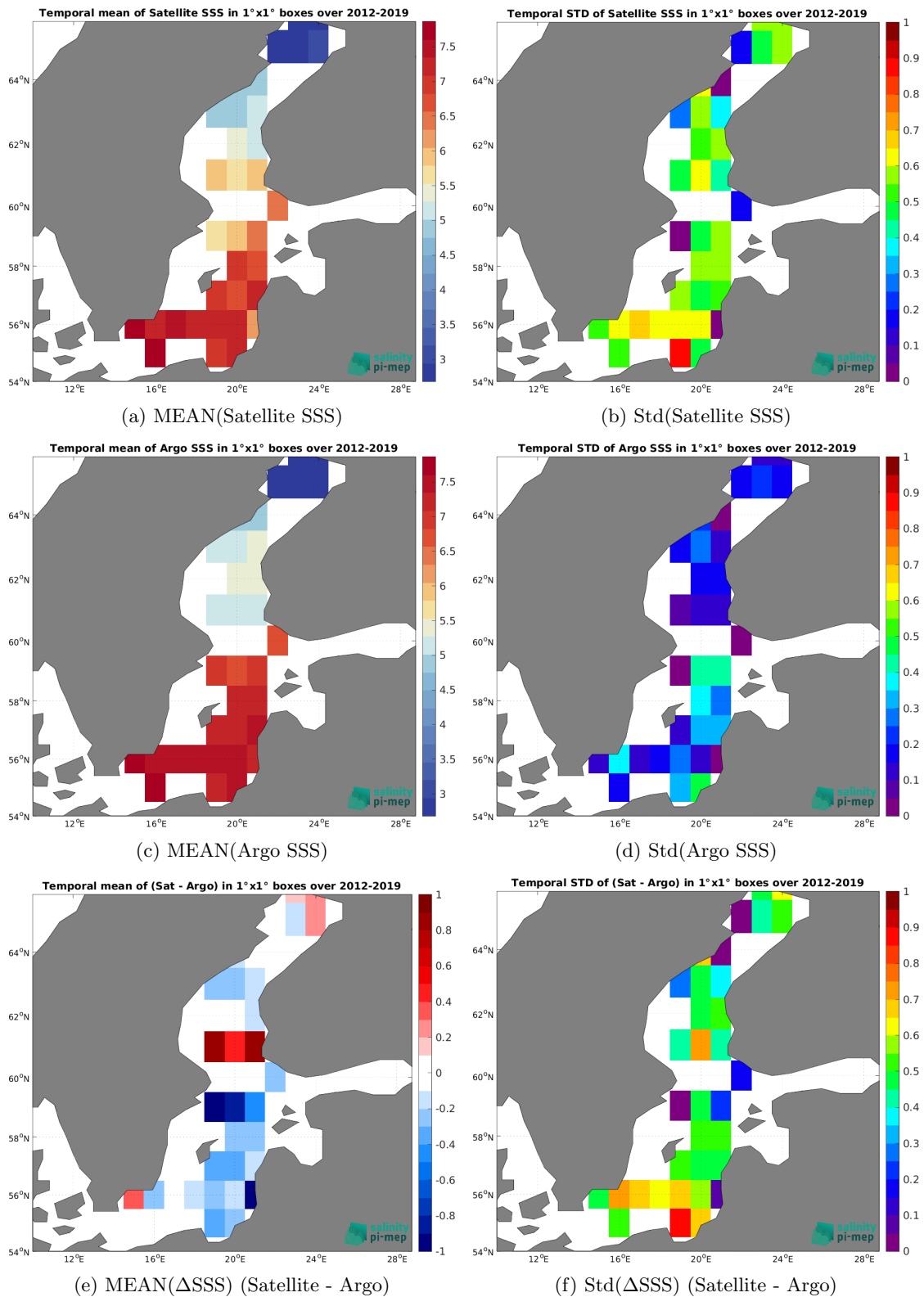
Figure 7: Temporal mean (left) and Std (right) of SSS from SMOS SSS L4 Baltic v1 - Daily (BEC) (top), Argo (middle), and of \Delta SSS (Satellite - Argo). Only match-up pairs are used to generate these maps.
