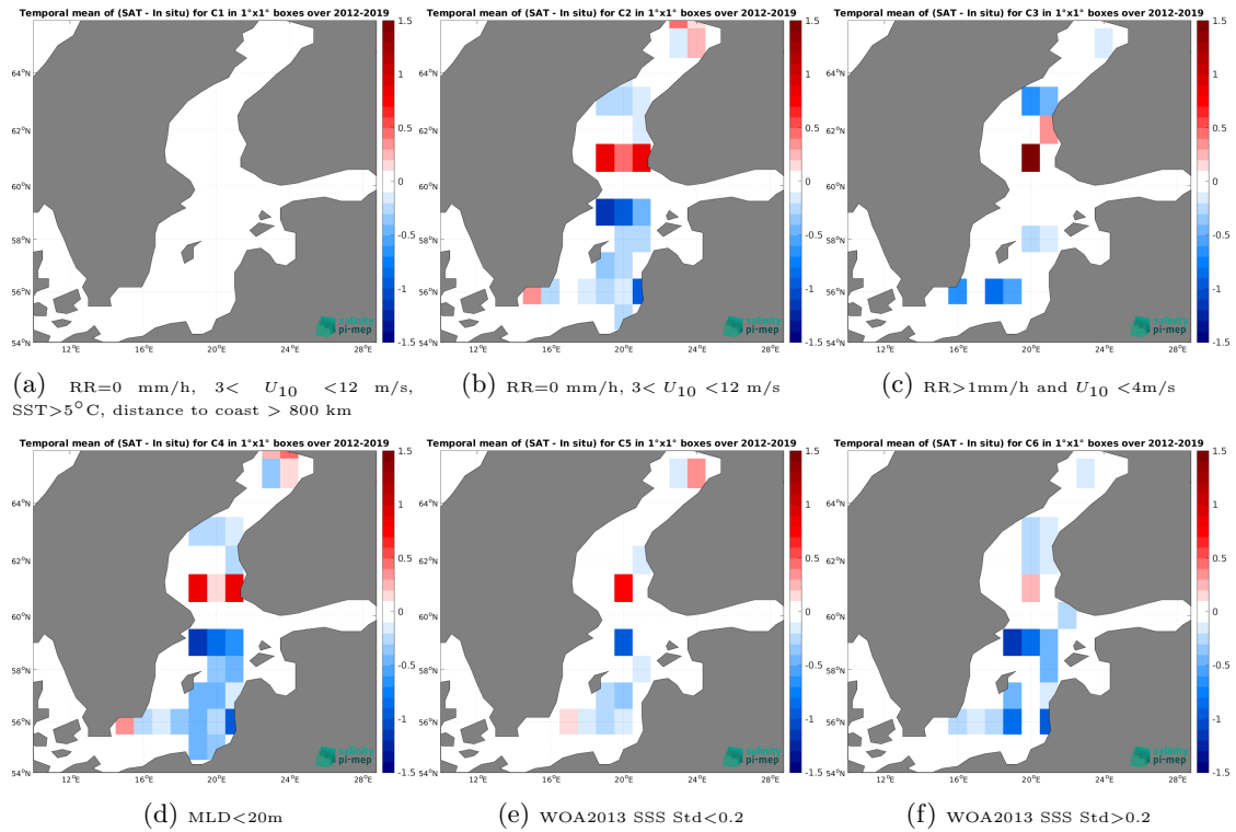
Figure 14: Temporal mean gridded over spatial boxes of size 1^\circ \times 1^\circ of \Delta SSS (SMOS SSS L4 Baltic v1 - Daily (BEC) - Argo) for 6 different subdatasets corresponding to:RR=0 mm/h, 3 < U_{10} < 12 m/s, SST>5°C, distance to coast > 800 km (a), RR=0 mm/h, 3 < U_{10} < 12 m/s (b), RR>1mm/h and U_{10} < 4 m/s (c),MLD<20m (d),WOA2013 SSS Std<0.2 (e),WOA2013 SSS Std>0.2 (f).
