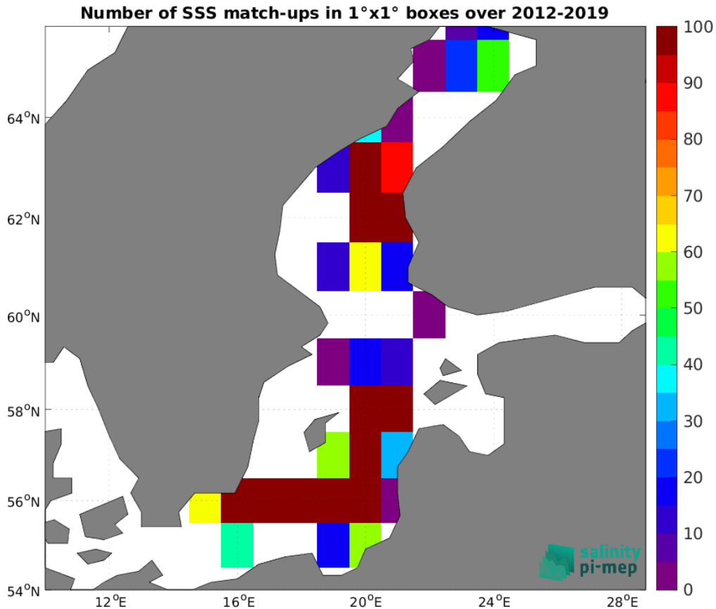
Figure 5: Number of SSS match-ups between Argo SSS and the SMOS SSS L4 Baltic v1 - Daily (BEC) SSS product for the Baltic Sea Pi-MEP region over 1^\circ \times 1^\circ boxes and for the full satellite product period.
