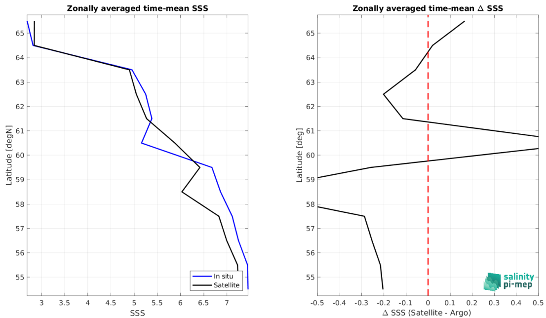
Figure 9: Left panel: Zonal mean SSS from SMOS SSS L4 Baltic v1 - Daily (BEC) satellite product (black) and from Argo (blue). Right panel: Zonal mean of \Delta SSS (Satellite - Argo) for all the collected Pi-MEP match-up pairs estimated over the full satellite product period.
