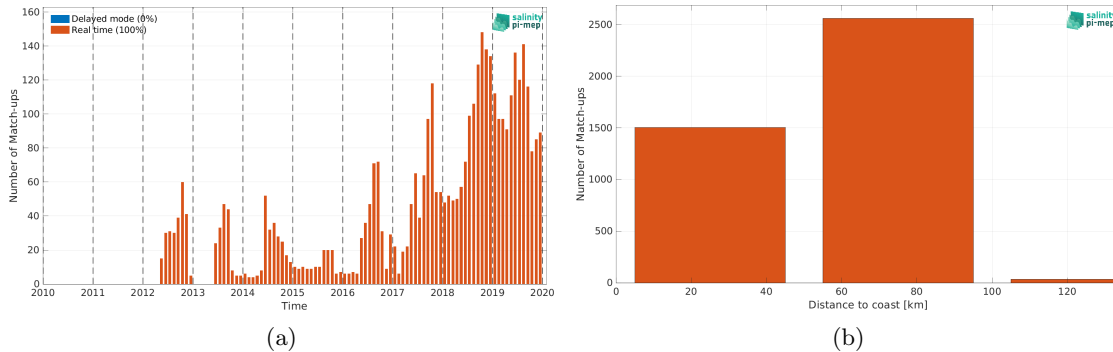
Figure 2: Number of match-ups between Argo and SMOS SSS L4 Baltic v1 - Daily (BEC) SSS as a function of time (a) and as function of the distance to coast (b) over the Baltic Sea Pi-MEP region and for the full satellite product period.
