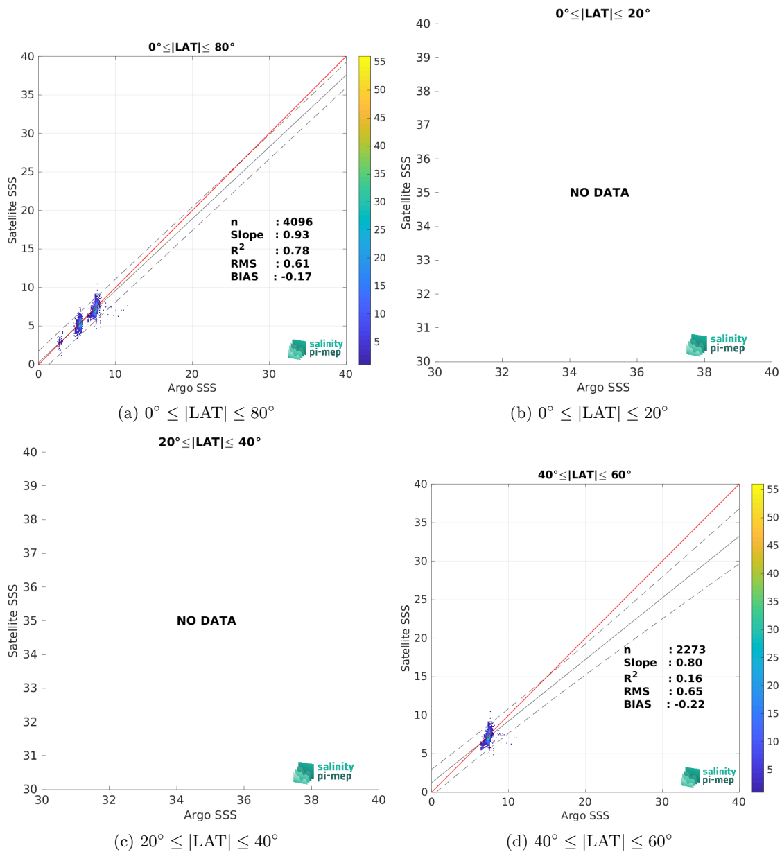
Figure 10: Contour maps of the concentration of SMOS SSS L4 Baltic v1 - Daily (BEC) SSS (y-axis) versus Argo SSS (x-axis) at match-up pairs for different latitude bands. For each plot, the red line shows x=y . The black thin and dashed lines indicate a linear fit through the data cloud and the \pm 95\% confidence levels, respectively. The number match-up pairs n , the slope and R^2 coefficient of the linear fit, the root mean square (RMS) and the mean bias between satellite and in situ data are indicated for each latitude band in each plot.
