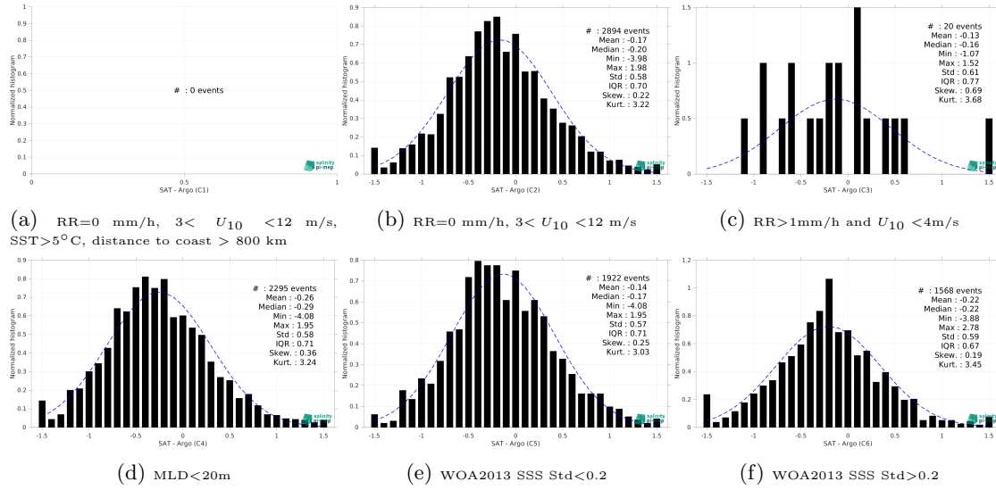
Figure 15: Normalized histogram of \Delta SSS (SMOS SSS L4 Baltic v1 - Daily (BEC) - Argo) for 6 different subdatasets corresponding to: RR=0 mm/h, 3 < U_{10} < 12 m/s, SST>5°C, distance to coast > 800 km (a), RR=0 mm/h, 3 < U_{10} < 12 m/s (b), RR>1mm/h and U_{10} < 4 m/s (c), MLD<20m (d), WOA2013 SSS Std<0.2 (e), WOA2013 SSS Std>0.2 (f).
