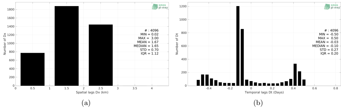
Figure 5: Histograms of the spatial (a) and temporal (b) lags between the location/time of the Argo measurement and the date of the corresponding SMOS SSS L4 Baltic v1 - Daily (BEC) SSS pixel.
