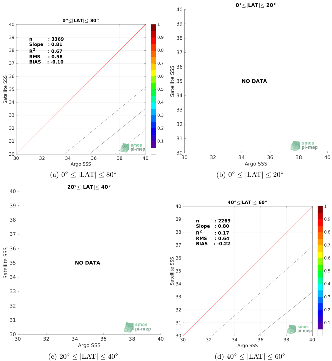
Figure 9: Contour maps of the concentration of SMOS SSS L4 Baltic v1 - Daily (BEC) SSS (y-axis) versus Argo SSS (x-axis) at match-up pairs for different latitude bands. For each plot, the red line shows x=y . The black thin and dashed lines indicate a linear fit through the data cloud and the \pm 95\% confidence levels, respectively. The number match-up pairs n , the slope and R^2 coefficient of the linear fit, the root mean square (RMS) and the mean bias between satellite and in situ data are indicated for each latitude band in each plots.
