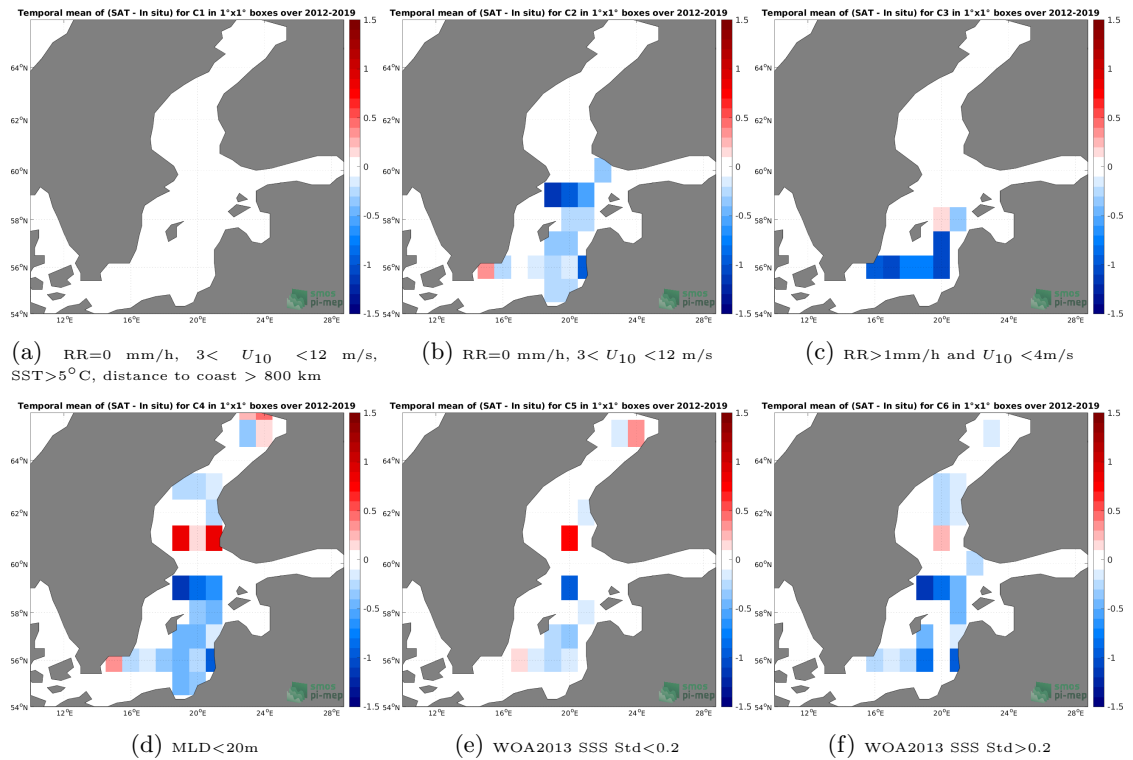
Figure 12: Temporal mean gridded over spatial boxes of size 1^{\circ}\times 1^{\circ} of \Delta\text{SSS} (SMOS SSS L4 Baltic v1 - Daily (BEC) - Argo) for 6 different subdatasets corresponding to:RR=0 mm/h, 3 < U_{10} < 12 m/s, SST >5^{\circ}\text{C} , distance to coast > 800 km (a), RR=0 mm/h, 3 < U_{10} < 12 m/s (b), RR >1\text{mm/h} and U_{10} < 4\text{m/s} (c),MLD <20\text{m} (d),WOA2013 SSS Std <0.2 (e),WOA2013 SSS Std >0.2 (f).
