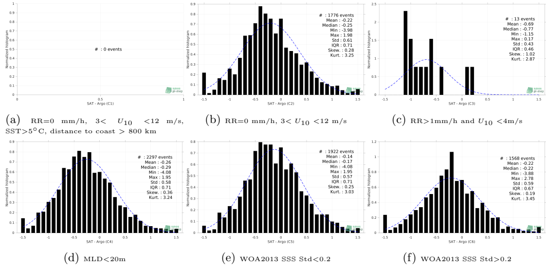
Figure 13: Normalized histogram of \Delta SSS (SMOS SSS L4 Baltic v1 - Daily (BEC) - Argo) for 6 different subdatasets corresponding to: RR=0 mm/h, 3 < U_{10} < 12 m/s, SST>5°C, distance to coast > 800 km (a), RR=0 mm/h, 3 < U_{10} < 12 m/s (b), RR>1mm/h and U_{10} < 4 m/s (c), MLD<20m (d), WOA2013 SSS Std<0.2 (e), WOA2013 SSS Std>0.2 (f).
