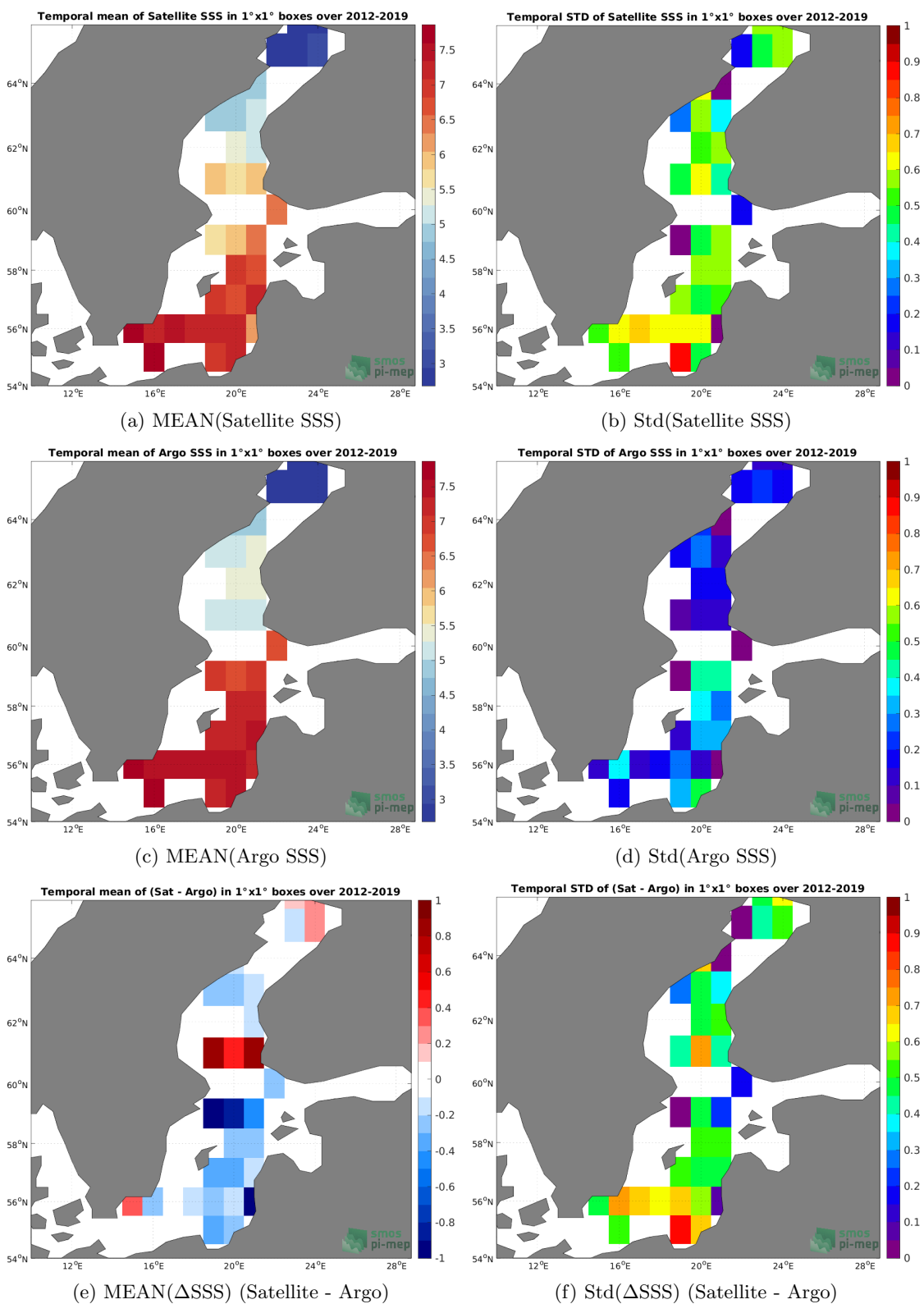
Figure 6: Temporal mean (left) and Std (right) of SSS from SMOS SSS L4 Baltic v1 - Daily (BEC) (top), Argo (middle), and of \Delta SSS (Satellite - Argo). Only match-up pairs are used to generate these maps.
