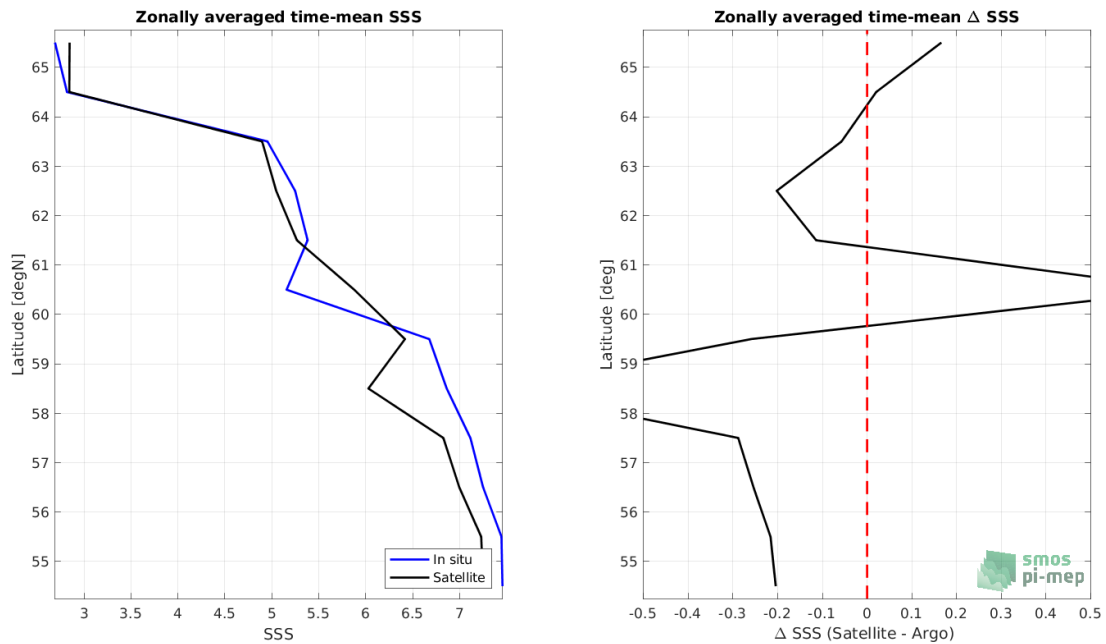
Figure 8: Left panel: Zonal mean SSS from SMOS SSS L4 Baltic v1 - Daily (BEC) satellite product (black) and from Argo (blue). Right panel: Zonal mean of \Delta SSS (Satellite - Argo) for all the collected Pi-MEP match-up pairs estimated over the full satellite product period.
