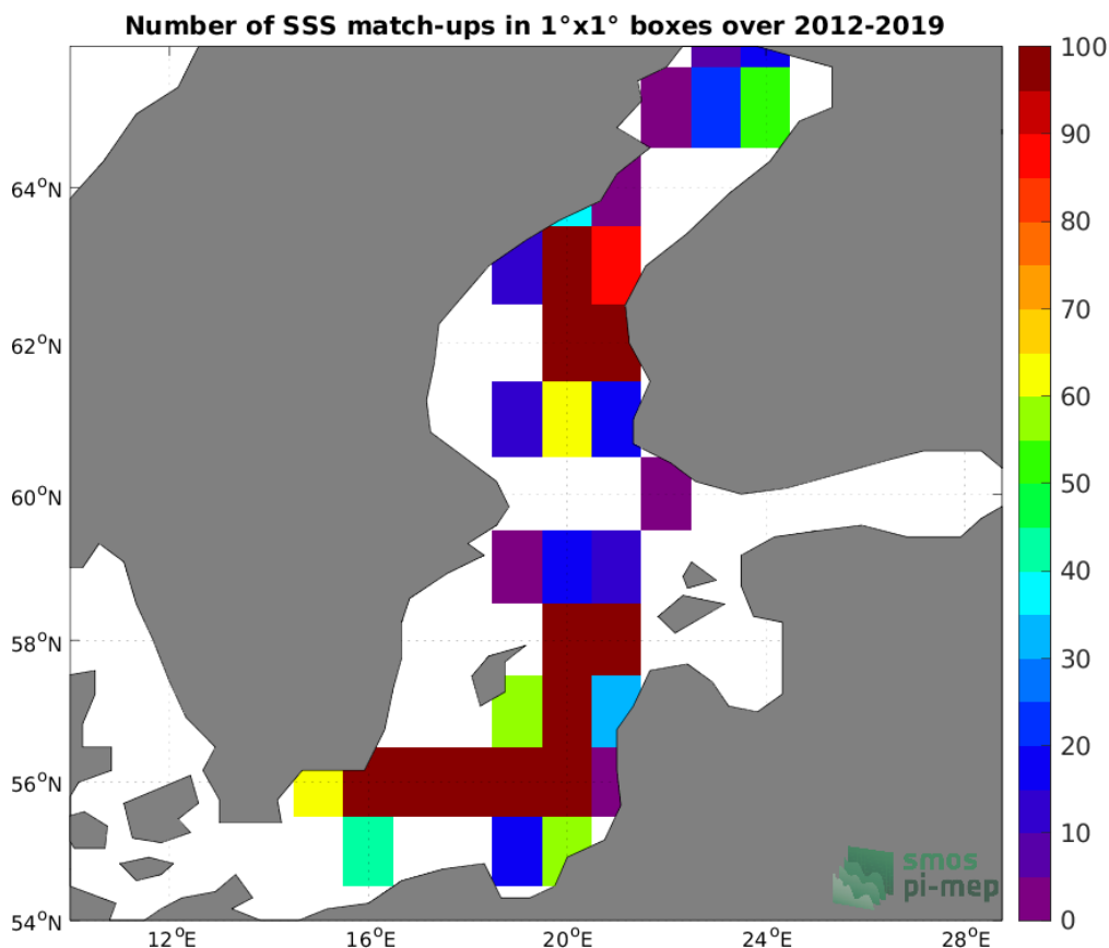
Figure 4: Number of SSS match-ups between Argo SSS and the SMOS SSS L4 Baltic v1 - Daily (BEC) SSS product for the Baltic Sea Pi-MEP region over 1^\circ \times 1^\circ boxes and for the full satellite product period.
