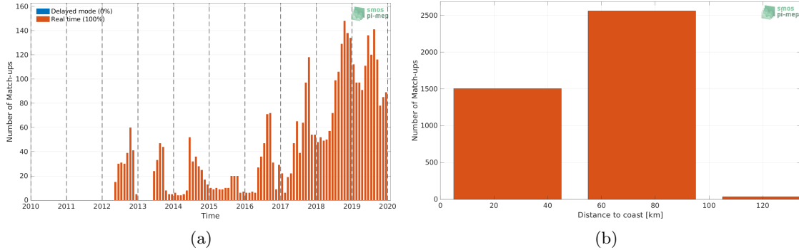
Figure 1: Number of match-ups between Argo and SMOS SSS L4 Baltic v1 - Daily (BEC) SSS as a function of time (a) and as function of the distance to coast (b) over the Baltic Sea Pi-MEP region and for the full satellite product period.
