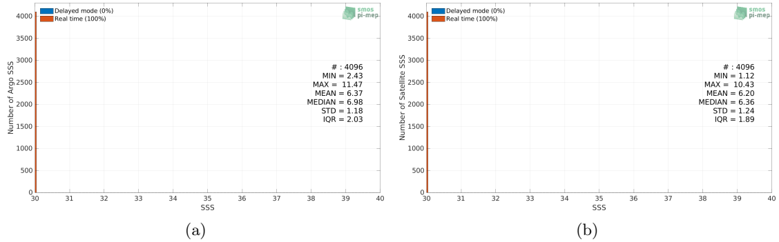
Figure 2: Histograms of SSS from Argo (a) and SMOS SSS L4 Baltic v1 - Daily (BEC) (b) considering all match-up pairs per bins of 0.1 over the Baltic Sea Pi-MEP region and for the full satellite product period.
