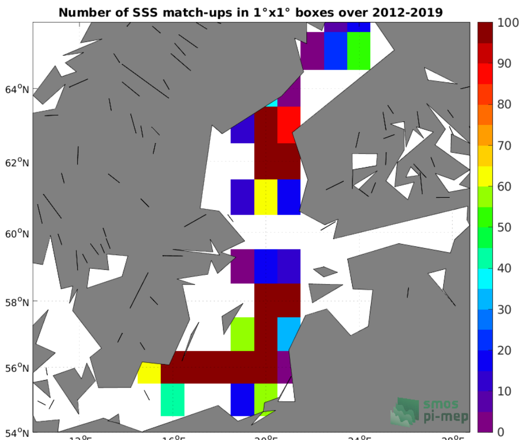
Figure 4: Number of SSS match-ups between Argo SSS and the SMOS SSS L4 Baltic v1 - Daily (BEC) SSS product for the Baltic Sea Pi-MEP region over 1°×1° boxes and for the full satellite product period.
