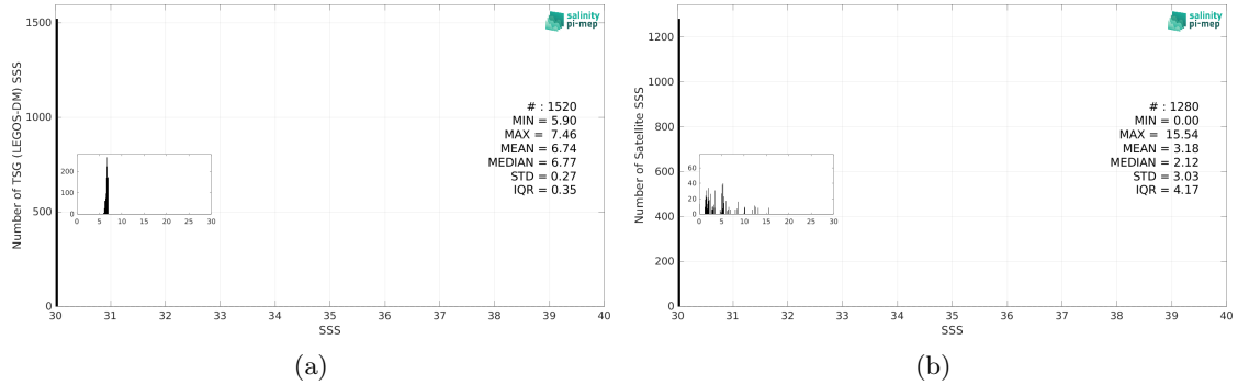
Figure 3: Histograms of SSS from TSG (LEGOS-DM) (a) and SMOS SSS L2Q v331 - With FLAG (CMEMS-CATDS-CPDC) (b) considering all match-up pairs per bins of 0.1 over the Baltic Sea Pi-MEP region and for the full satellite product period.
