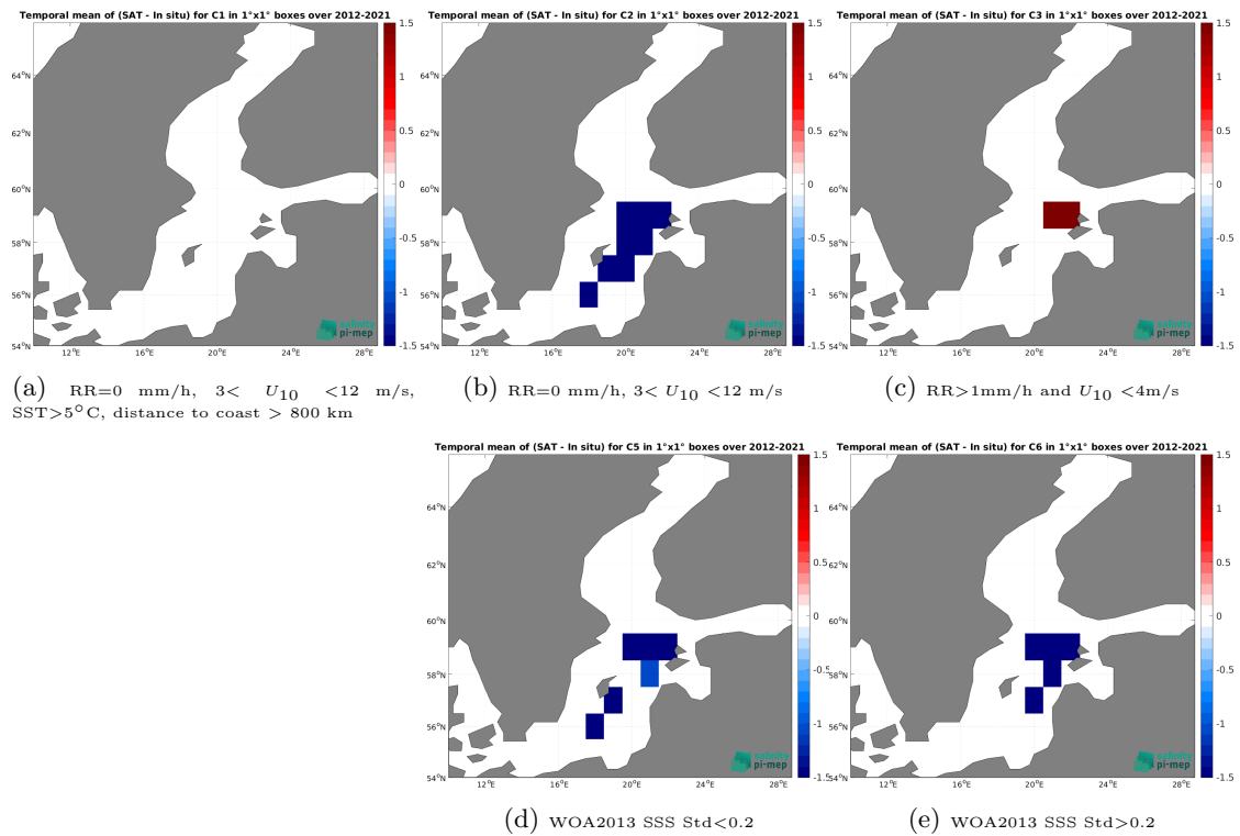
Figure 14: Temporal mean gridded over spatial boxes of size 1^\circ \times 1^\circ of \Delta\text{SSS} (SMOS SSS L2Q v331 - With FLAG (CMEMS-CATDS-CPDC) - TSG (LEGOS-DM)) for 5 different subdatasets corresponding to:RR=0 mm/h, 3 < U_{10} < 12 m/s, SST >5^\circ\text{C} , distance to coast > 800 km (a), RR=0 mm/h, 3 < U_{10} < 12 m/s (b), RR >1 mm/h and U_{10} < 4 m/s (c), WOA2013 SSS Std <0.2 (d), WOA2013 SSS Std >0.2 (e).
