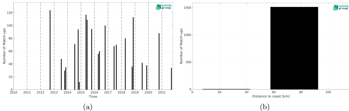
Figure 2: Number of match-ups between TSG (LEGOS-DM) and SMOS SSS L2Q v331 - With FLAG (CMEMS-CATDS-CPDC) SSS as a function of time (a) and as function of the distance to coast (b) over the Baltic Sea Pi-MEP region and for the full satellite product period.
