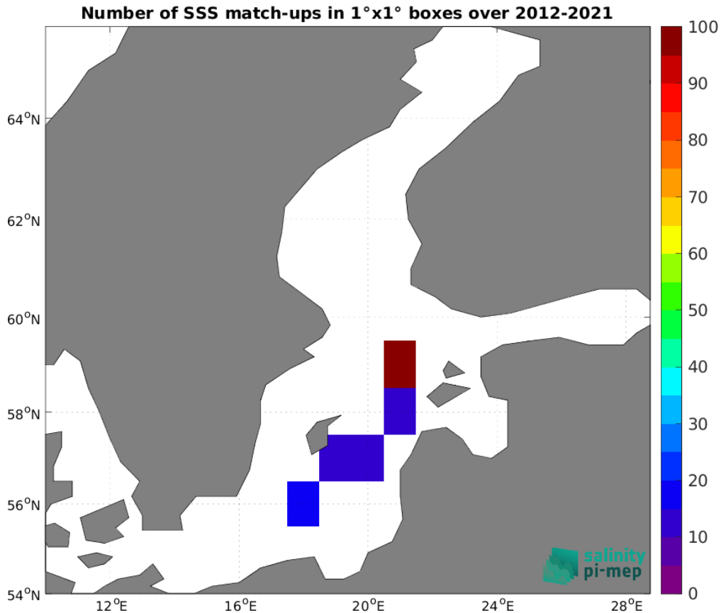
Figure 5: Number of SSS match-ups between TSG (LEGOS-DM) SSS and the SMOS SSS L2Q v331 - With FLAG (CMEMS-CATDS-CPDC) SSS product for the Baltic Sea Pi-MEP region over 1^\circ \times 1^\circ boxes and for the full satellite product period.
