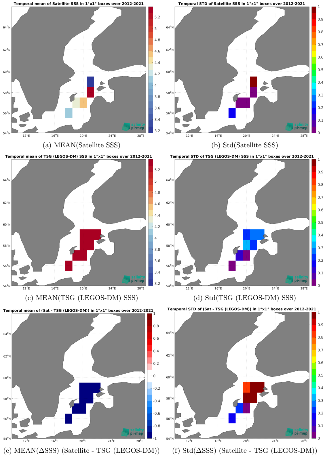
Figure 7: Temporal mean (left) and Std (right) of SSS from SMOS SSS L2Q v331 - With FLAG (CMEMS-CATDS-CPDC) (top), TSG (LEGOS-DM) (middle), and of \Delta SSS (Satellite - TSG (LEGOS-DM)). Only match-up pairs are used to generate these maps.
