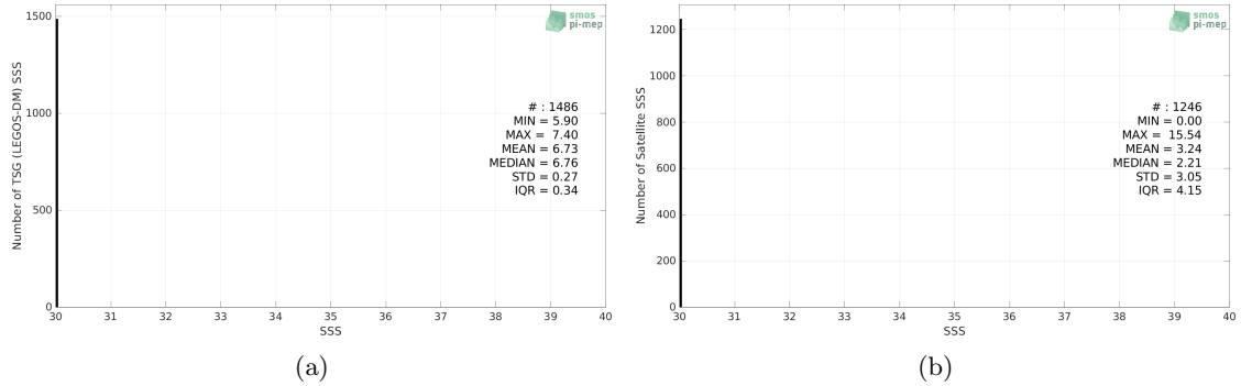
Figure 2: Histograms of SSS from TSG (LEGOS-DM) (a) and SMOS SSS L2Q v331 - With FLAG (CMEMS-CATDS-CPDC) (b) considering all match-up pairs per bins of 0.1 over the Baltic Sea Pi-MEP region and for the full satellite product period.
