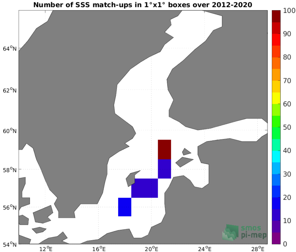
Figure 4: Number of SSS match-ups between TSG (LEGOS-DM) SSS and the SMOS SSS L2Q v331 - With FLAG (CMEMS-CATDS-CPDC) SSS product for the Baltic Sea Pi-MEP region over 1^\circ \times 1^\circ boxes and for the full satellite product period.
