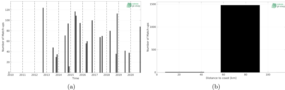
Figure 1: Number of match-ups between TSG (LEGOS-DM) and SMOS SSS L2Q v331 - With FLAG (CMEMS-CATDS-CPDC) SSS as a function of time (a) and as function of the distance to coast (b) over the Baltic Sea Pi-MEP region and for the full satellite product period.
