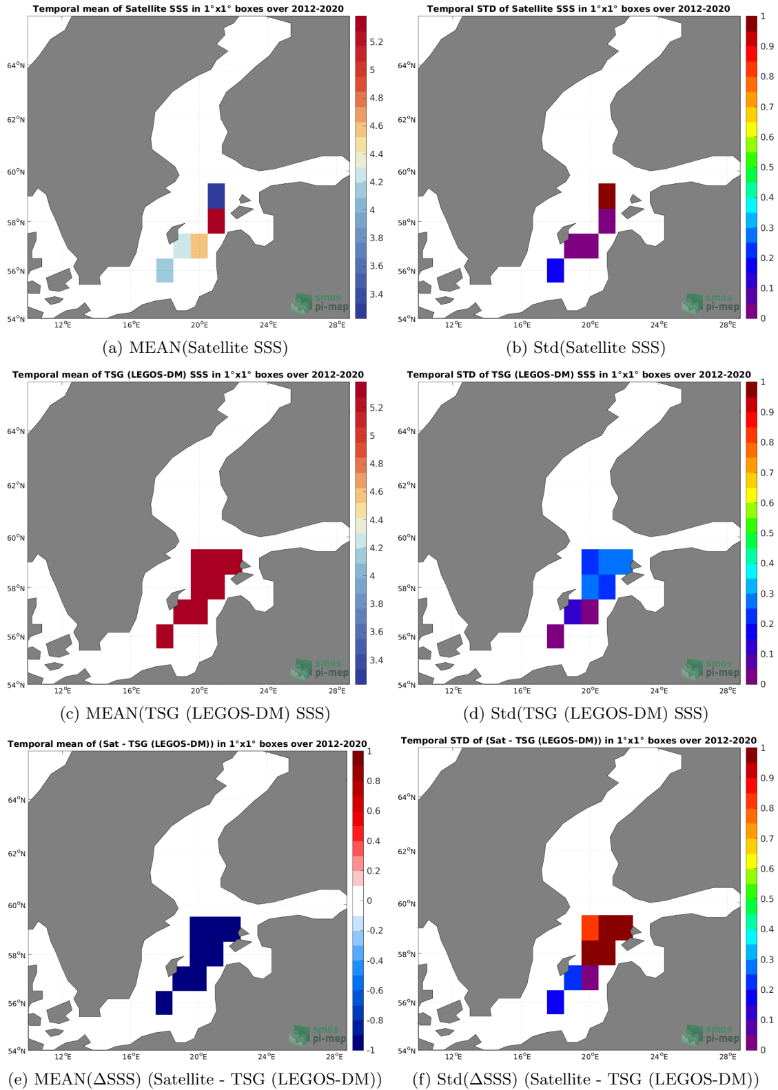
Figure 6: Temporal mean (left) and Std (right) of SSS from SMOS SSS L2Q v331 - With FLAG (CMEMS-CATDS-CPDC) (top), TSG (LEGOS-DM) (middle), and of \Delta SSS (Satellite - TSG (LEGOS-DM)). Only match-up pairs are used to generate these maps.
