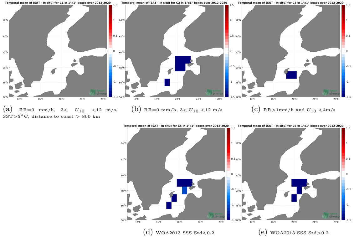
Figure 12: Temporal mean gridded over spatial boxes of size 1^{\circ}\times 1^{\circ} of \Delta\text{SSS} (SMOS SSS L2Q v331 - With FLAG (CMEMS-CATDS-CPDC) - TSG (LEGOS-DM)) for 5 different subdatasets corresponding to:RR=0 mm/h, 3 < U_{10} < 12 m/s, SST >5^{\circ}\text{C} , distance to coast > 800 km (a), RR=0 mm/h, 3 < U_{10} < 12 m/s (b), RR >1 mm/h and U_{10} < 4 m/s (c), WOA2013 SSS Std <0.2 (d), WOA2013 SSS Std >0.2 (e).
