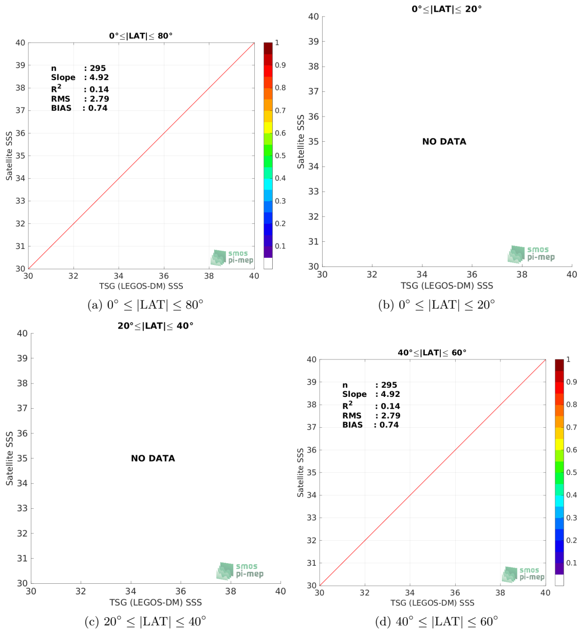
Figure 9: Contour maps of the concentration of SMOS SSS L2Q v331 - With FLAG (CMEMS-CATDS-CPDC) SSS (y-axis) versus TSG (LEGOS-DM) SSS (x-axis) at match-up pairs for different latitude bands. For each plot, the red line shows x=y . The black thin and dashed lines indicate a linear fit through the data cloud and the \pm 95\% confidence levels, respectively. The number match-up pairs n , the slope and R^2 coefficient of the linear fit, the root mean square (RMS) and the mean bias between satellite and in situ data are indicated for each latitude band in each plots.
