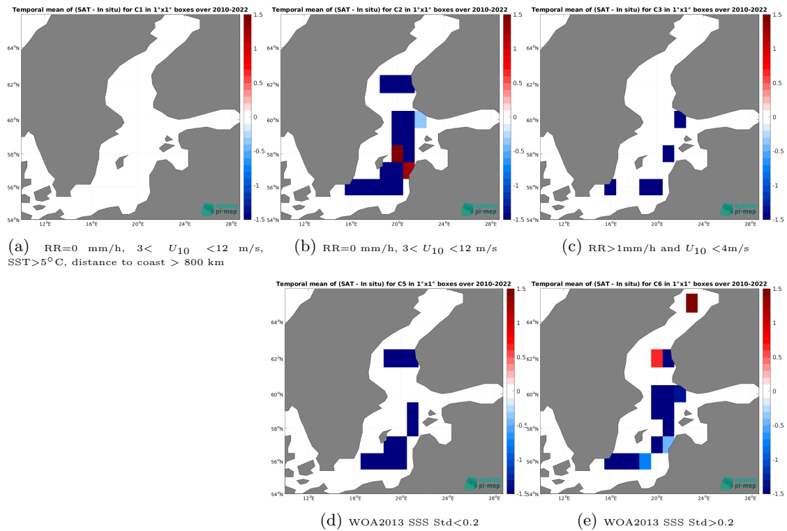
Figure 14: Temporal mean gridded over spatial boxes of size 1^\circ \times 1^\circ of \Delta\text{SSS} (SMOS SSS L2Q v331 - With FLAG (CMEMS-CATDS-CPDC) - ICES) for 5 different subdatasets corresponding to:RR=0 mm/h, 3 < U_{10} < 12 m/s, SST >5^\circ\text{C} , distance to coast > 800 km (a), RR=0 mm/h, 3 < U_{10} < 12 m/s (b), RR >1 mm/h and U_{10} < 4 m/s (c), WOA2013 SSS Std <0.2 (d), WOA2013 SSS Std >0.2 (e).
