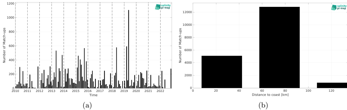
Figure 2: Number of match-ups between ICES and SMOS SSS L2Q v331 - With FLAG (CMEMS-CATDS-CPDC) SSS as a function of time (a) and as function of the distance to coast (b) over the Baltic Sea Pi-MEP region and for the full satellite product period.
