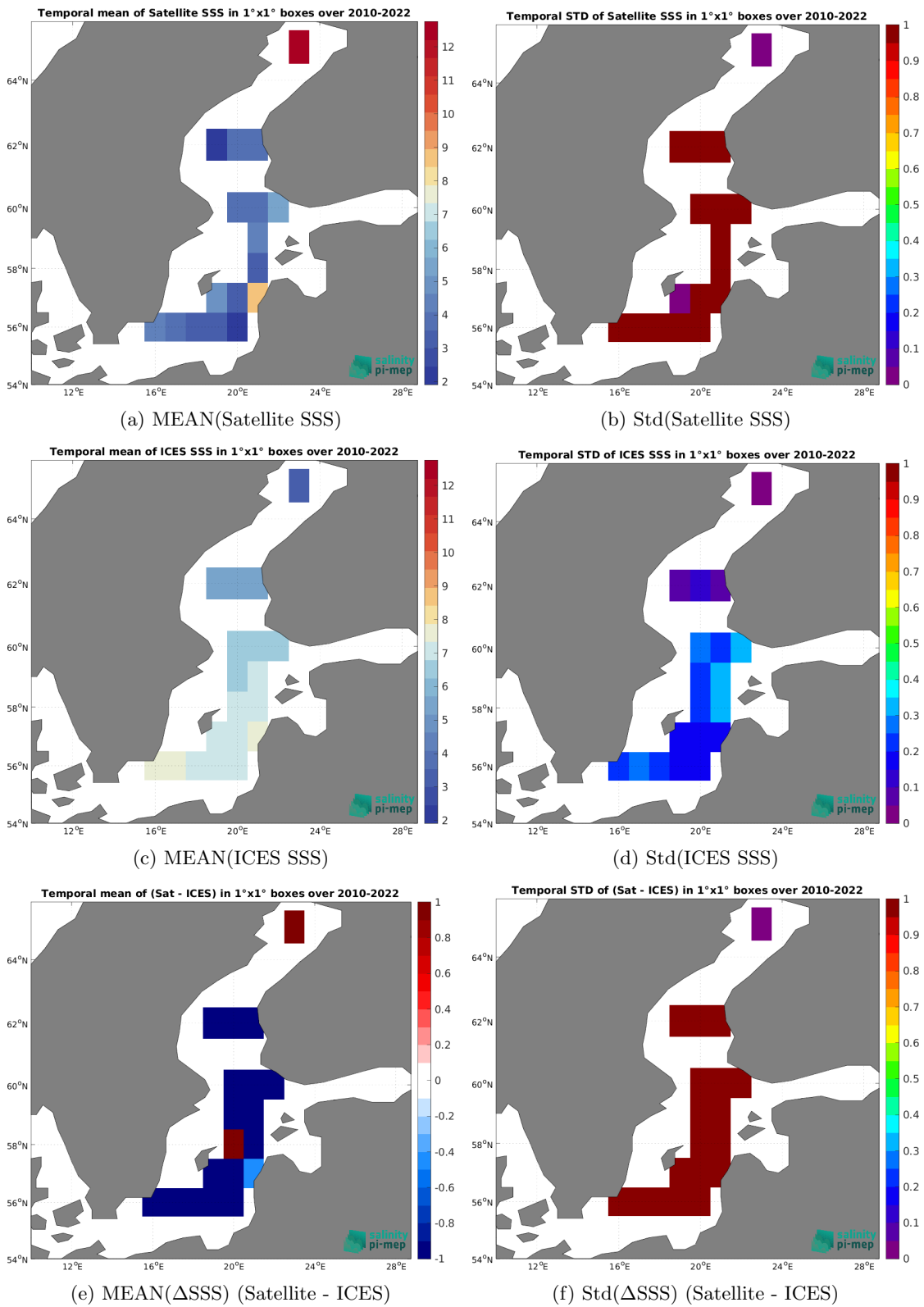
Figure 7: Temporal mean (left) and Std (right) of SSS from SMOS SSS L2Q v331 - With FLAG (CMEMS-CATDS-CPDC) (top), ICES (middle) and of \Delta SSS (Satellite - ICES). Only match-up pairs are used to generate these maps.
