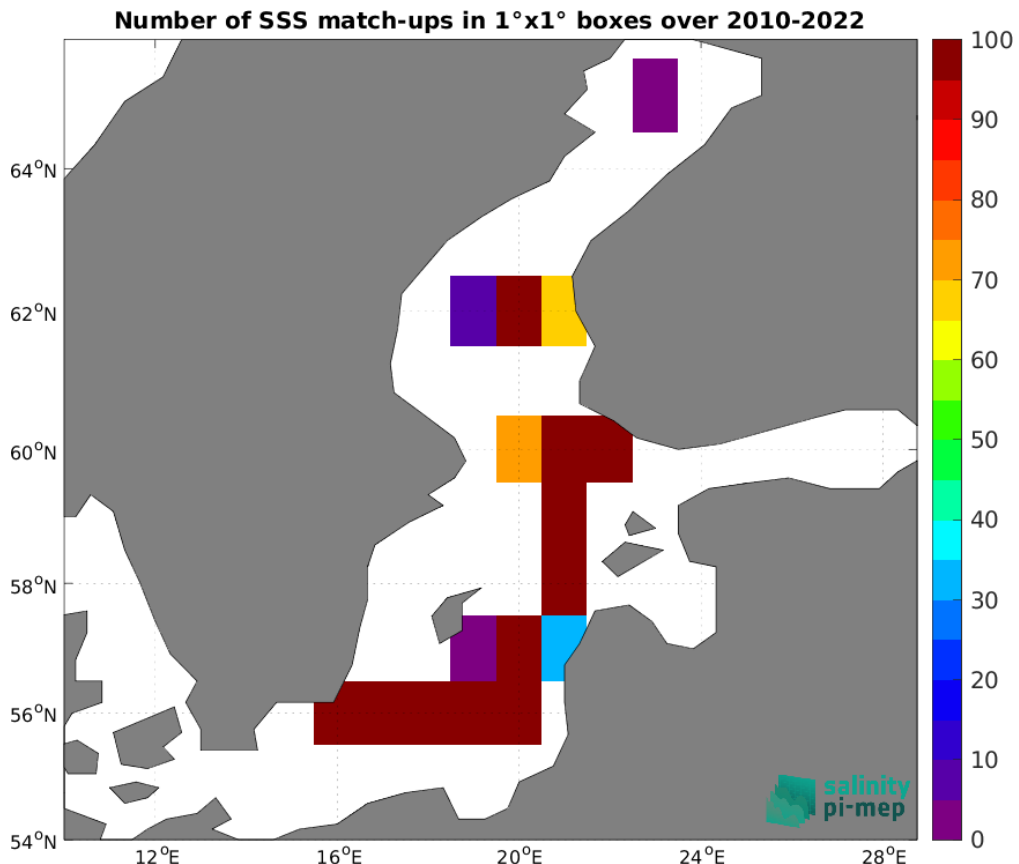
Figure 5: Number of SSS match-ups between ICES SSS and the SMOS SSS L2Q v331 - With FLAG (CMEMS-CATDS-CPDC) SSS product for the Baltic Sea Pi-MEP region over 1°x1° boxes and for the full satellite product period.
