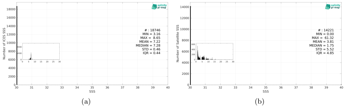
Figure 3: Histograms of SSS from ICES (a) and SMOS SSS L2Q v331 - With FLAG (CMEMS-CATDS-CPDC) (b) considering all match-up pairs per bins of 0.1 over the Baltic Sea Pi-MEP region and for the full satellite product period.
