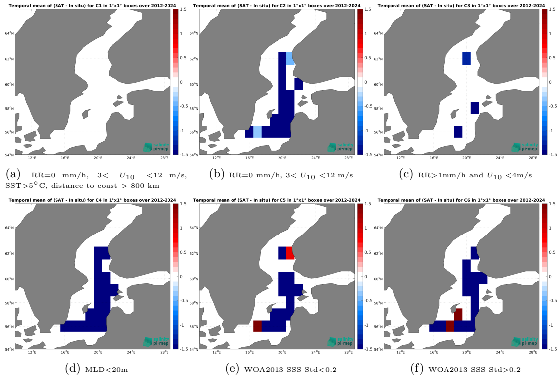
Figure 14: Temporal mean gridded over spatial boxes of size 1^\circ \times 1^\circ of \Delta SSS (SMOS SSS L2Q v331 - With FLAG (CMEMS-CATDS-CPDC) - Argo) for 6 different subdatasets corresponding to:RR=0 mm/h, 3 < U_{10} < 12 m/s, SST>5°C, distance to coast > 800 km (a), RR=0 mm/h, 3 < U_{10} < 12 m/s (b), RR>1mm/h and U_{10} < 4 m/s (c),MLD<20m (d),WOA2013 SSS Std<0.2 (e),WOA2013 SSS Std>0.2 (f).
