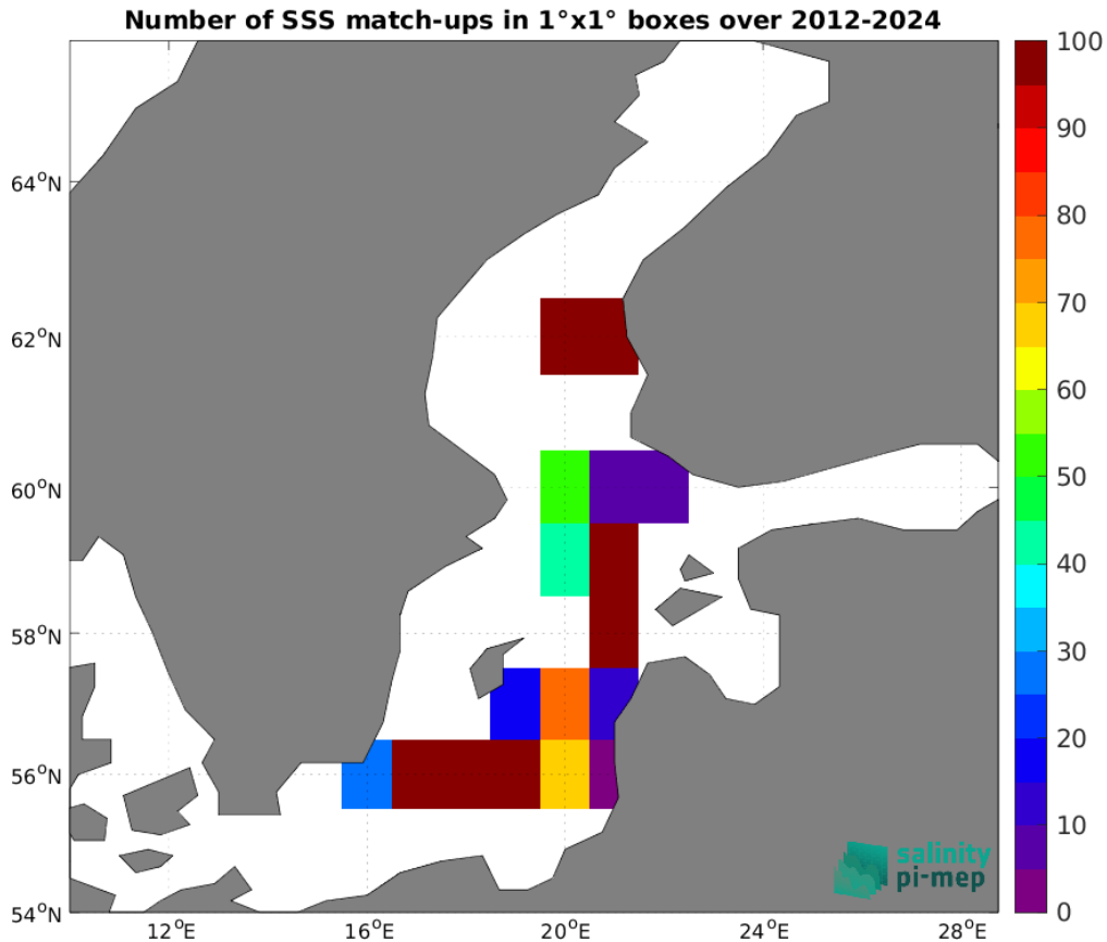
Figure 5: Number of SSS match-ups between Argo SSS and the SMOS SSS L2Q v331 - With FLAG (CMEMS-CATDS-CPDC) SSS product for the Baltic Sea Pi-MEP region over 1^\circ \times 1^\circ boxes and for the full satellite product period.
