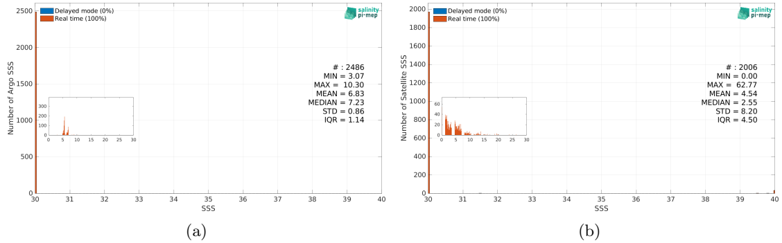
Figure 3: Histograms of SSS from Argo (a) and SMOS SSS L2Q v331 - With FLAG (CMEMS-CATDS-CPDC) (b) considering all match-up pairs per bins of 0.1 over the Baltic Sea Pi-MEP region and for the full satellite product period.
