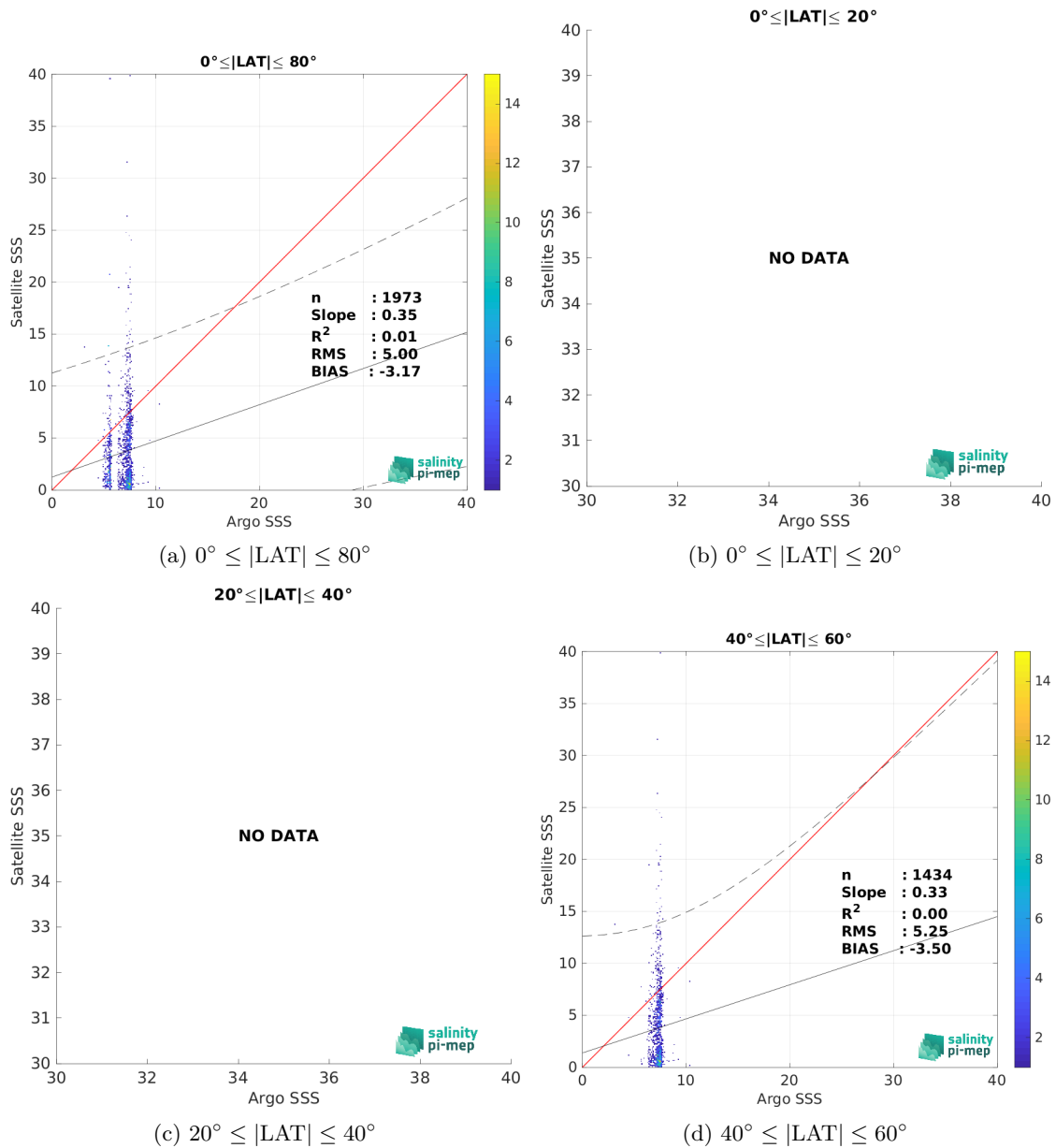
Figure 10: Contour maps of the concentration of SMOS SSS L2Q v331 - With FLAG (CMEMS-CATDS-CPDC) SSS (y-axis) versus Argo SSS (x-axis) at match-up pairs for different latitude bands. For each plot, the red line shows x=y . The black thin and dashed lines indicate a linear fit through the data cloud and the \pm 95\% confidence levels, respectively. The number match-up pairs n , the slope and R^2 coefficient of the linear fit, the root mean square (RMS) and the mean bias between satellite and in situ data are indicated for each latitude band in each plots.
