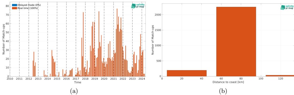
Figure 2: Number of match-ups between Argo and SMOS SSS L2Q v331 - With FLAG (CMEMS-CATDS-CPDC) SSS as a function of time (a) and as function of the distance to coast (b) over the Baltic Sea Pi-MEP region and for the full satellite product period.
