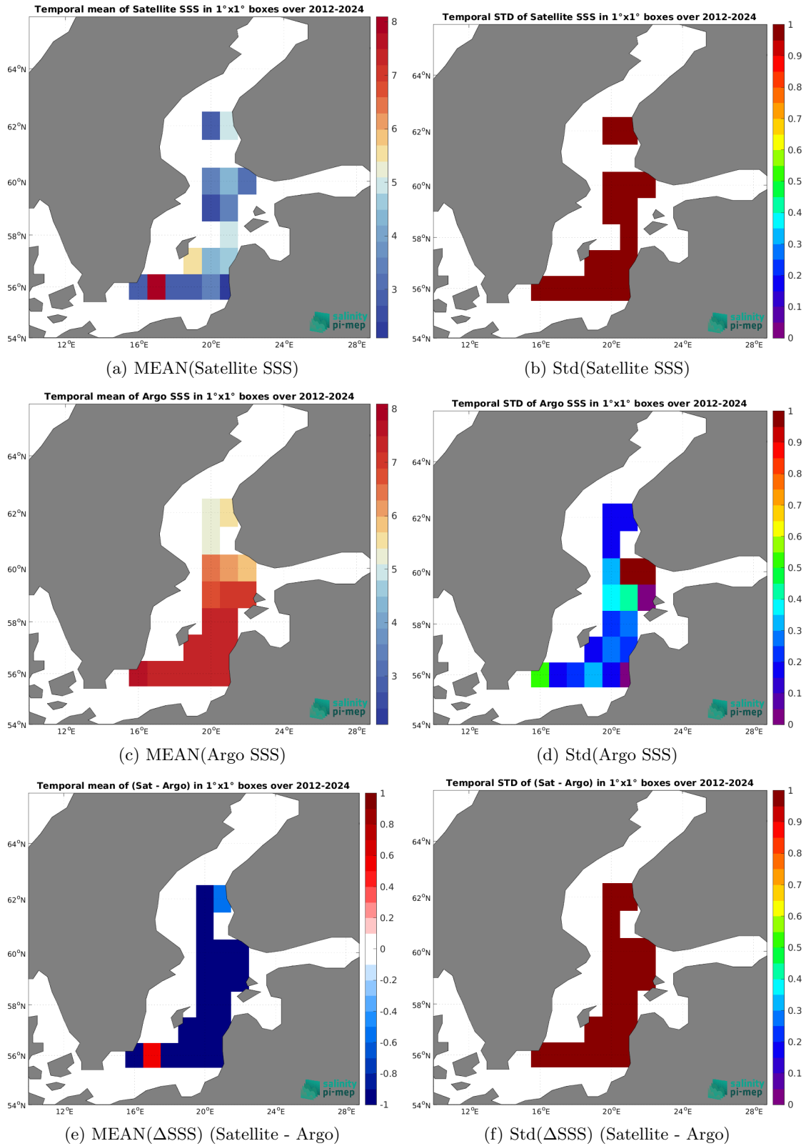
Figure 7: Temporal mean (left) and Std (right) of SSS from SMOS SSS L2Q v331 - With FLAG (CMEMS-CATDS-CPDC) (top), Argo (middle), and of \Delta SSS (Satellite - Argo). Only match-up pairs are used to generate these maps.
