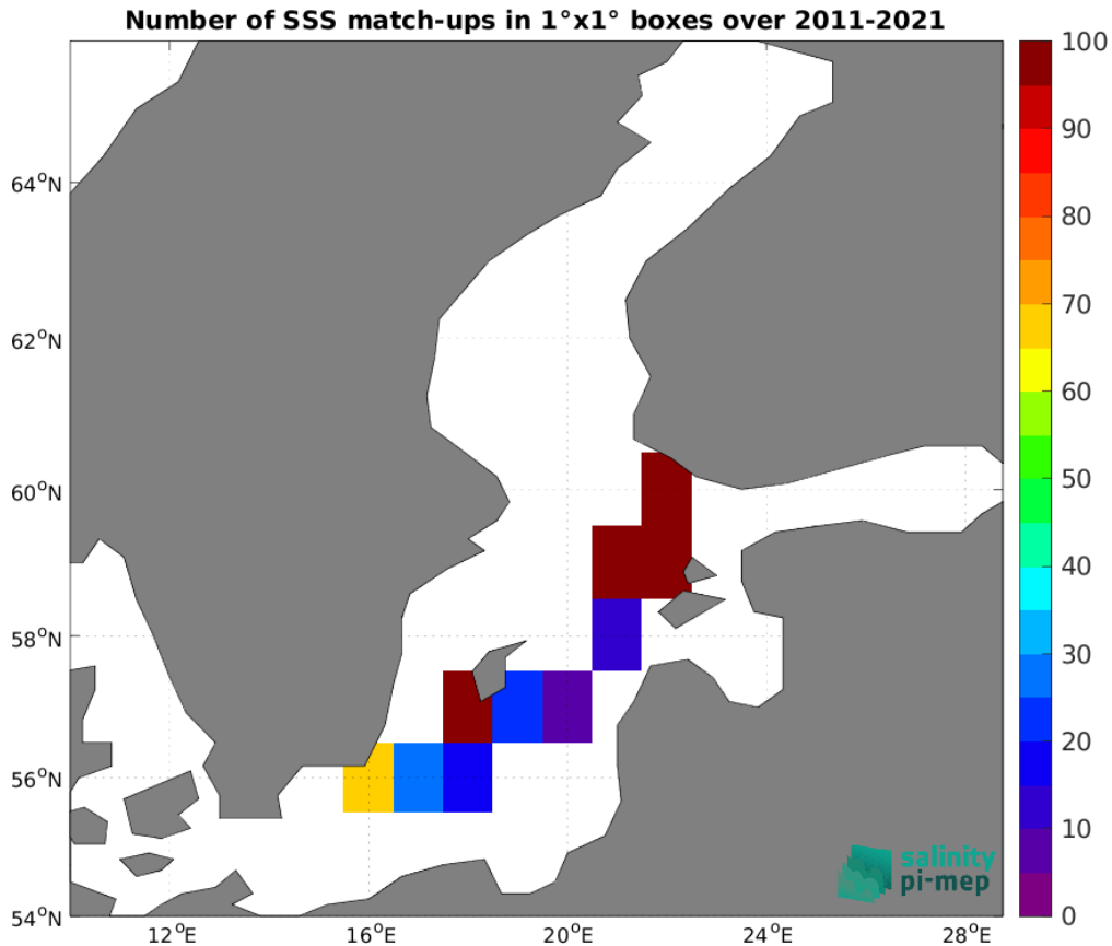
Figure 5: Number of SSS match-ups between TSG (LEGOS-DM) SSS and the SMOS SSS L2Q v331 - No FLAG (CMEMS-CATDS-CPDC) SSS product for the Baltic Sea Pi-MEP region over 1^\circ \times 1^\circ boxes and for the full satellite product period.
