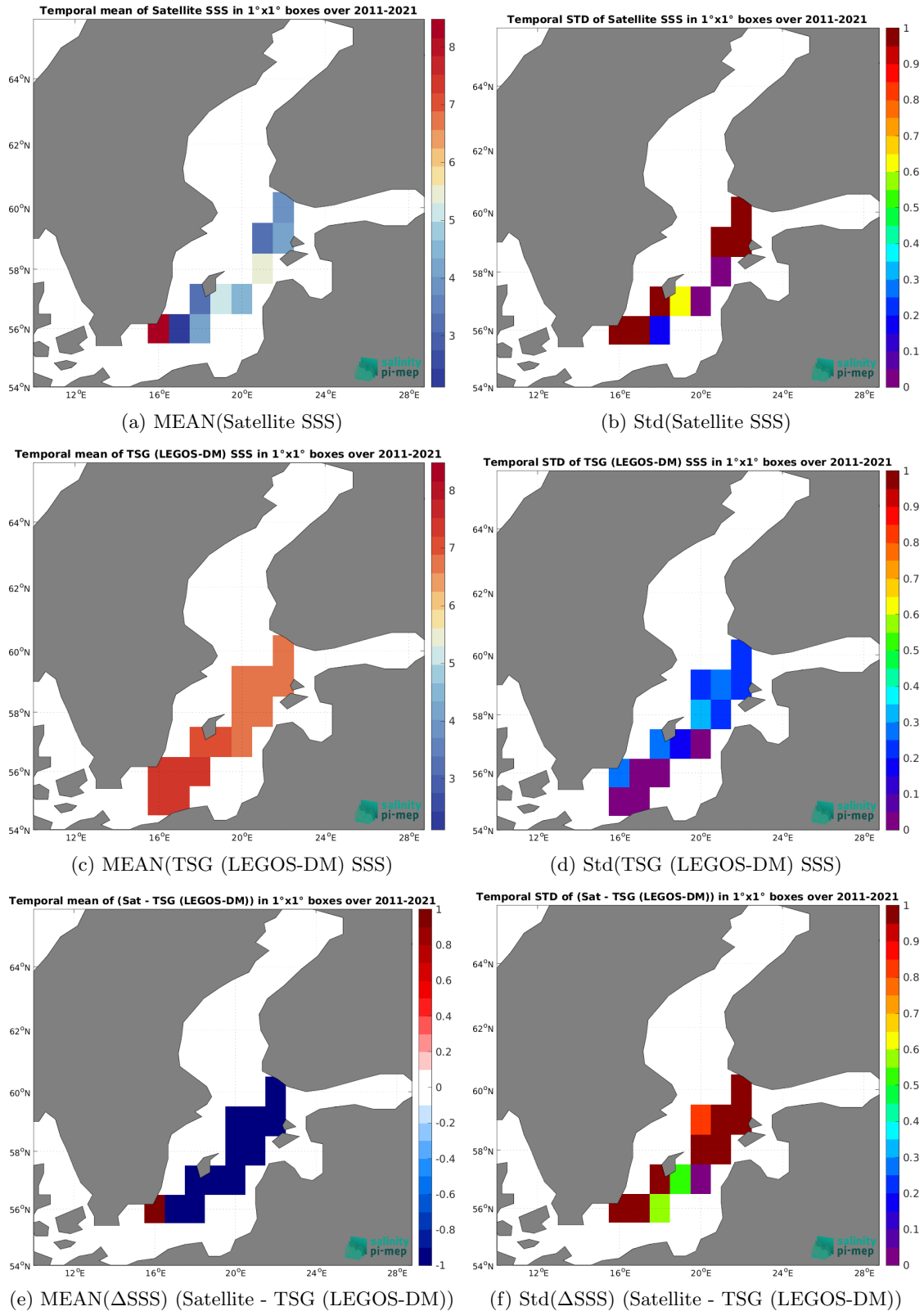
Figure 7: Temporal mean (left) and Std (right) of SSS from SMOS SSS L2Q v331 - No FLAG (CMEMS-CATDS-CPDC) (top), TSG (LEGOS-DM) (middle), and of \Delta SSS (Satellite - TSG (LEGOS-DM)). Only match-up pairs are used to generate these maps.
