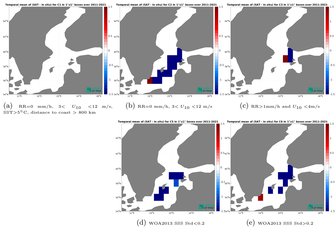
Figure 14: Temporal mean gridded over spatial boxes of size 1^\circ \times 1^\circ of \Delta\text{SSS} (SMOS SSS L2Q v331 - No FLAG (CMEMS-CATDS-CPDC) - TSG (LEGOS-DM)) for 5 different subdatasets corresponding to:RR=0 mm/h, 3 < U_{10} < 12 m/s, SST>5°C, distance to coast > 800 km (a), RR=0 mm/h, 3 < U_{10} < 12 m/s (b), RR>1mm/h and U_{10} < 4 m/s (c), WOA2013 SSS Std<0.2 (d), WOA2013 SSS Std>0.2 (e).
