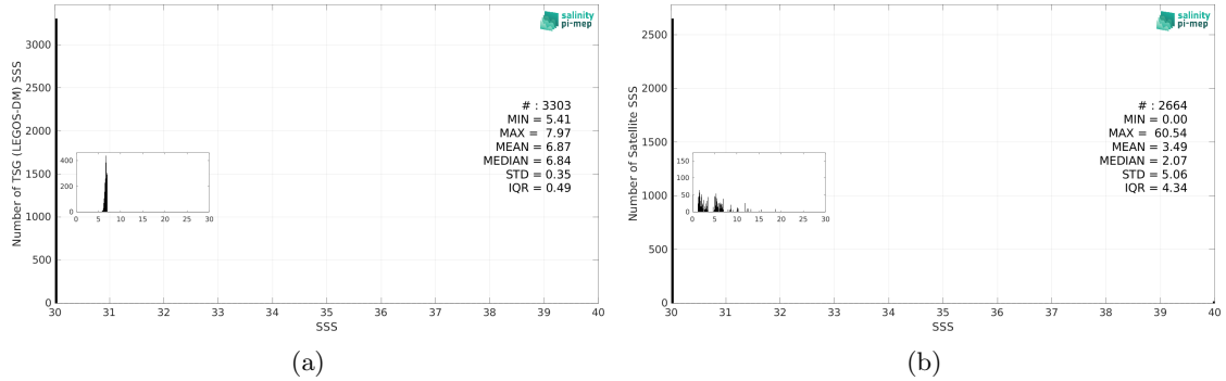
Figure 3: Histograms of SSS from TSG (LEGOS-DM) (a) and SMOS SSS L2Q v331 - No FLAG (CMEMS-CATDS-CPDC) (b) considering all match-up pairs per bins of 0.1 over the Baltic Sea Pi-MEP region and for the full satellite product period.
