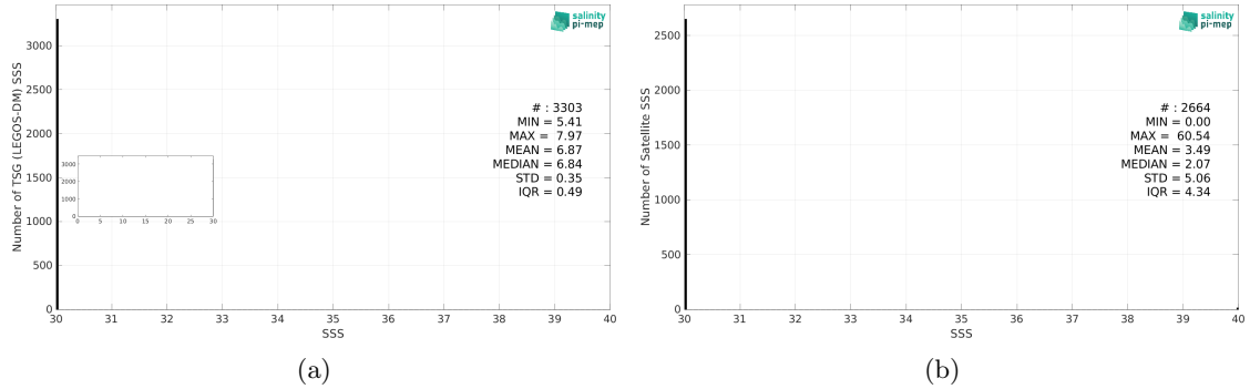
Figure 2: Histograms of SSS from TSG (LEGOS-DM) (a) and SMOS SSS L2Q v331 - No FLAG (CMEMS-CATDS-CPDC) (b) considering all match-up pairs per bins of 0.1 over the Baltic Sea Pi-MEP region and for the full satellite product period.
