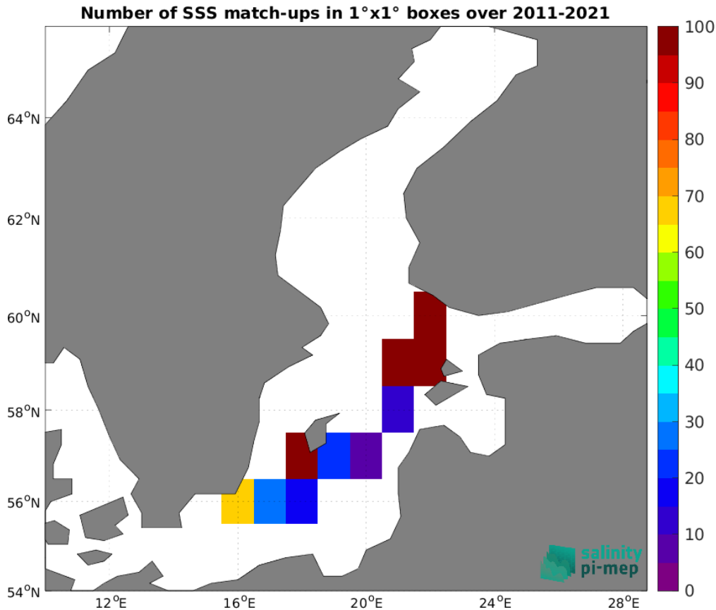
Figure 4: Number of SSS match-ups between TSG (LEGOS-DM) SSS and the SMOS SSS L2Q v331 - No FLAG (CMEMS-CATDS-CPDC) SSS product for the Baltic Sea Pi-MEP region over 1^\circ \times 1^\circ boxes and for the full satellite product period.
