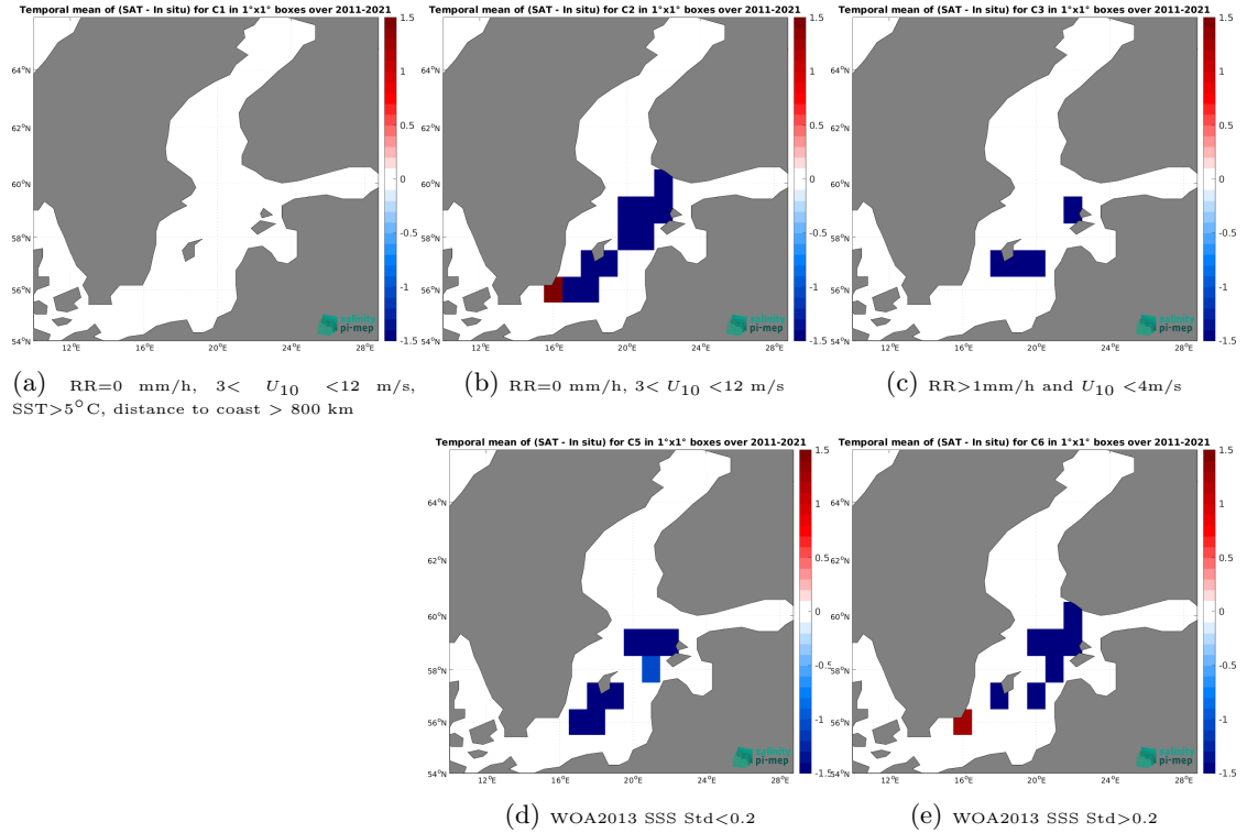
Figure 12: Temporal mean gridded over spatial boxes of size 1^{\circ}\times 1^{\circ} of \Delta\text{SSS} (SMOS SSS L2Q v331 - No FLAG (CMEMS-CATDS-CPDC) - TSG (LEGOS-DM)) for 5 different subdatasets corresponding to:RR=0 mm/h, 3 < U_{10} < 12 m/s, SST > 5^{\circ}\text{C} , distance to coast > 800 km (a), RR=0 mm/h, 3 < U_{10} < 12 m/s (b), RR > 1 mm/h and U_{10} < 4 m/s (c), WOA2013 SSS Std < 0.2 (d), WOA2013 SSS Std > 0.2 (e).
