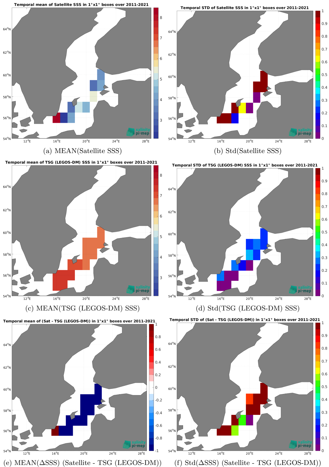
Figure 6: Temporal mean (left) and Std (right) of SSS from SMOS SSS L2Q v331 - No FLAG (CMEMS-CATDS-CPDC) (top), TSG (LEGOS-DM) (middle), and of \Delta SSS (Satellite - TSG (LEGOS-DM)). Only match-up pairs are used to generate these maps.
