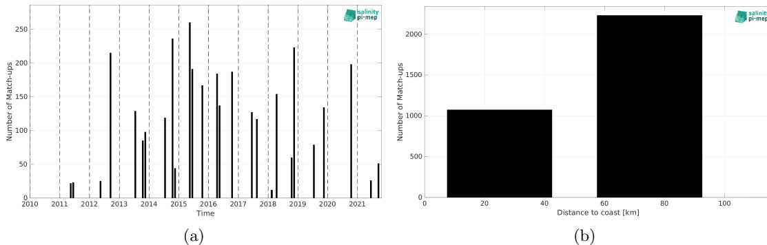
Figure 1: Number of match-ups between TSG (LEGOS-DM) and SMOS SSS L2Q v331 - No FLAG (CMEMS-CATDS-CPDC) SSS as a function of time (a) and as function of the distance to coast (b) over the Baltic Sea Pi-MEP region and for the full satellite product period.
