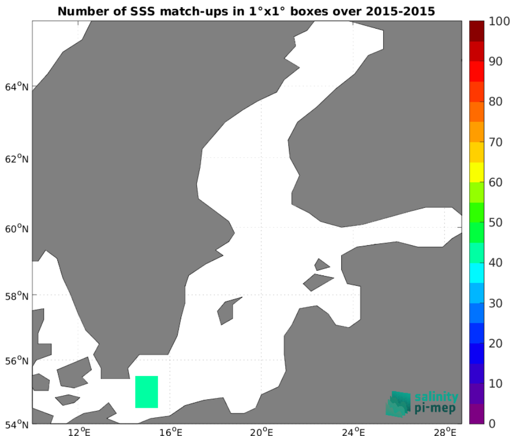
Figure 5: Number of SSS match-ups between TSG (GOSUD-Research-vessel) SSS and the SMOS SSS L2Q v331 - No FLAG (CMEMS-CATDS-CPDC) SSS product for the Baltic Sea Pi-MEP region over 1°x1° boxes and for the full satellite product period.
