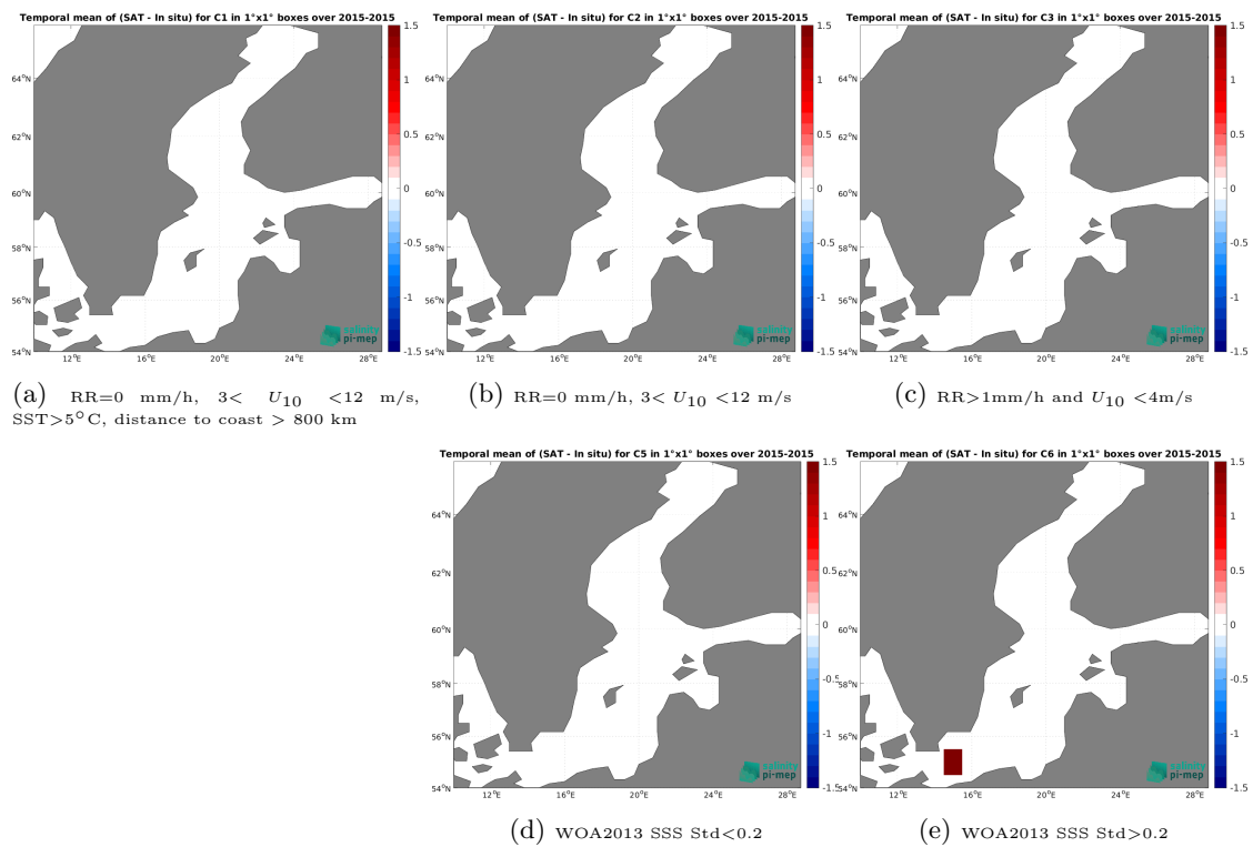
Figure 14: Temporal mean gridded over spatial boxes of size 1^\circ \times 1^\circ of \Delta SSS (SMOS SSS L2Q v331 - No FLAG (CMEMS-CATDS-CPDC) - TSG (GOSUD-Research-vessel)) for 5 different subdatasets corresponding to:RR=0 mm/h, 3 < U_{10} < 12 m/s, SST >5^\circ\text{C} , distance to coast > 800 km (a), RR=0 mm/h, 3 < U_{10} < 12 m/s (b), RR >1 mm/h and U_{10} < 4 m/s (c), WOA2013 SSS Std <0.2 (d), WOA2013 SSS Std >0.2 (e).
