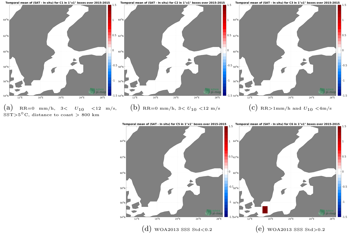
Figure 12: Temporal mean gridded over spatial boxes of size 1^\circ \times 1^\circ of \Delta SSS (SMOS SSS L2Q v331 - No FLAG (CMEMS-CATDS-CPDC) - TSG (GOSUD-Research-vessel)) for 5 different subdatasets corresponding to: RR=0 mm/h, 3 < U_{10} < 12 m/s, SST > 5^\circ\text{C} , distance to coast > 800 km (a), RR=0 mm/h, 3 < U_{10} < 12 m/s (b), RR > 1 mm/h and U_{10} < 4 m/s (c), WOA2013 SSS Std < 0.2 (d), WOA2013 SSS Std > 0.2 (e).
