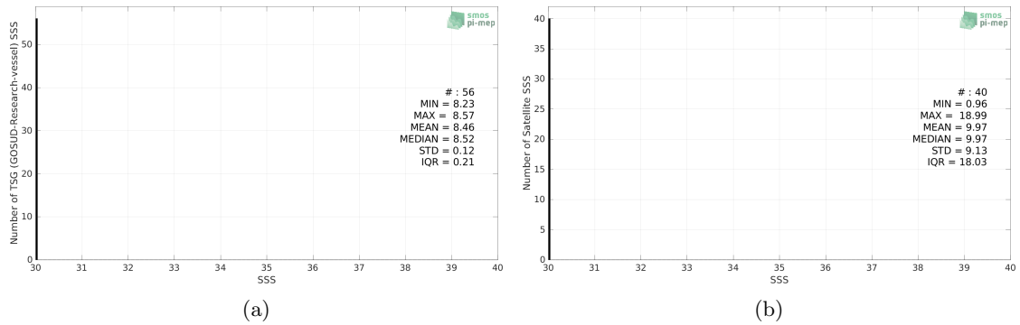
Figure 2: Histograms of SSS from TSG (GOSUD-Research-vessel) (a) and SMOS SSS L2Q v331 - No FLAG (CMEMS-CATDS-CPDC) (b) considering all match-up pairs per bins of 0.1 over the Baltic Sea Pi-MEP region and for the full satellite product period.
