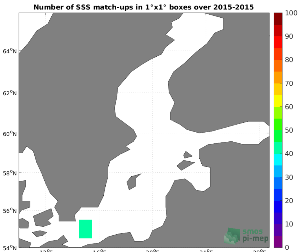
Figure 4: Number of SSS match-ups between TSG (GOSUD-Research-vessel) SSS and the SMOS SSS L2Q v331 - No FLAG (CMEMS-CATDS-CPDC) SSS product for the Baltic Sea Pi-MEP region over 1°x1° boxes and for the full satellite product period.
