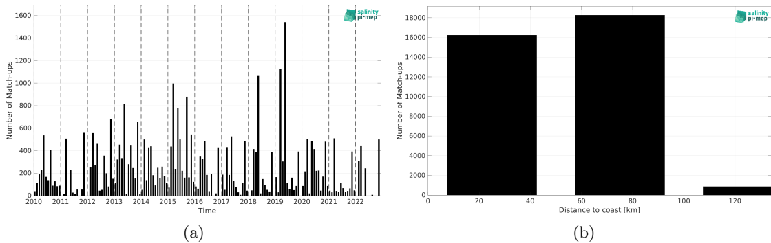
Figure 2: Number of match-ups between ICES and SMOS SSS L2Q v331 - No FLAG (CMEMS-CATDS-CPDC) SSS as a function of time (a) and as function of the distance to coast (b) over the Baltic Sea Pi-MEP region and for the full satellite product period.
