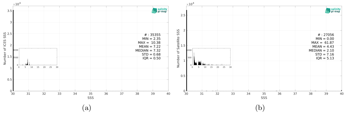
Figure 3: Histograms of SSS from ICES (a) and SMOS SSS L2Q v331 - No FLAG (CMEMS-CATDS-CPDC) (b) considering all match-up pairs per bins of 0.1 over the Baltic Sea Pi-MEP region and for the full satellite product period.
