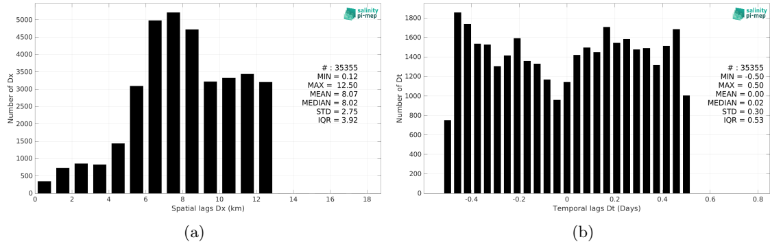
Figure 6: Histograms of the spatial (a) and temporal (b) lags between the location/time of the ICES measurement and the date of the corresponding SMOS SSS L2Q v331 - No FLAG (CMEMS-CATDS-CPDC) SSS pixel.
