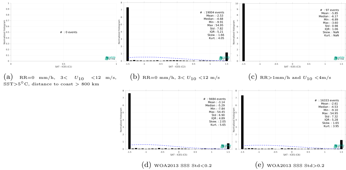
Figure 15: Normalized histogram of \Delta SSS (SMOS SSS L2Q v331 - No FLAG (CMEMS-CATDS-CPDC) - ICES) for 5 different subdatasets corresponding to: RR=0 mm/h, 3 < U_{10} < 12 m/s, SST > 5°C, distance to coast > 800 km (a), RR=0 mm/h, 3 < U_{10} < 12 m/s (b), RR > 1mm/h and U_{10} < 4 m/s (c), WOA2013 SSS Std < 0.2 (d), WOA2013 SSS Std > 0.2 (e).
