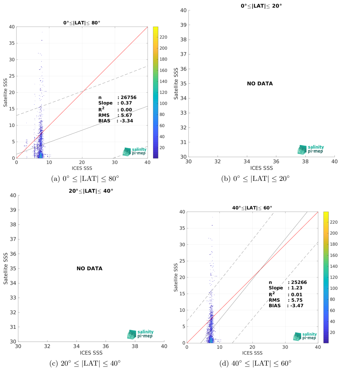
Figure 10: Contour maps of the concentration of SMOS SSS L2Q v331 - No FLAG (CMEMS-CATDS-CPDC) SSS (y-axis) versus ICES SSS (x-axis) at match-up pairs for different latitude bands. For each plot, the red line shows x=y . The black thin and dashed lines indicate a linear fit through the data cloud and the \pm 95\% confidence levels, respectively. The number match-up pairs n , the slope and R^2 coefficient of the linear fit, the root mean square (RMS) and the mean bias between satellite and in situ data are indicated for each latitude band in each plots.
