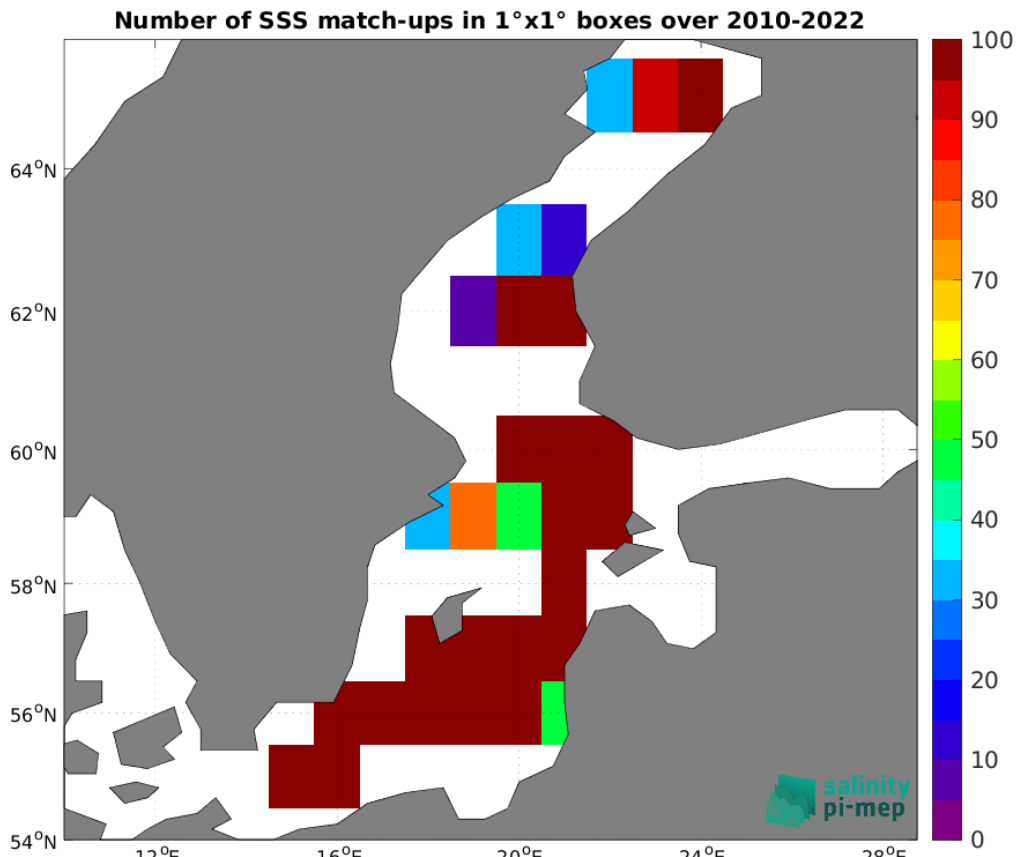
Figure 5: Number of SSS match-ups between ICES SSS and the SMOS SSS L2Q v331 - No FLAG (CMEMS-CATDS-CPDC) SSS product for the Baltic Sea Pi-MEP region over 1°x1° boxes and for the full satellite product period.
