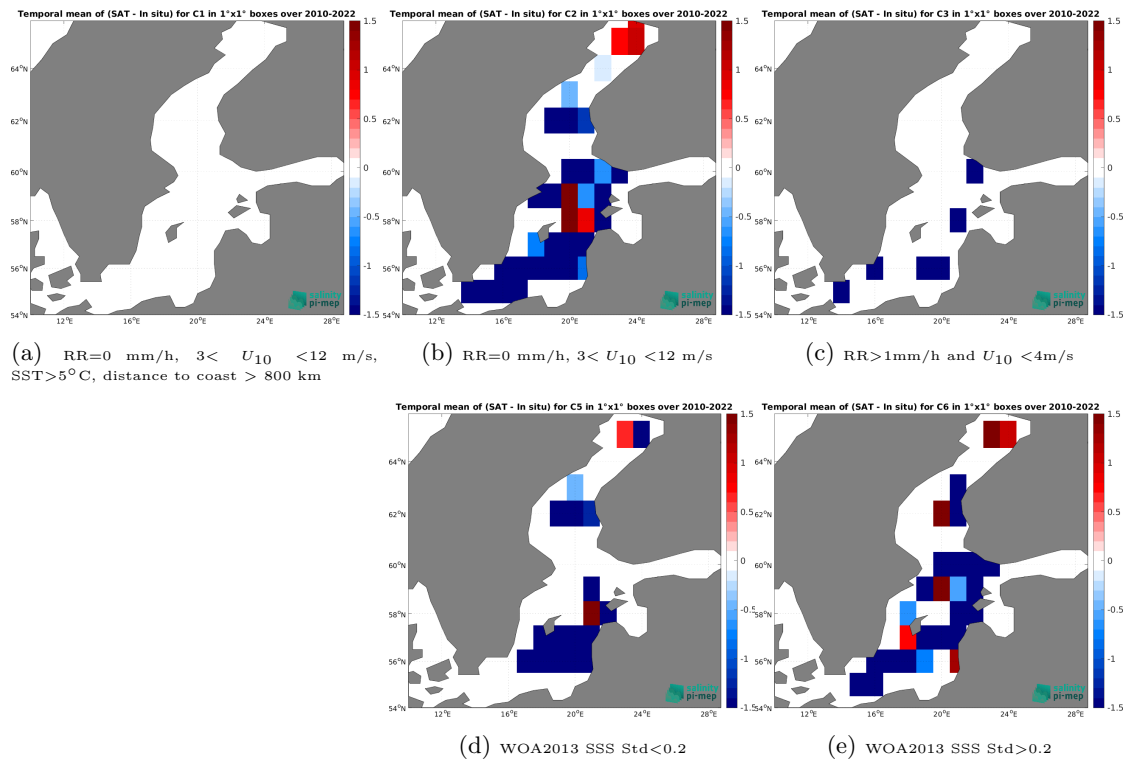
Figure 14: Temporal mean gridded over spatial boxes of size 1^\circ \times 1^\circ of \Delta SSS (SMOS SSS L2Q v331 - No FLAG (CMEMS-CATDS-CPDC) - ICES) for 5 different subdatasets corresponding to:RR=0 mm/h, 3 < U_{10} < 12 m/s, SST >5^\circ C, distance to coast > 800 km (a), RR=0 mm/h, 3 < U_{10} < 12 m/s (b), RR >1 mm/h and U_{10} < 4 m/s (c), WOA2013 SSS Std <0.2 (d), WOA2013 SSS Std >0.2 (e).
