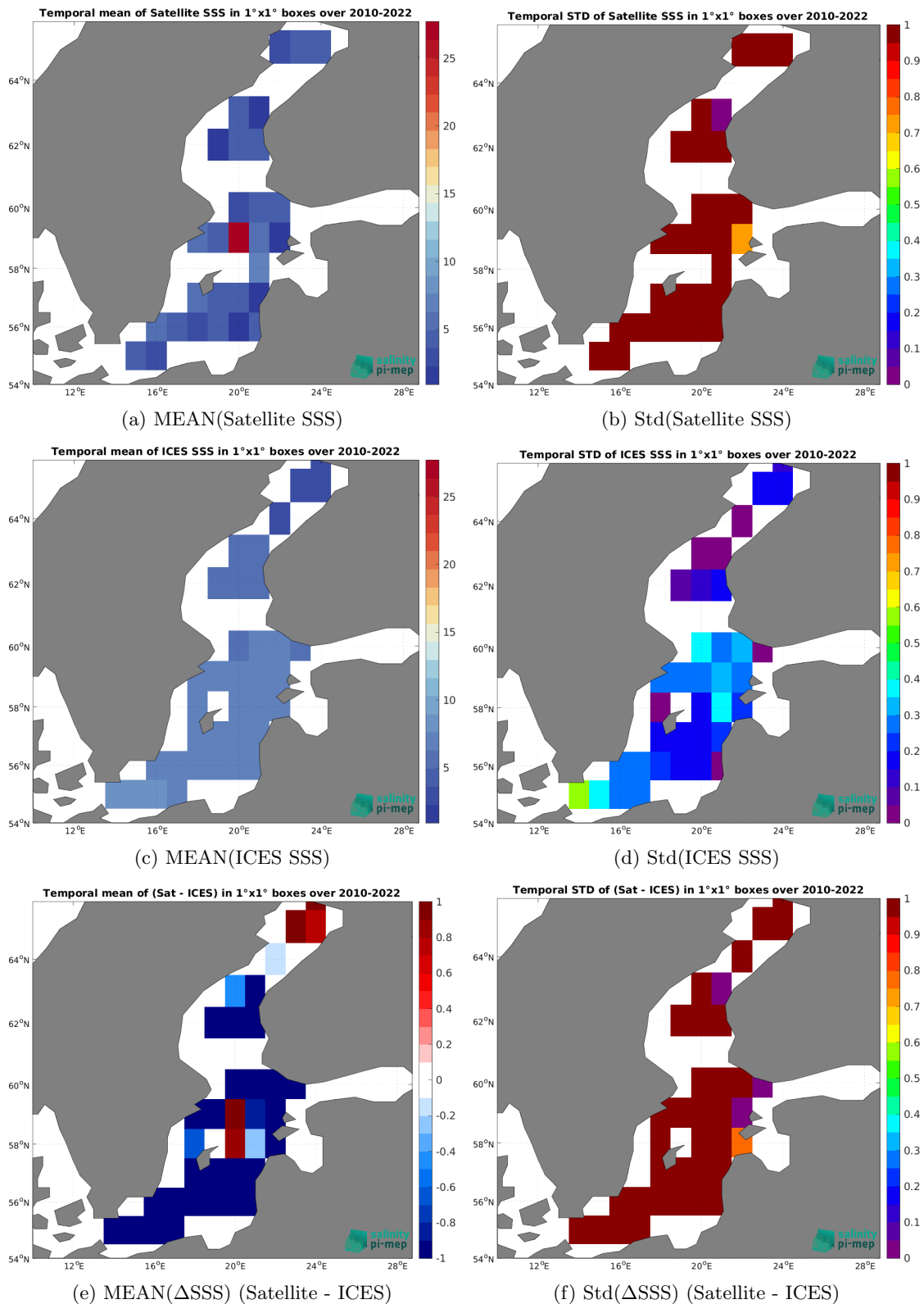
Figure 7: Temporal mean (left) and Std (right) of SSS from SMOS SSS L2Q v331 - No FLAG (CMEMS-CATDS-CPDC) (top), ICES (middle) and of \Delta SSS (Satellite - ICES). Only match-up pairs are used to generate these maps.
