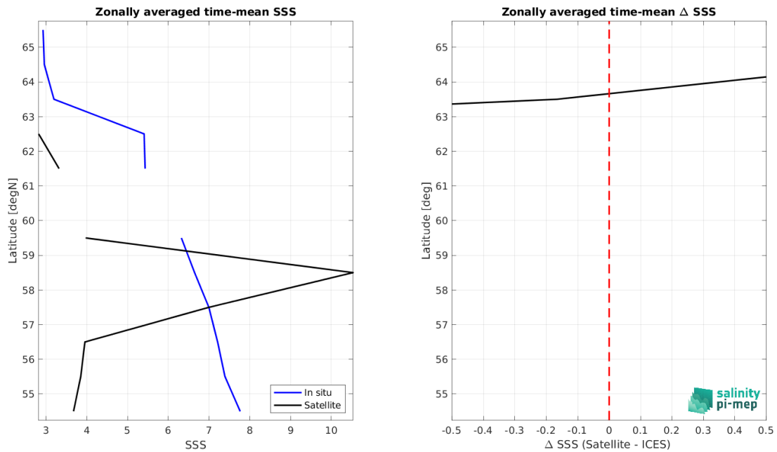
Figure 9: Left panel: Zonal mean SSS from SMOS SSS L2Q v331 - No FLAG (CMEMS-CATDS-CPDC) satellite product (black) and from ICES (blue). Right panel: Zonal mean of \Delta SSS (Satellite - ICES) for all the collected Pi-MEP match-up pairs estimated over the full satellite product period.
