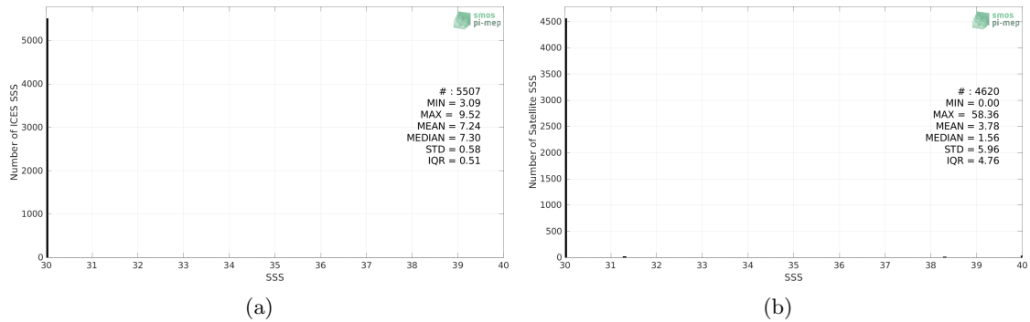
Figure 2: Histograms of SSS from ICES (a) and SMOS SSS L2Q v331 - No FLAG (CMEMS-CATDS-CPDC) (b) considering all match-up pairs per bins of 0.1 over the Baltic Sea Pi-MEP region and for the full satellite product period.
