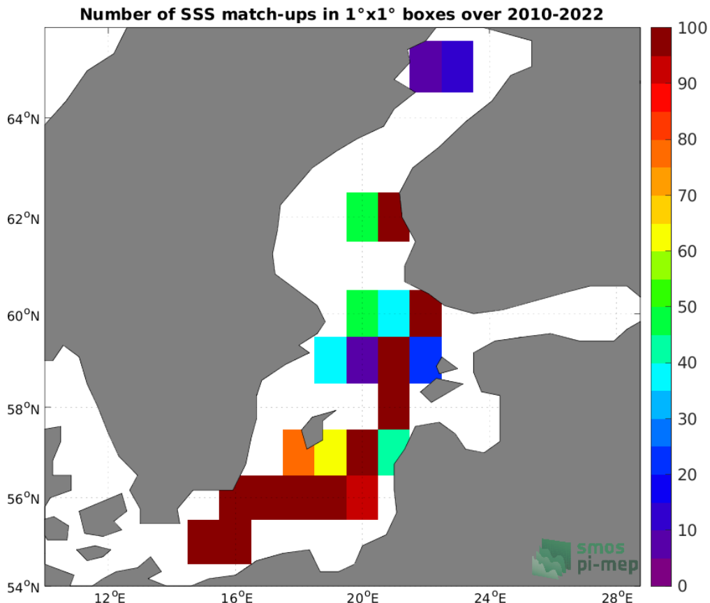
Figure 4: Number of SSS match-ups between ICES SSS and the SMOS SSS L2Q v331 - No FLAG (CMEMS-CATDS-CPDC) SSS product for the Baltic Sea Pi-MEP region over 1°×1° boxes and for the full satellite product period.
