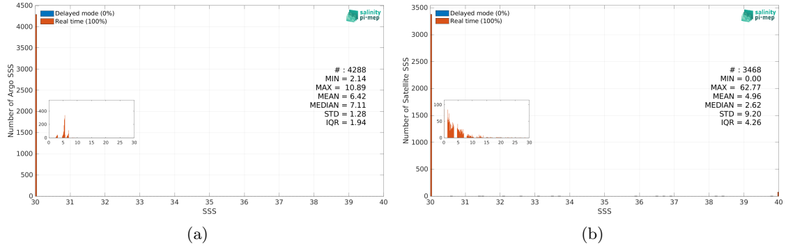
Figure 3: Histograms of SSS from Argo (a) and SMOS SSS L2Q v331 - No FLAG (CMEMS-CATDS-CPDC) (b) considering all match-up pairs per bins of 0.1 over the Baltic Sea Pi-MEP region and for the full satellite product period.
