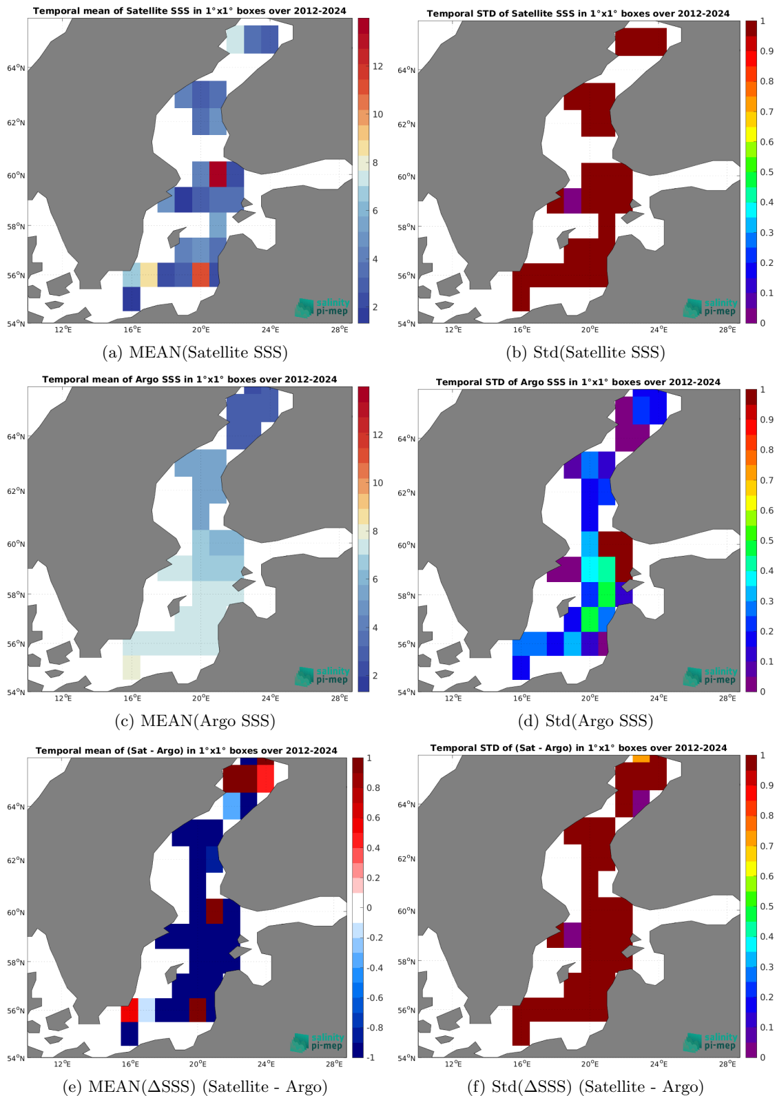
Figure 7: Temporal mean (left) and Std (right) of SSS from SMOS SSS L2Q v331 - No FLAG (CMEMS-CATDS-CPDC) (top), Argo (middle) and of \Delta SSS (Satellite - Argo). Only match-up pairs are used to generate these maps.
