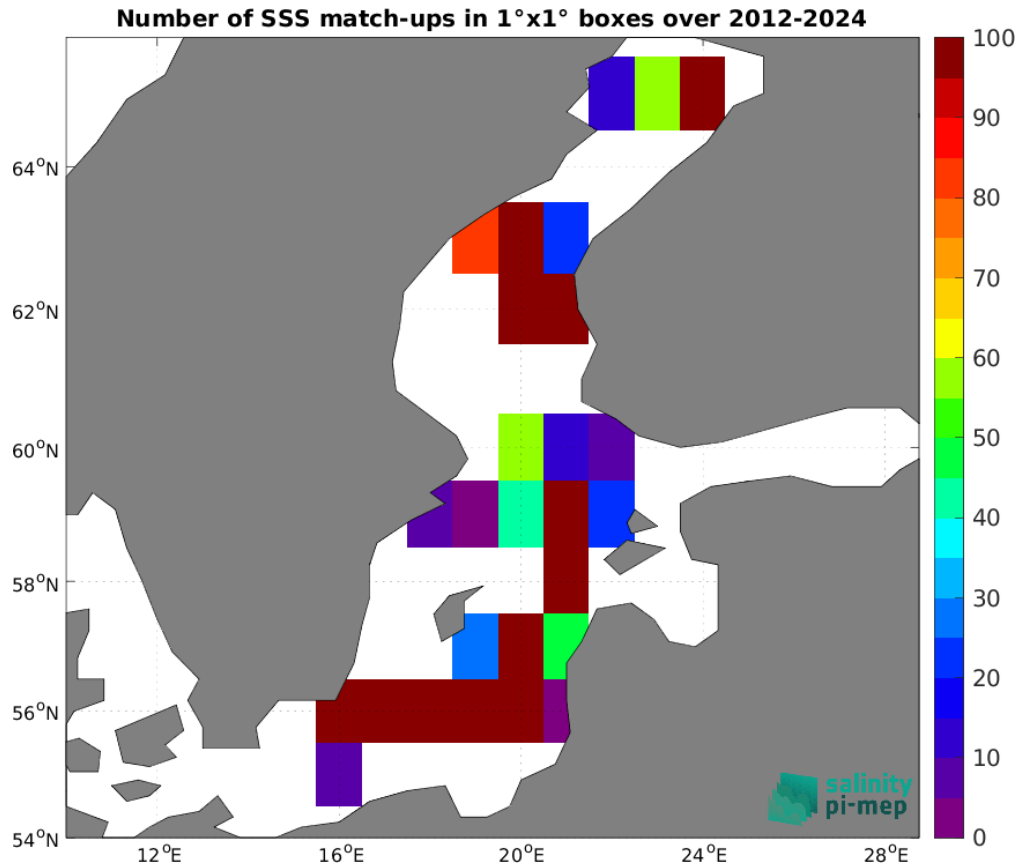
Figure 5: Number of SSS match-ups between Argo SSS and the SMOS SSS L2Q v331 - No FLAG (CMEMS-CATDS-CPDC) SSS product for the Baltic Sea Pi-MEP region over 1^{\circ} \times 1^{\circ} boxes and for the full satellite product period.
