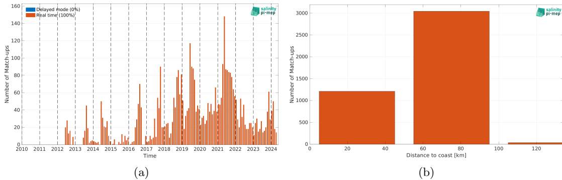
Figure 2: Number of match-ups between Argo and SMOS SSS L2Q v331 - No FLAG (CMEMS-CATDS-CPDC) SSS as a function of time (a) and as function of the distance to coast (b) over the Baltic Sea Pi-MEP region and for the full satellite product period.
