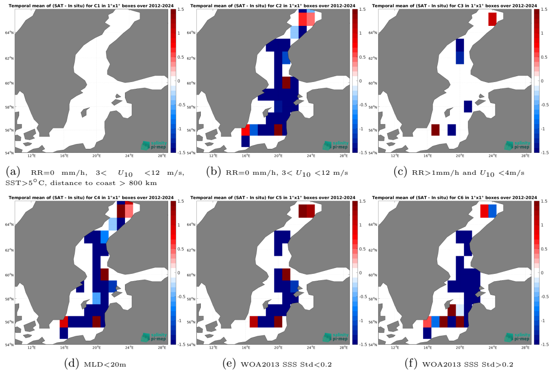
Figure 14: Temporal mean gridded over spatial boxes of size 1^\circ \times 1^\circ of \Delta\text{SSS} (SMOS SSS L2Q v331 - No FLAG (CMEMS-CATDS-CPDC) - Argo) for 6 different subdatasets corresponding to:RR=0 mm/h, 3 < U_{10} < 12 m/s, SST>5°C, distance to coast > 800 km (a), RR=0 mm/h, 3 < U_{10} < 12 m/s (b), RR>1mm/h and U_{10} < 4 m/s (c),MLD<20m (d),WOA2013 SSS Std<0.2 (e),WOA2013 SSS Std>0.2 (f).
