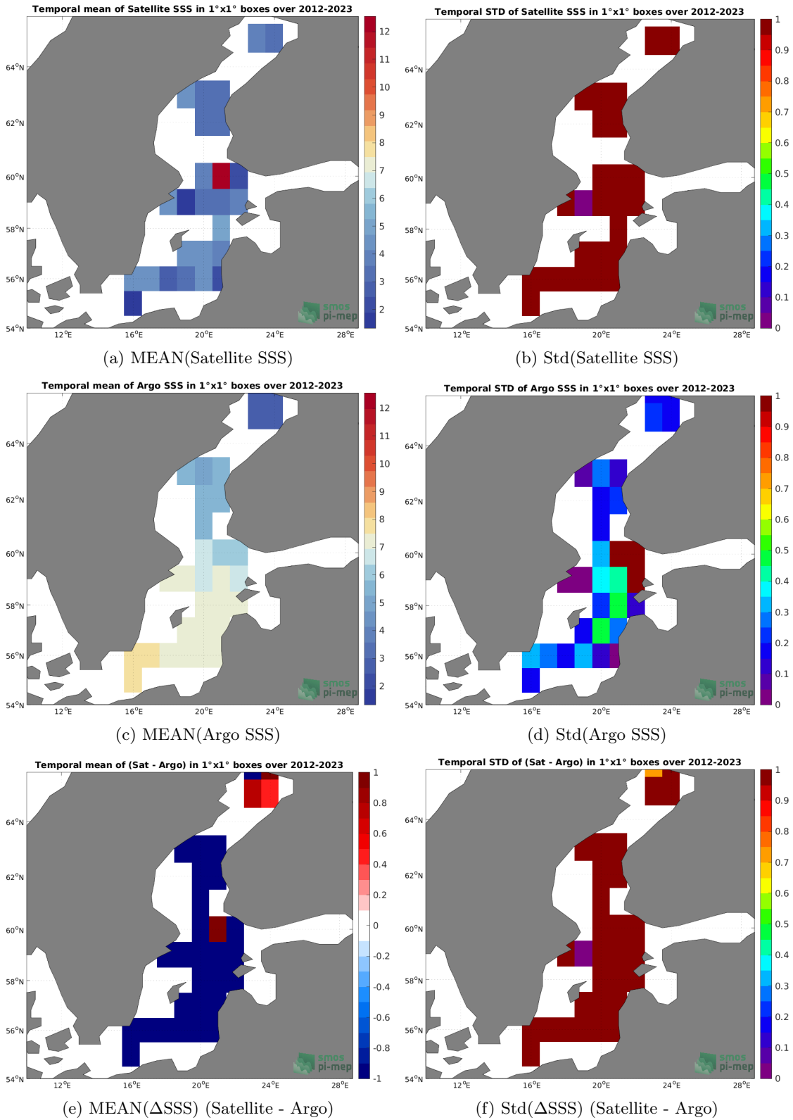
Figure 6: Temporal mean (left) and Std (right) of SSS from SMOS SSS L2Q v331 - No FLAG (CMEMS-CATDS-CPDC) (top), Argo (middle), and of \Delta SSS (Satellite - Argo). Only match-up pairs are used to generate these maps.
