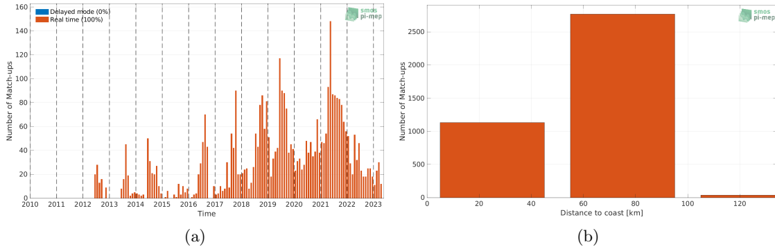
Figure 1: Number of match-ups between Argo and SMOS SSS L2Q v331 - No FLAG (CMEMS-CATDS-CPDC) SSS as a function of time (a) and as function of the distance to coast (b) over the Baltic Sea Pi-MEP region and for the full satellite product period.
