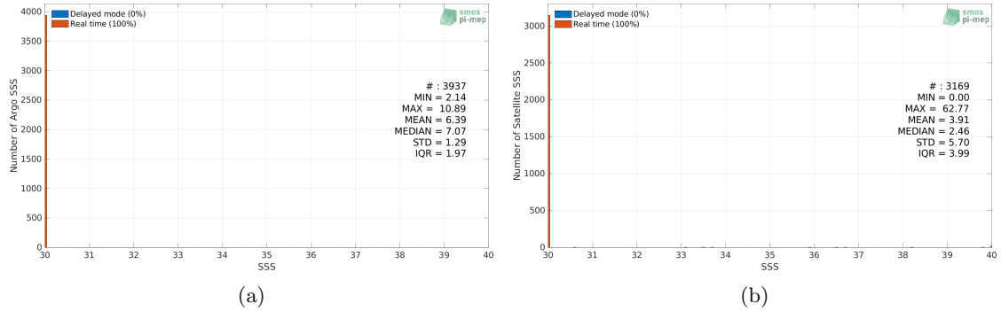
Figure 2: Histograms of SSS from Argo (a) and SMOS SSS L2Q v331 - No FLAG (CMEMS-CATDS-CPDC) (b) considering all match-up pairs per bins of 0.1 over the Baltic Sea Pi-MEP region and for the full satellite product period.
