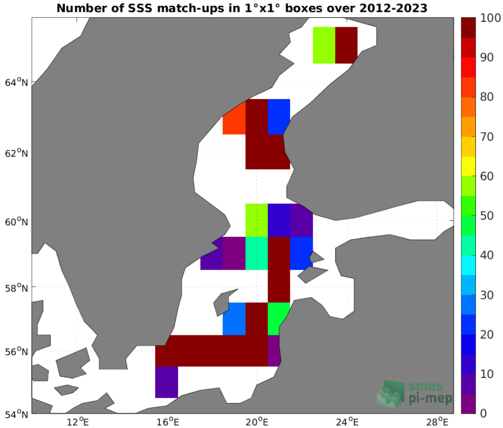
Figure 4: Number of SSS match-ups between Argo SSS and the SMOS SSS L2Q v331 - No FLAG (CMEMS-CATDS-CPDC) SSS product for the Baltic Sea Pi-MEP region over 1^\circ \times 1^\circ boxes and for the full satellite product period.
