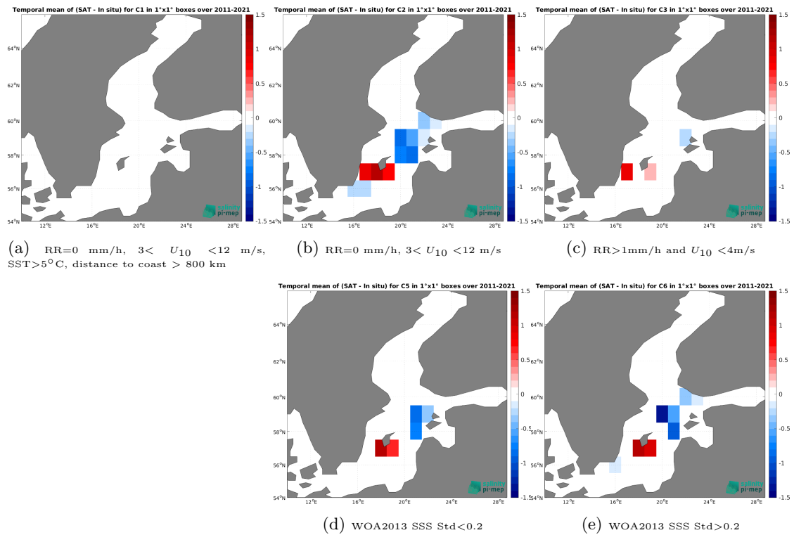
Figure 14: Temporal mean gridded over spatial boxes of size 1^\circ \times 1^\circ of \Delta SSS (SMOS SSS L3 v9 - 9 Days (CATDS-CEC-LOCEAN) - TSG (LEGOS-DM)) for 5 different subdatasets corresponding to:RR=0 mm/h, 3 < U_{10} < 12 m/s, SST >5^\circ\text{C} , distance to coast > 800 km (a), RR=0 mm/h, 3 < U_{10} < 12 m/s (b), RR >1 mm/h and U_{10} < 4 m/s (c), WOA2013 SSS Std <0.2 (d), WOA2013 SSS Std >0.2 (e).
