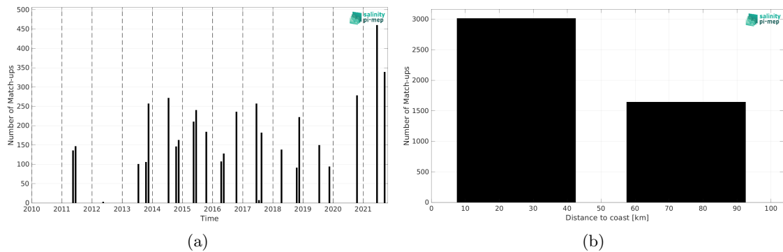
Figure 2: Number of match-ups between TSG (LEGOS-DM) and SMOS SSS L3 v9 - 9 Days (CATDS-CEC-LOCEAN) SSS as a function of time (a) and as function of the distance to coast (b) over the Baltic Sea Pi-MEP region and for the full satellite product period.
