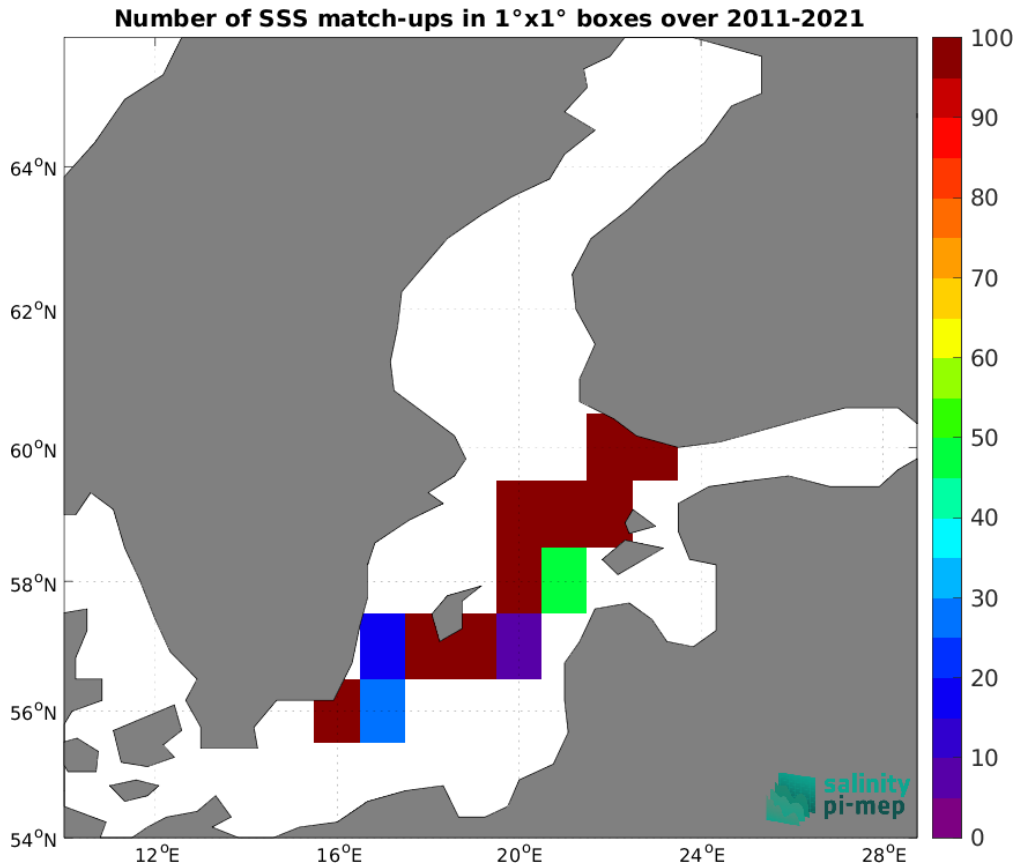
Figure 5: Number of SSS match-ups between TSG (LEGOS-DM) SSS and the SMOS SSS L3 v9 - 9 Days (CATDS-CEC-LOCEAN) SSS product for the Baltic Sea Pi-MEP region over 1^\circ \times 1^\circ boxes and for the full satellite product period.
