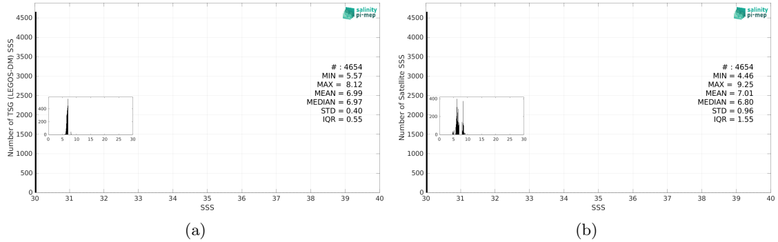
Figure 2: Histograms of SSS from TSG (LEGOS-DM) (a) and SMOS SSS L3 v9 - 9 Days (CATDS-CEC-LOCEAN) (b) considering all match-up pairs per bins of 0.1 over the Baltic Sea Pi-MEP region and for the full satellite product period.
