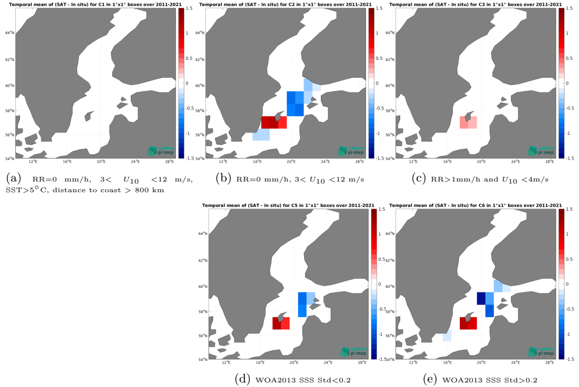
Figure 12: Temporal mean gridded over spatial boxes of size 1^{\circ}\times 1^{\circ} of \Delta\text{SSS} (SMOS SSS L3 v9 - 9 Days (CATDS-CEC-LOCEAN) - TSG (LEGOS-DM)) for 5 different subdatasets corresponding to:RR=0 mm/h, 3 < U_{10} < 12 m/s, SST >5^{\circ}\text{C} , distance to coast > 800 km (a), RR=0 mm/h, 3 < U_{10} < 12 m/s (b), RR >1 mm/h and U_{10} < 4 m/s (c), WOA2013 SSS Std <0.2 (d), WOA2013 SSS Std >0.2 (e).
