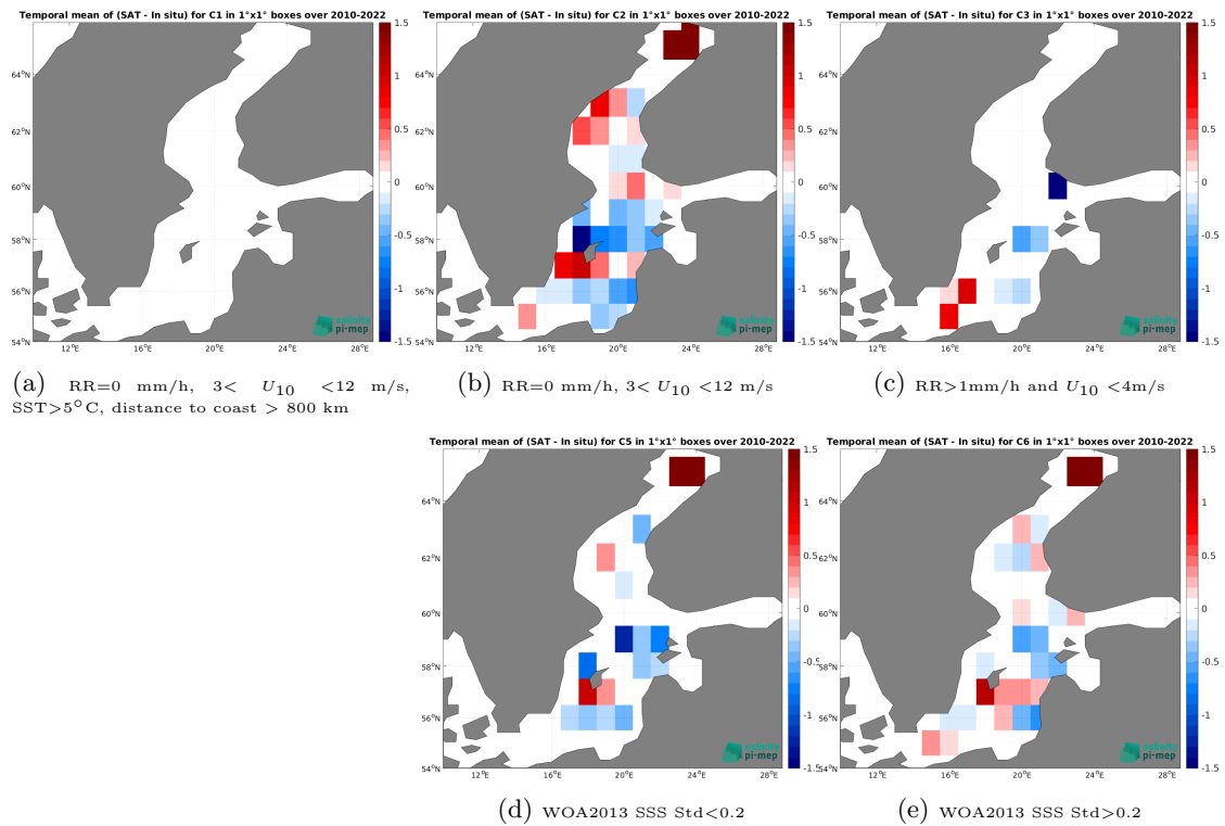
Figure 14: Temporal mean gridded over spatial boxes of size 1^\circ \times 1^\circ of \Delta SSS (SMOS SSS L3 v9 - 9 Days (CATDS-CEC-LOCEAN) - ICES) for 5 different subdatasets corresponding to:RR=0 mm/h, 3 < U_{10} < 12 m/s, SST >5^\circ\text{C} , distance to coast > 800 km (a), RR=0 mm/h, 3 < U_{10} < 12 m/s (b), RR >1 mm/h and U_{10} < 4 m/s (c), WOA2013 SSS Std <0.2 (d), WOA2013 SSS Std >0.2 (e).
