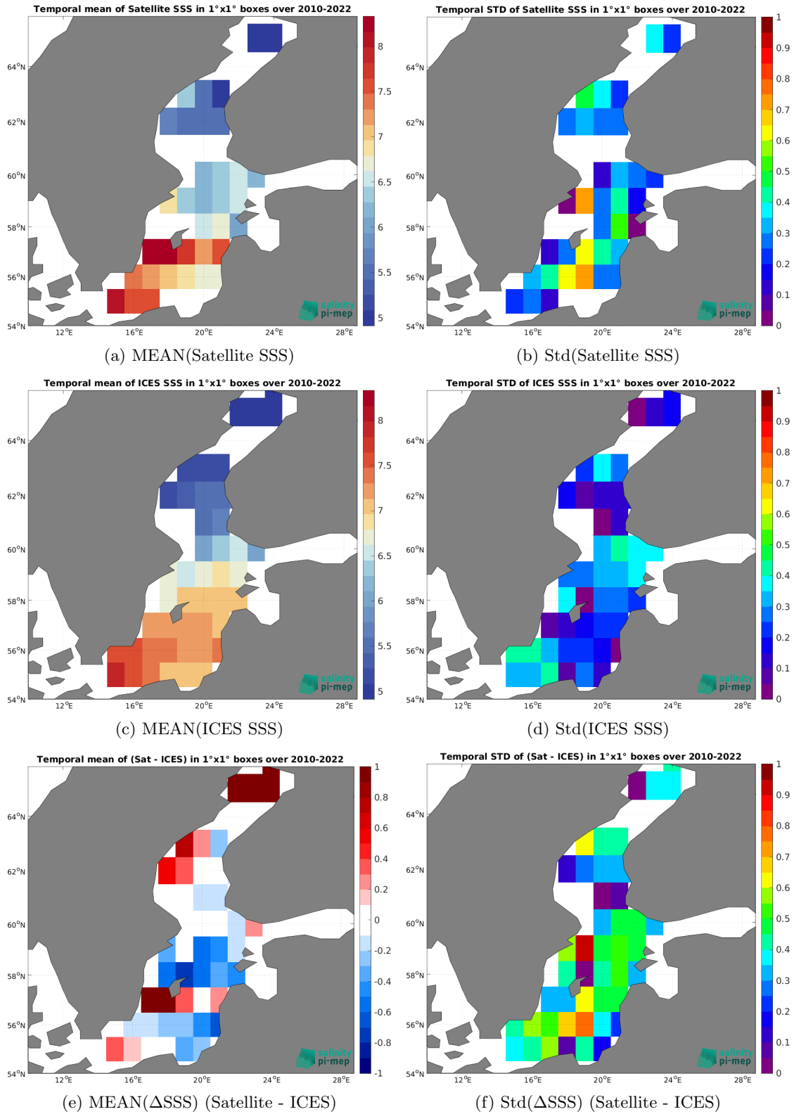
Figure 7: Temporal mean (left) and Std (right) of SSS from SMOS SSS L3 v9 - 9 Days (CATDS-CEC-LOCEAN) (top), ICES (middle), and of \Delta SSS (Satellite - ICES). Only match-up pairs are used to generate these maps.
