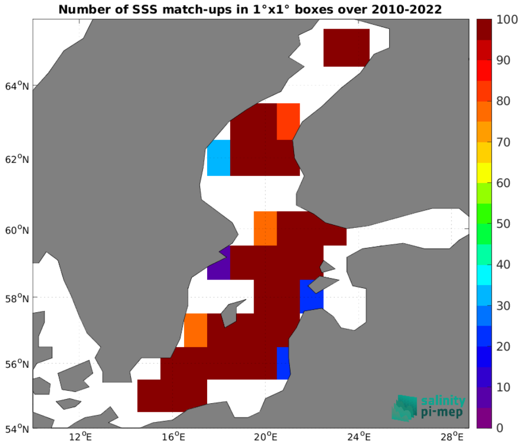
Figure 5: Number of SSS match-ups between ICES SSS and the SMOS SSS L3 v9 - 9 Days (CATDS-CEC-LOCEAN) SSS product for the Baltic Sea Pi-MEP region over 1^\circ \times 1^\circ boxes and for the full satellite product period.
