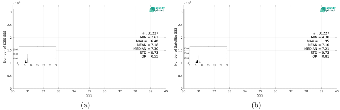
Figure 3: Histograms of SSS from ICES (a) and SMOS SSS L3 v9 - 9 Days (CATDS-CEC-LOCEAN) (b) considering all match-up pairs per bins of 0.1 over the Baltic Sea Pi-MEP region and for the full satellite product period.
