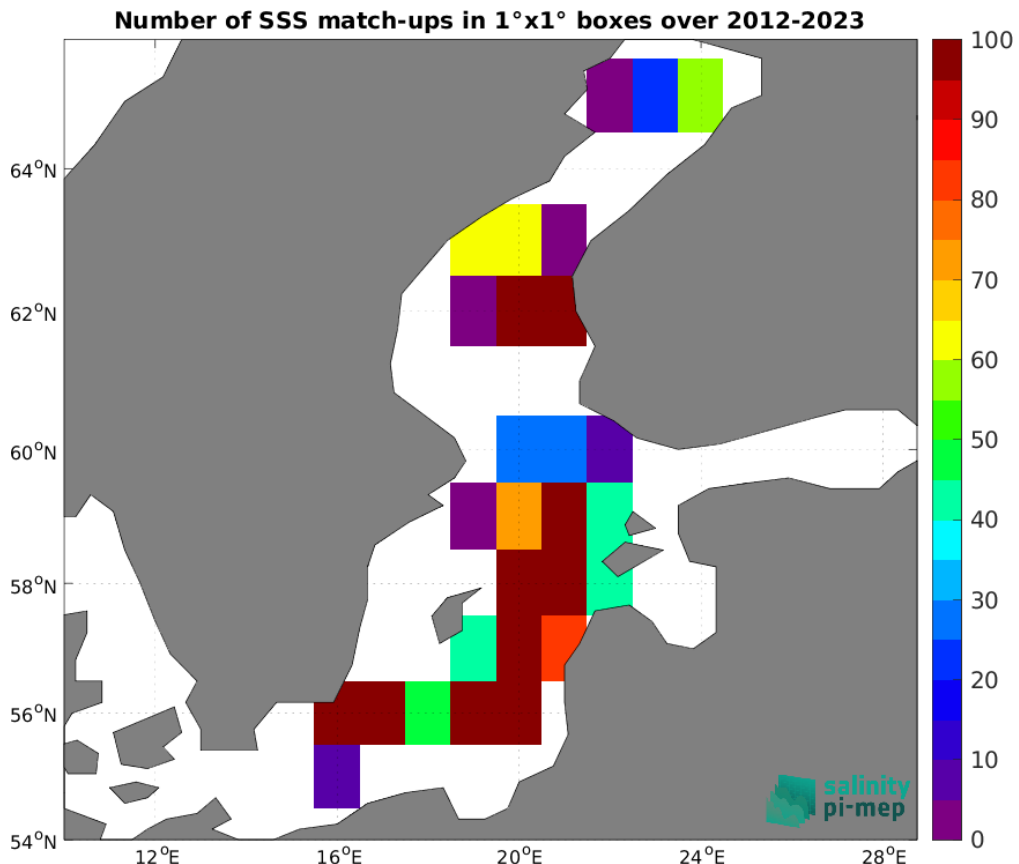
Figure 5: Number of SSS match-ups between Argo SSS and the SMOS SSS L3 v9 - 9 Days (CATDS-CEC-LOCEAN) SSS product for the Baltic Sea Pi-MEP region over 1°x1° boxes and for the full satellite product period.
