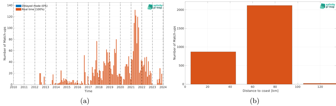
Figure 2: Number of match-ups between Argo and SMOS SSS L3 v9 - 9 Days (CATDS-CEC-LOCEAN) SSS as a function of time (a) and as function of the distance to coast (b) over the Baltic Sea Pi-MEP region and for the full satellite product period.
