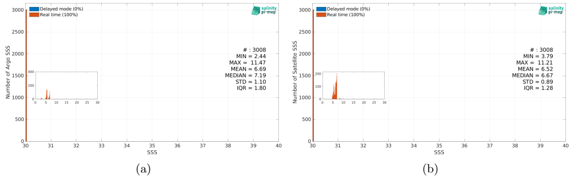
Figure 3: Histograms of SSS from Argo (a) and SMOS SSS L3 v9 - 9 Days (CATDS-CEC-LOCEAN) (b) considering all match-up pairs per bins of 0.1 over the Baltic Sea Pi-MEP region and for the full satellite product period.
