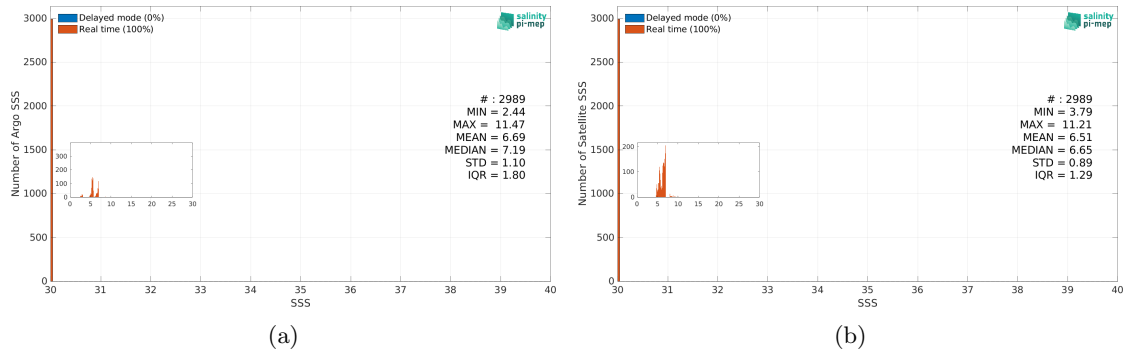
Figure 2: Histograms of SSS from Argo (a) and SMOS SSS L3 v9 - 9 Days (CATDS-CEC-LOCEAN) (b) considering all match-up pairs per bins of 0.1 over the Baltic Sea Pi-MEP region and for the full satellite product period.
