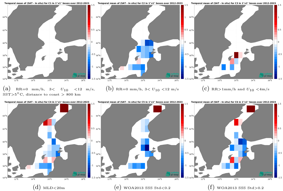
Figure 12: Temporal mean gridded over spatial boxes of size 1^{\circ}\times 1^{\circ} of \Delta\text{SSS} (SMOS SSS L3 v9 - 9 Days (CATDS-CEC-LOCEAN) - Argo) for 6 different subdatasets corresponding to:RR=0 mm/h, 3 < U_{10} < 12 m/s, SST >5^{\circ}\text{C} , distance to coast > 800 km (a), RR=0 mm/h, 3 < U_{10} < 12 m/s (b), RR >1\text{mm/h} and U_{10} < 4\text{m/s} (c),MLD <20\text{m} (d),WOA2013 SSS Std <0.2 (e),WOA2013 SSS Std >0.2 (f).
