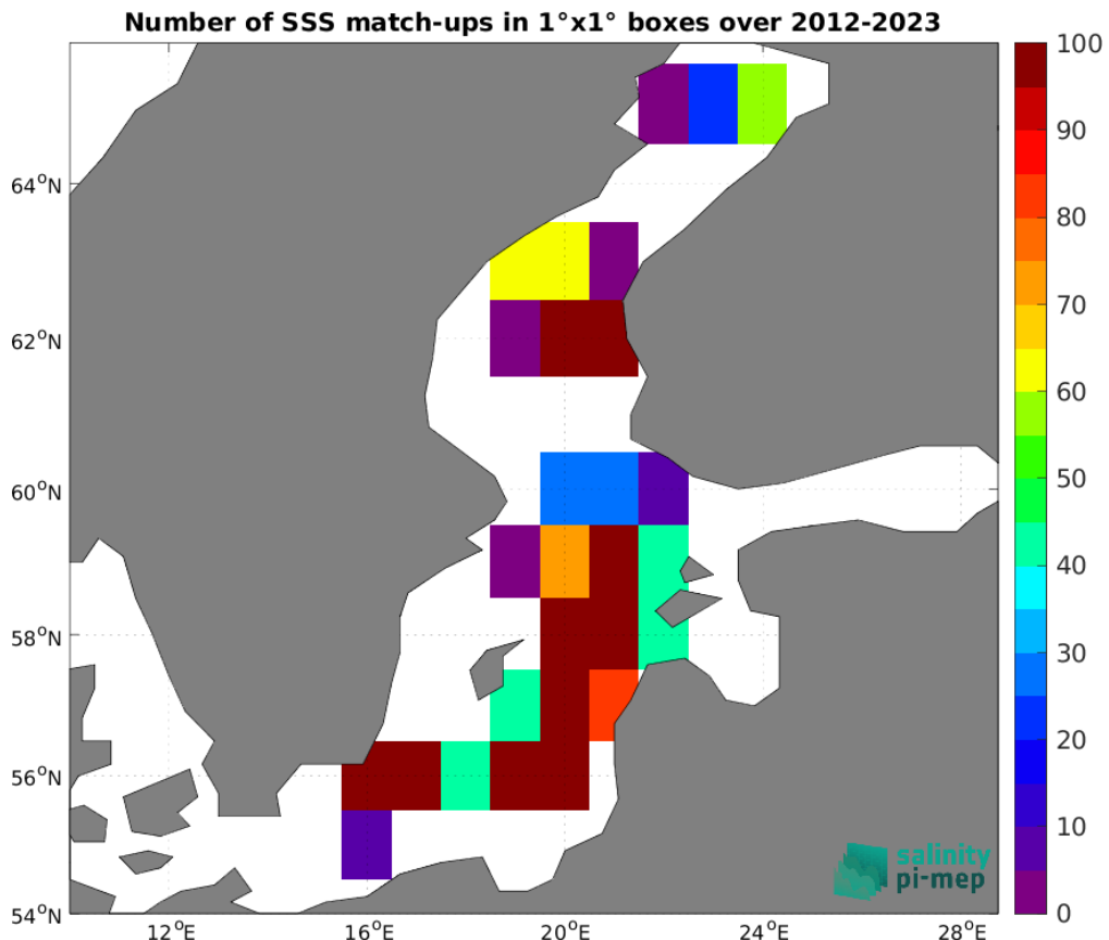
Figure 4: Number of SSS match-ups between Argo SSS and the SMOS SSS L3 v9 - 9 Days (CATDS-CEC-LOCEAN) SSS product for the Baltic Sea Pi-MEP region over 1^{\circ} \times 1^{\circ} boxes and for the full satellite product period.
