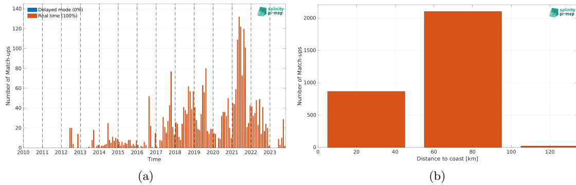
Figure 1: Number of match-ups between Argo and SMOS SSS L3 v9 - 9 Days (CATDS-CEC-LOCEAN) SSS as a function of time (a) and as function of the distance to coast (b) over the Baltic Sea Pi-MEP region and for the full satellite product period.
