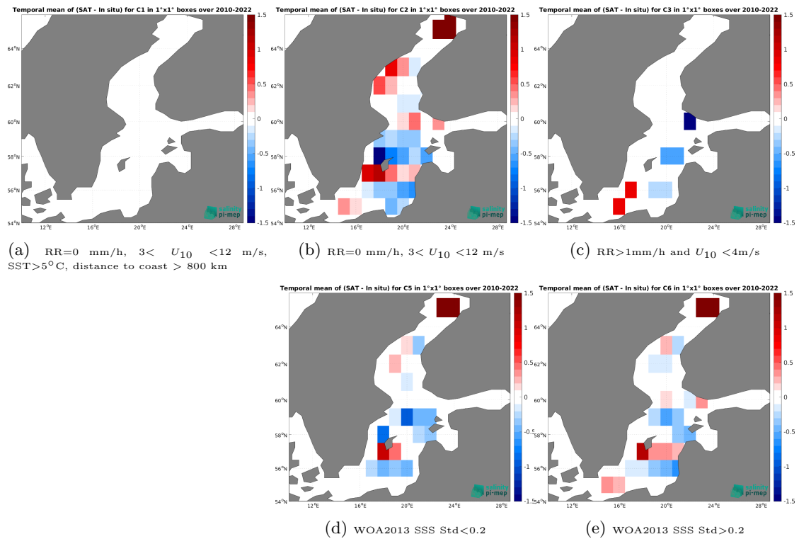
Figure 14: Temporal mean gridded over spatial boxes of size 1^\circ \times 1^\circ of \Delta\text{SSS} (SMOS SSS L3 v9 - 18 Days (CATDS-CEC-LOCEAN) - ICES) for 5 different subdatasets corresponding to:RR=0 mm/h, 3 < U_{10} < 12 m/s, SST>5°C, distance to coast > 800 km (a), RR=0 mm/h, 3 < U_{10} < 12 m/s (b), RR>1mm/h and U_{10} < 4 m/s (c), WOA2013 SSS Std<0.2 (d), WOA2013 SSS Std>0.2 (e).
