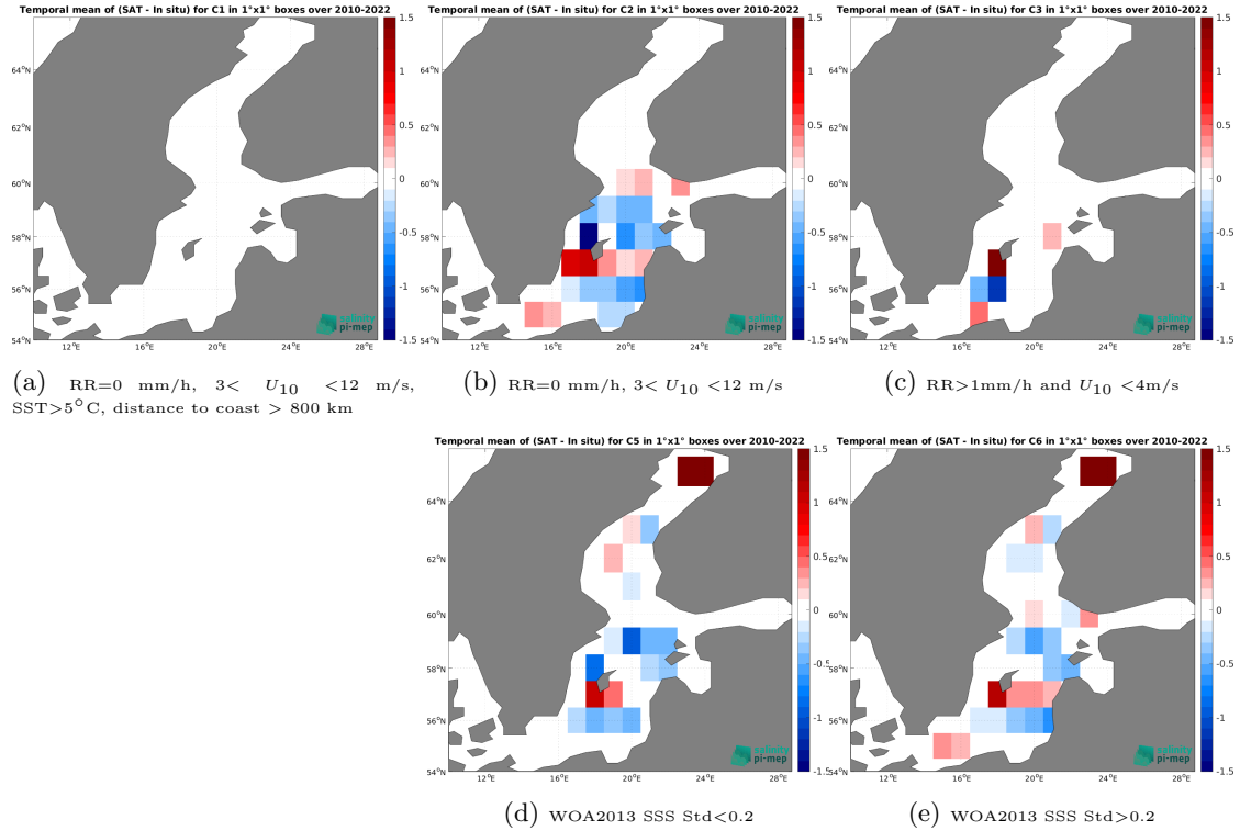
Figure 12: Temporal mean gridded over spatial boxes of size 1^{\circ}\times 1^{\circ} of \Delta\text{SSS} (SMOS SSS L3 v9 - 18 Days (CATDS-CEC-LOCEAN) - ICES) for 5 different subdatasets corresponding to:RR=0 mm/h, 3 < U_{10} < 12 m/s, SST > 5^{\circ}\text{C} , distance to coast > 800 km (a), RR=0 mm/h, 3 < U_{10} < 12 m/s (b), RR > 1 mm/h and U_{10} < 4 m/s (c), WOA2013 SSS Std < 0.2 (d), WOA2013 SSS Std > 0.2 (e).
