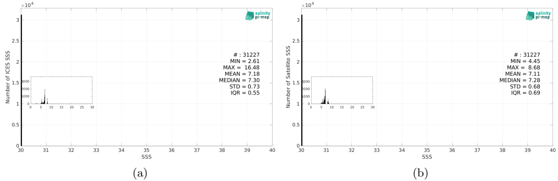
Figure 2: Histograms of SSS from ICES (a) and SMOS SSS L3 v9 - 18 Days (CATDS-CEC-LOCEAN) (b) considering all match-up pairs per bins of 0.1 over the Baltic Sea Pi-MEP region and for the full satellite product period.
