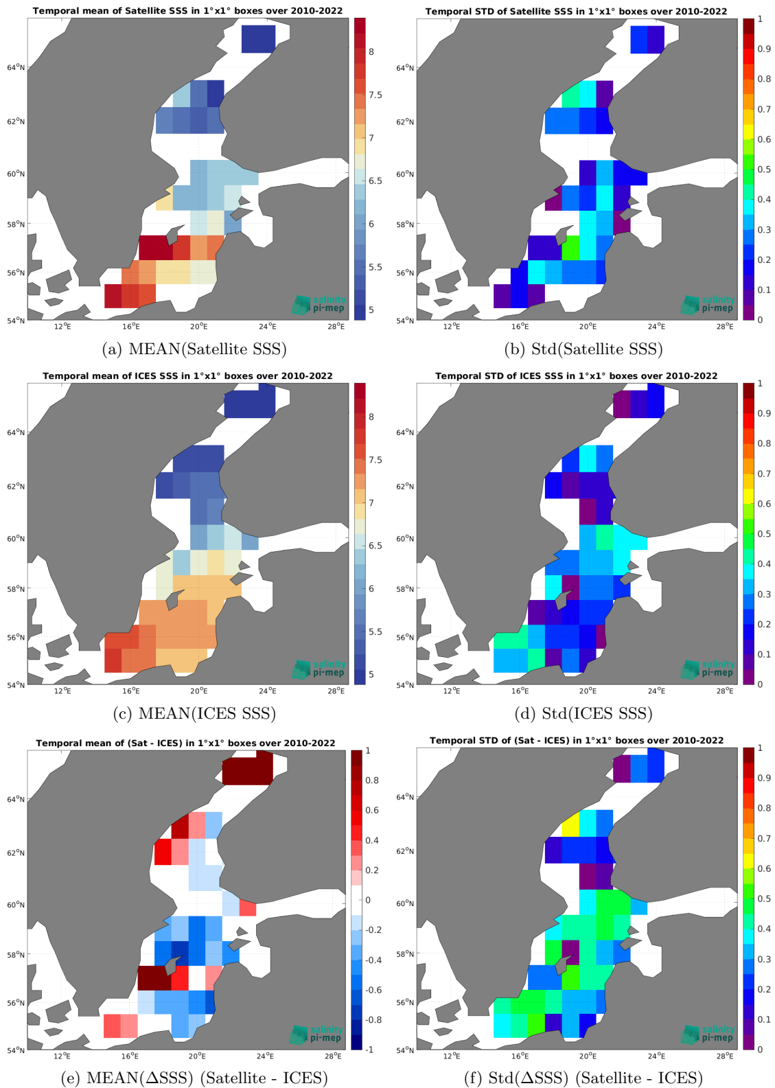
Figure 6: Temporal mean (left) and Std (right) of SSS from SMOS SSS L3 v9 - 18 Days (CATDS-CEC-LOCEAN) (top), ICES (middle), and of \Delta SSS (Satellite - ICES). Only match-up pairs are used to generate these maps.
