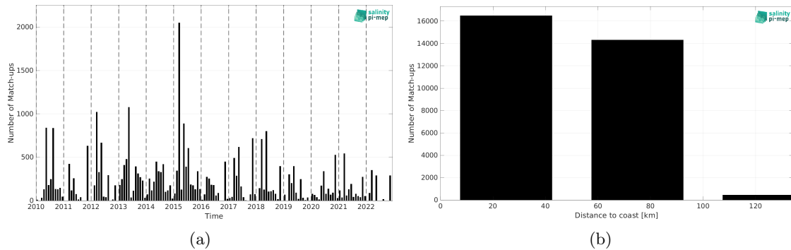
Figure 1: Number of match-ups between ICES and SMOS SSS L3 v9 - 18 Days (CATDS-CEC-LOCEAN) SSS as a function of time (a) and as function of the distance to coast (b) over the Baltic Sea Pi-MEP region and for the full satellite product period.
