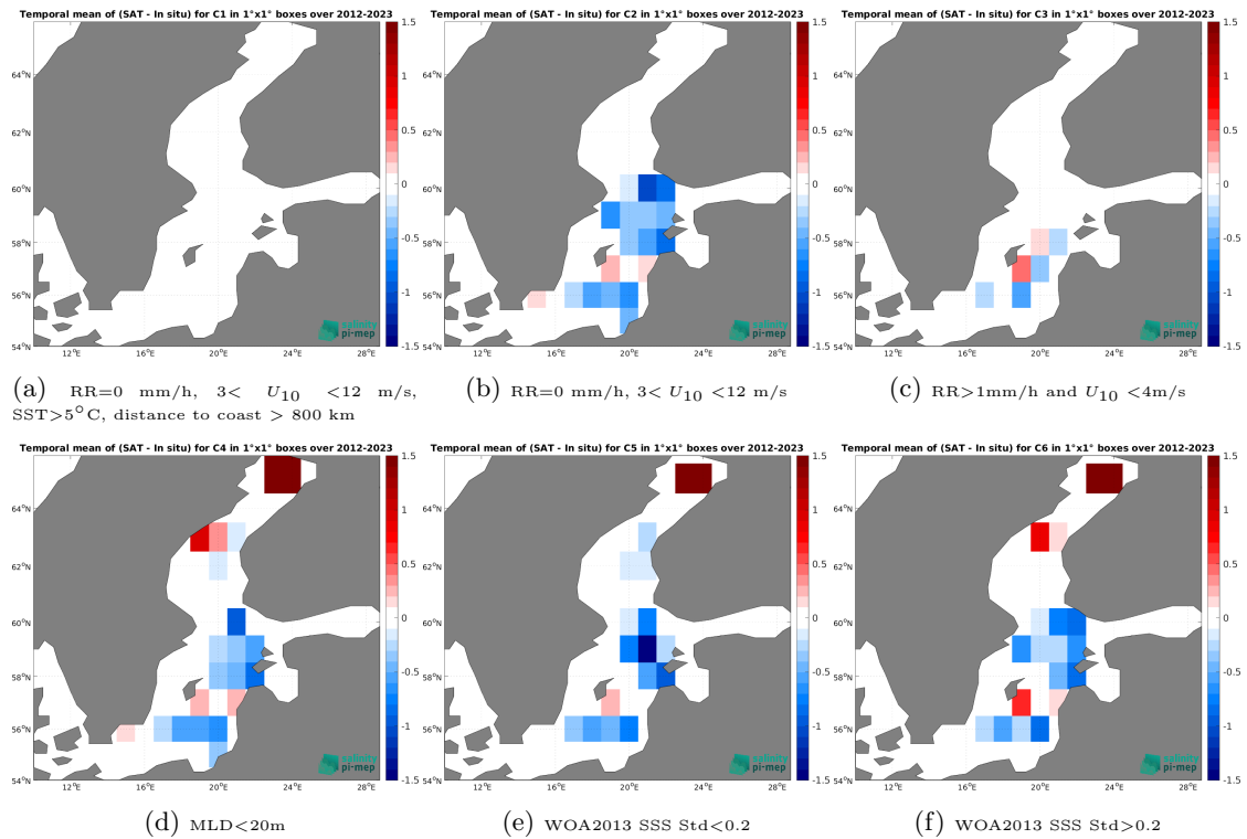
Figure 12: Temporal mean gridded over spatial boxes of size 1^{\circ}\times 1^{\circ} of \Delta\text{SSS} (SMOS SSS L3 v9 - 18 Days (CATDS-CEC-LOCEAN) - Argo) for 6 different subdatasets corresponding to:RR=0 mm/h, 3 < U_{10} < 12 m/s, SST >5^{\circ}\text{C} , distance to coast > 800 km (a), RR=0 mm/h, 3 < U_{10} < 12 m/s (b), RR >1\text{mm/h} and U_{10} < 4\text{m/s} (c),MLD <20\text{m} (d),WOA2013 SSS Std <0.2 (e),WOA2013 SSS Std >0.2 (f).
