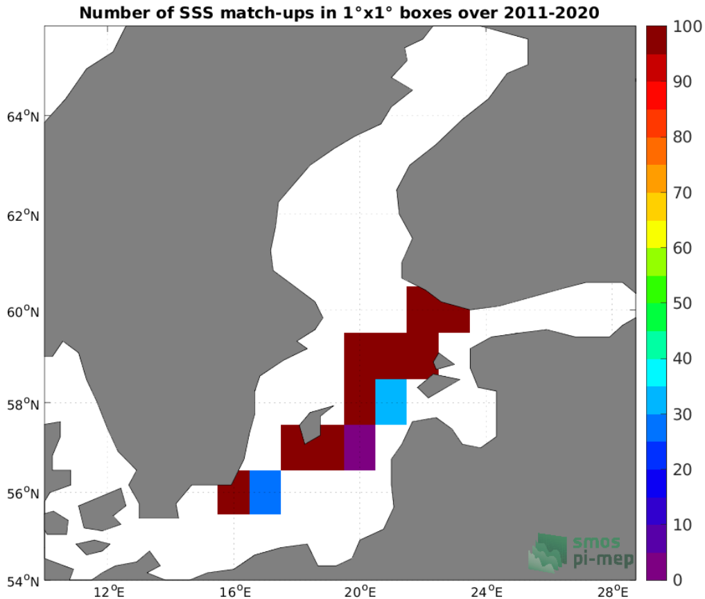
Figure 4: Number of SSS match-ups between TSG (LEGOS-DM) SSS and the SMOS SSS L3 v8 - 9 Days (CATDS-CECOS-LOCEAN) SSS product for the Baltic Sea Pi-MEP region over 1^\circ \times 1^\circ boxes and for the full satellite product period.
