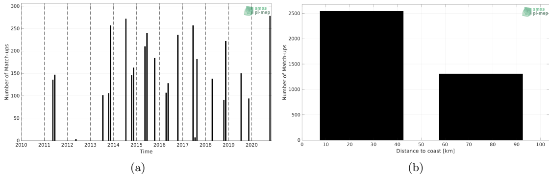
Figure 1: Number of match-ups between TSG (LEGOS-DM) and SMOS SSS L3 v8 - 9 Days (CATDS-CECOS-LOCEAN) SSS as a function of time (a) and as function of the distance to coast (b) over the Baltic Sea Pi-MEP region and for the full satellite product period.
