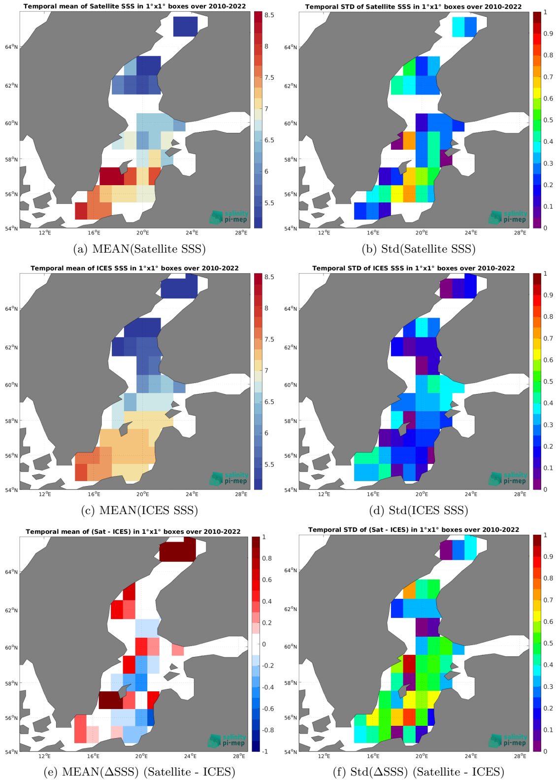
Figure 6: Temporal mean (left) and Std (right) of SSS from SMOS SSS L3 v8 - 9 Days (CATDS-CEC-LOCEAN) (top), ICES (middle), and of \Delta SSS (Satellite - ICES). Only match-up pairs are used to generate these maps.
