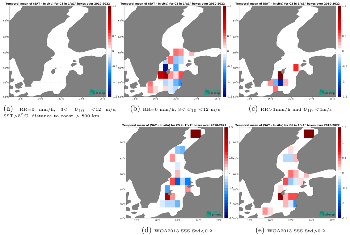
Figure 12: Temporal mean gridded over spatial boxes of size 1^{\circ}\times 1^{\circ} of \Delta\text{SSS} (SMOS SSS L3 v8 - 9 Days (CATDS-CEC-LOCEAN) - ICES) for 5 different subdatasets corresponding to:RR=0 mm/h, 3 < U_{10} < 12 m/s, SST > 5^{\circ}\text{C} , distance to coast > 800 km (a), RR=0 mm/h, 3 < U_{10} < 12 m/s (b), RR > 1 mm/h and U_{10} < 4 m/s (c), WOA2013 SSS Std < 0.2 (d), WOA2013 SSS Std > 0.2 (e).
