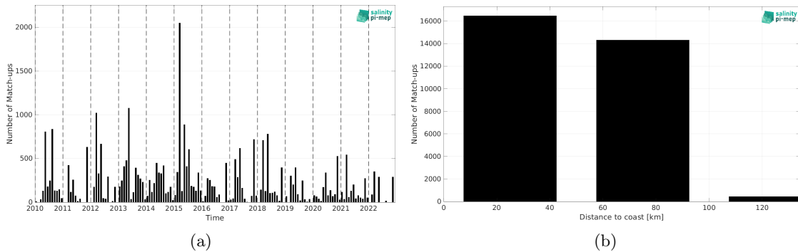
Figure 1: Number of match-ups between ICES and SMOS SSS L3 v8 - 9 Days (CATDS-CEC-LOCEAN) SSS as a function of time (a) and as function of the distance to coast (b) over the Baltic Sea Pi-MEP region and for the full satellite product period.
