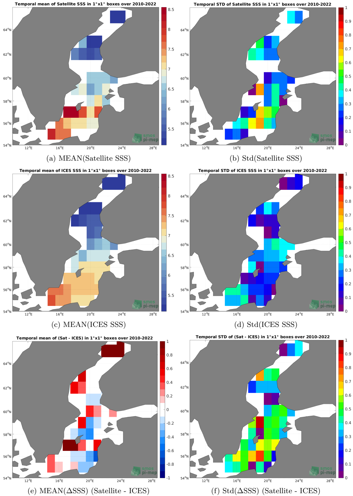
Figure 6: Temporal mean (left) and Std (right) of SSS from SMOS SSS L3 v8 - 9 Days (CATDS-CECOS-LOCEAN) (top), ICES (middle), and of \Delta SSS (Satellite - ICES). Only match-up pairs are used to generate these maps.
