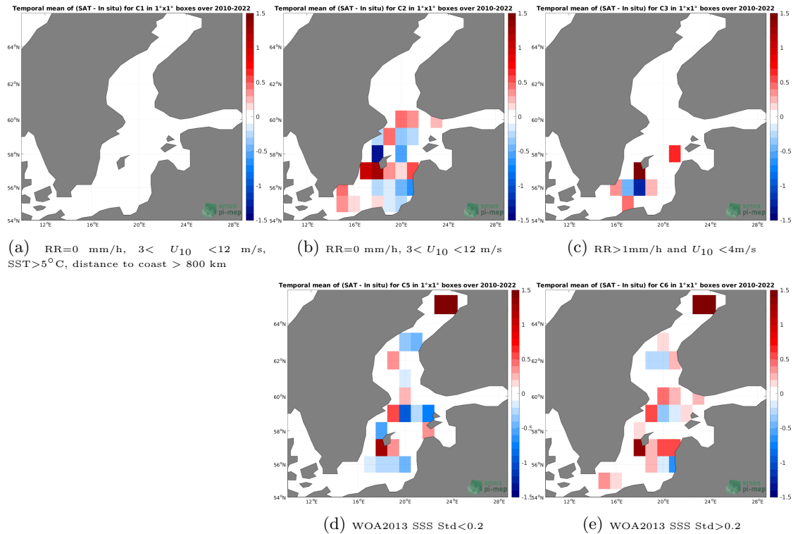
Figure 12: Temporal mean gridded over spatial boxes of size 1^{\circ}\times 1^{\circ} of \Delta\text{SSS} (SMOS SSS L3 v8 - 9 Days (CATDS-CECOS-LOCEAN) - ICES) for 5 different subdatasets corresponding to:RR=0 mm/h, 3 < U_{10} < 12 m/s, SST > 5^{\circ}\text{C} , distance to coast > 800 km (a), RR=0 mm/h, 3 < U_{10} < 12 m/s (b), RR > 1 mm/h and U_{10} < 4 m/s (c), WOA2013 SSS Std < 0.2 (d), WOA2013 SSS Std > 0.2 (e).
