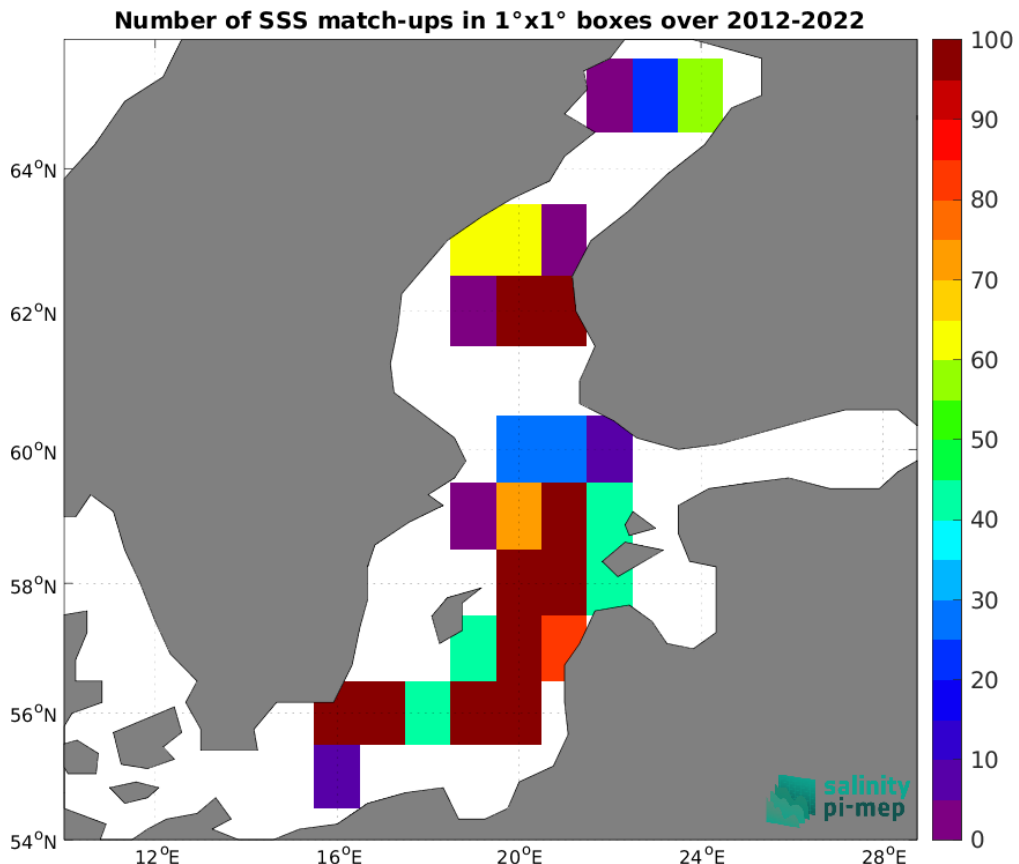
Figure 4: Number of SSS match-ups between Argo SSS and the SMOS SSS L3 v8 - 9 Days (CATDS-CEC-LOCEAN) SSS product for the Baltic Sea Pi-MEP region over 1°x1° boxes and for the full satellite product period.
