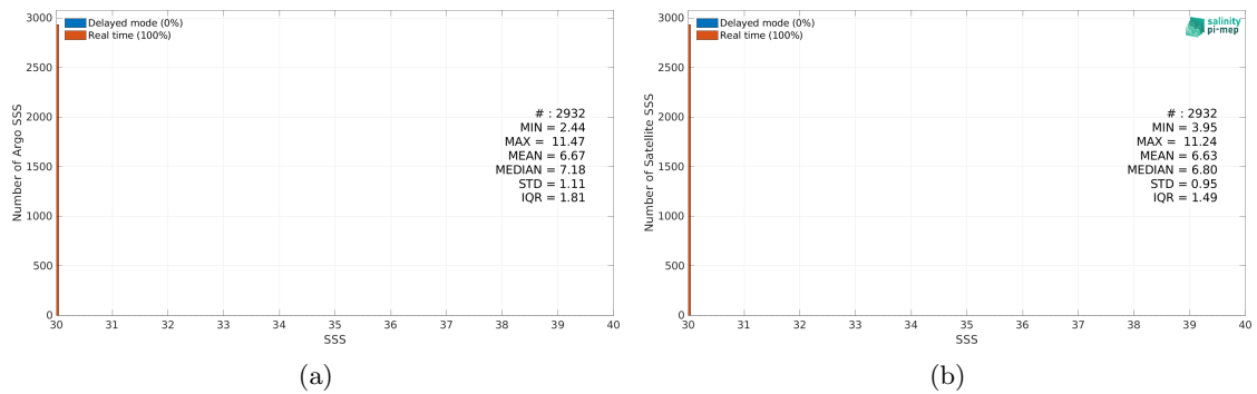
Figure 2: Histograms of SSS from Argo (a) and SMOS SSS L3 v8 - 9 Days (CATDS-CEC-LOCEAN) (b) considering all match-up pairs per bins of 0.1 over the Baltic Sea Pi-MEP region and for the full satellite product period.
