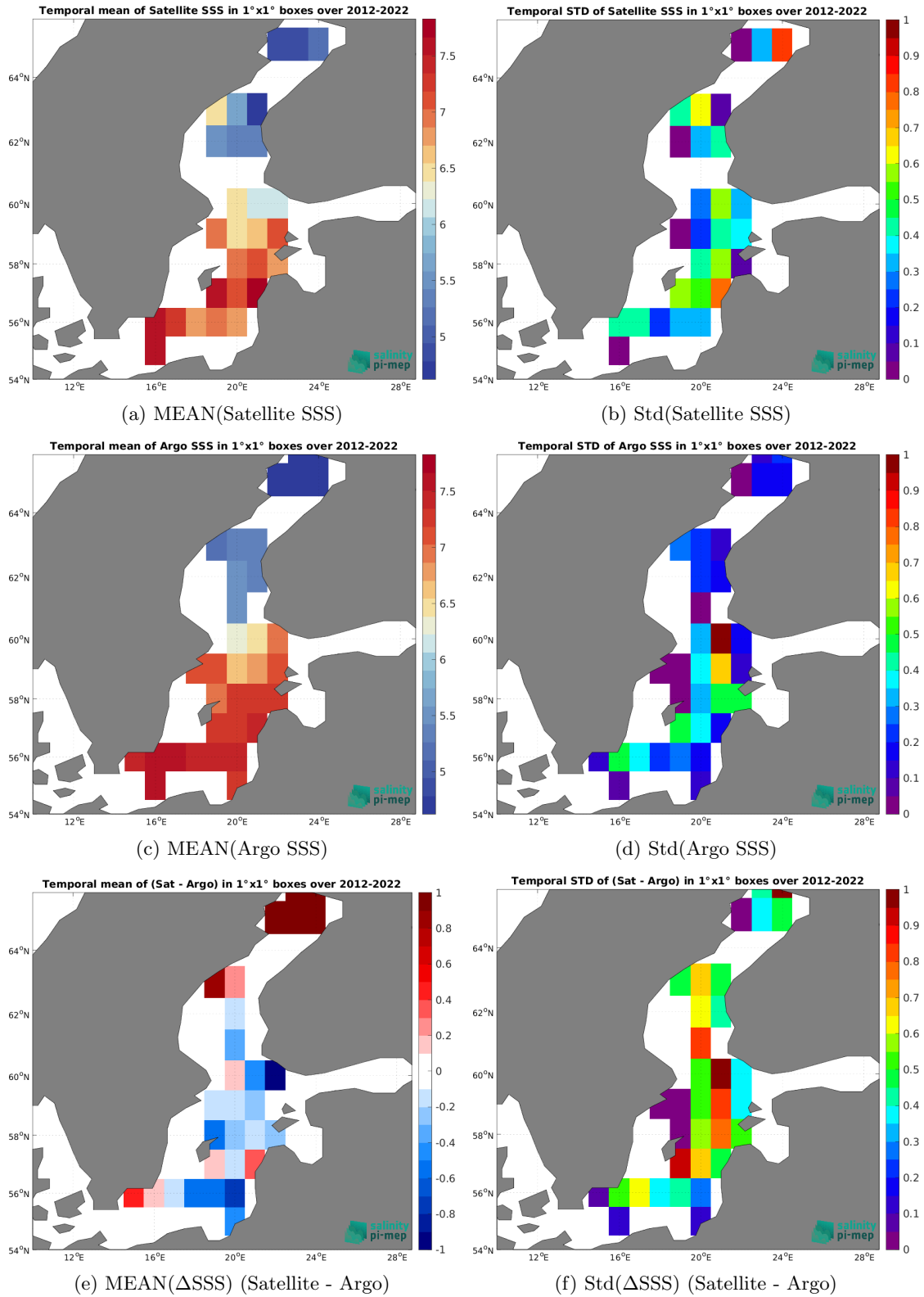
Figure 6: Temporal mean (left) and Std (right) of SSS from SMOS SSS L3 v8 - 9 Days (CATDS-CEC-LOCEAN) (top), Argo (middle), and of \Delta SSS (Satellite - Argo). Only match-up pairs are used to generate these maps.
