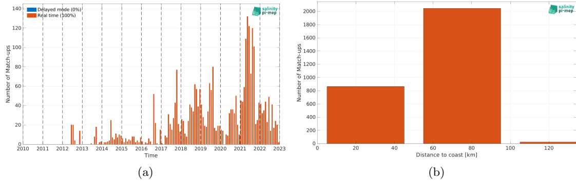
Figure 1: Number of match-ups between Argo and SMOS SSS L3 v8 - 9 Days (CATDS-CEC-LOCEAN) SSS as a function of time (a) and as function of the distance to coast (b) over the Baltic Sea Pi-MEP region and for the full satellite product period.
