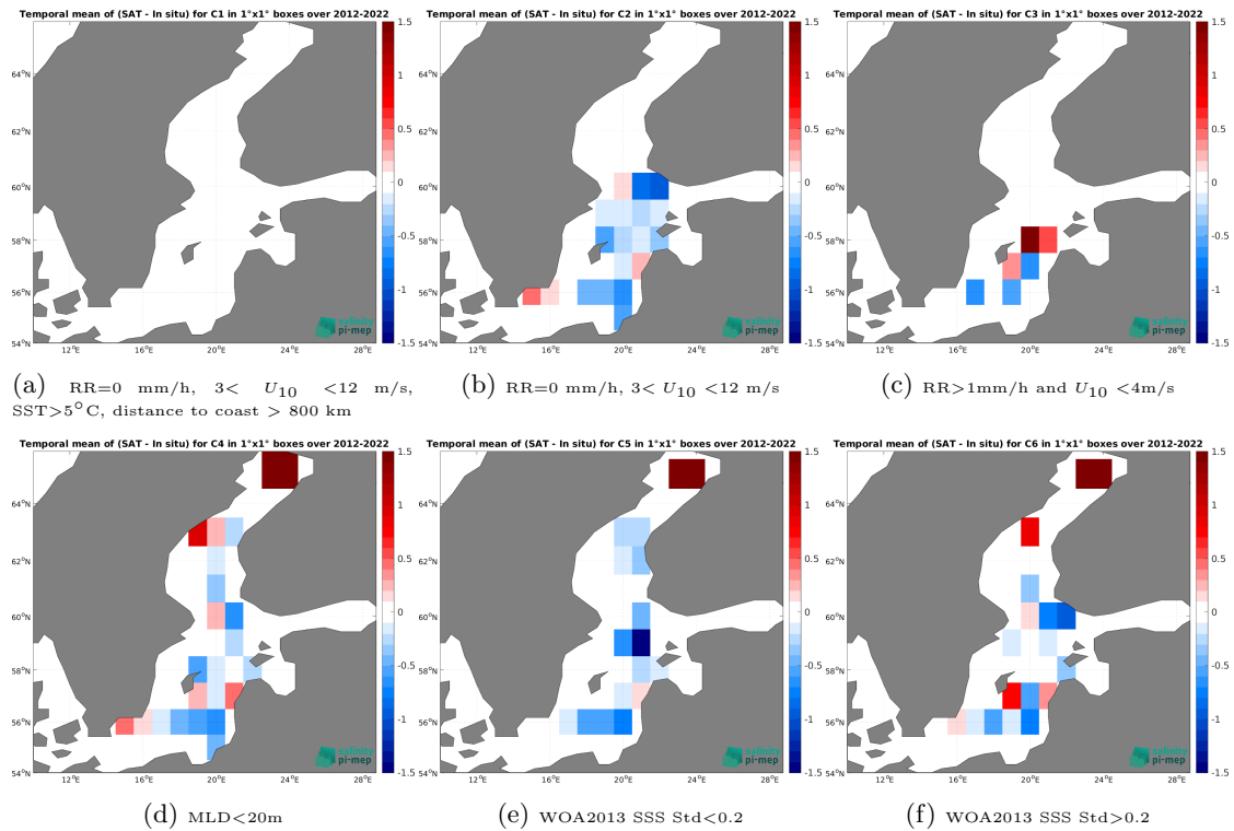
Figure 12: Temporal mean gridded over spatial boxes of size 1^{\circ}\times 1^{\circ} of \Delta\text{SSS} (SMOS SSS L3 v8 - 9 Days (CATDS-CEC-LOCEAN) - Argo) for 6 different subdatasets corresponding to:RR=0 mm/h, 3 < U_{10} < 12 m/s, SST >5^{\circ}\text{C} , distance to coast > 800 km (a), RR=0 mm/h, 3 < U_{10} < 12 m/s (b), RR >1\text{mm/h} and U_{10} < 4\text{m/s} (c),MLD <20\text{m} (d),WOA2013 SSS Std <0.2 (e),WOA2013 SSS Std >0.2 (f).
