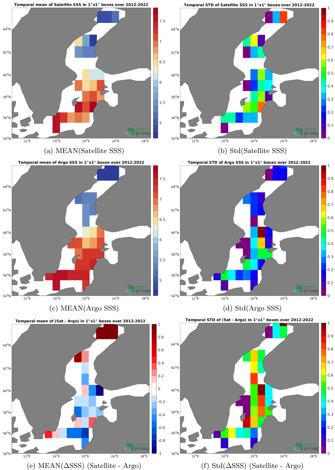
Figure 6: Temporal mean (left) and Std (right) of SSS from SMOS SSS L3 v8 - 9 Days (CATDS-CECOS-LOCEAN) (top), Argo (middle), and of \Delta SSS (Satellite - Argo). Only match-up pairs are used to generate these maps.
