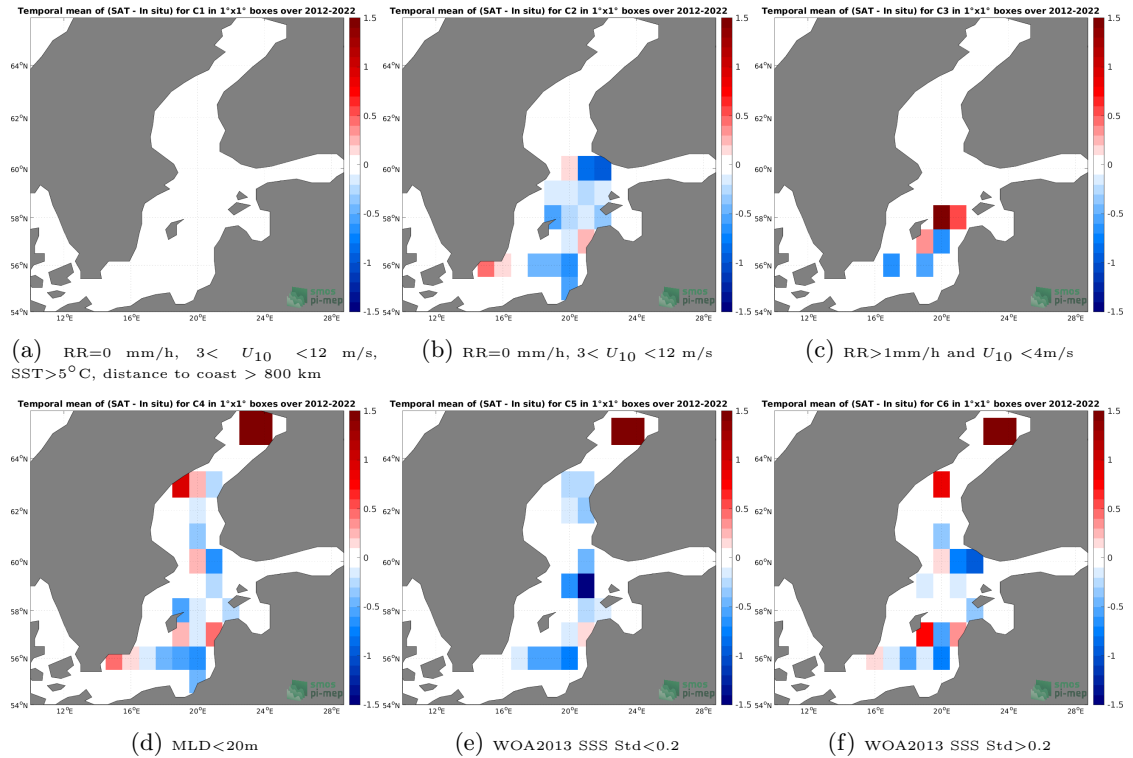
Figure 12: Temporal mean gridded over spatial boxes of size 1^{\circ}\times 1^{\circ} of \Delta\text{SSS} (SMOS SSS L3 v8 - 9 Days (CATDS-CECOS-LOCEAN) - Argo) for 6 different subdatasets corresponding to:RR=0 mm/h, 3 < U_{10} < 12 m/s, SST >5^{\circ}\text{C} , distance to coast > 800 km (a), RR=0 mm/h, 3 < U_{10} < 12 m/s (b), RR >1 mm/h and U_{10} < 4 m/s (c),MLD <20 m (d),WOA2013 SSS Std <0.2 (e),WOA2013 SSS Std >0.2 (f).
