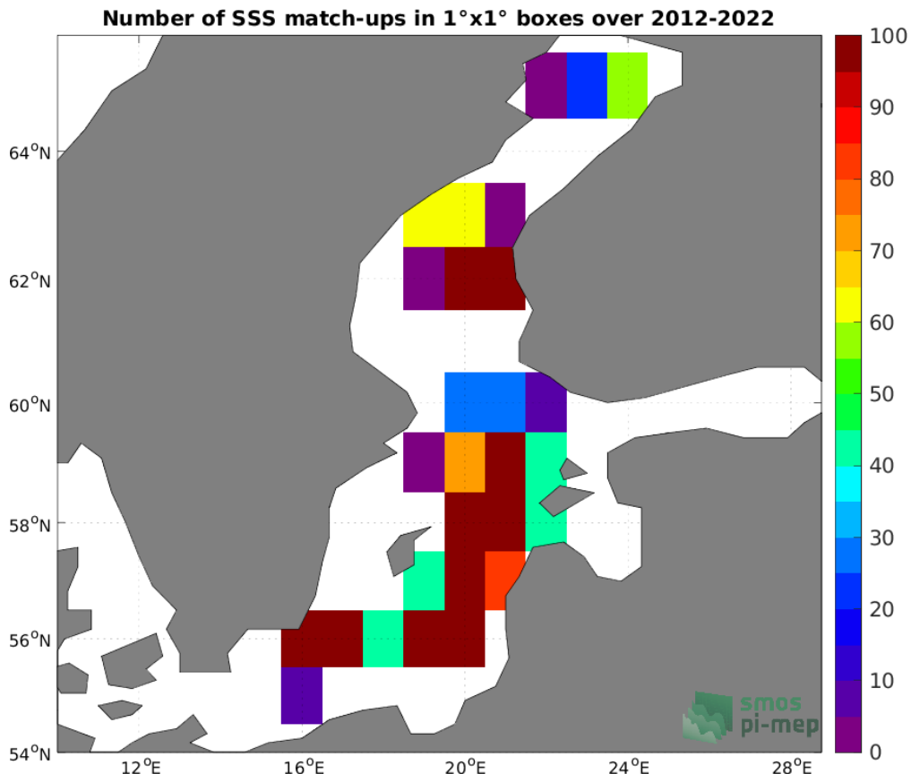
Figure 4: Number of SSS match-ups between Argo SSS and the SMOS SSS L3 v8 - 9 Days (CATDS-CECOS-LOCEAN) SSS product for the Baltic Sea Pi-MEP region over 1°x1° boxes and for the full satellite product period.
