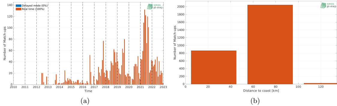
Figure 1: Number of match-ups between Argo and SMOS SSS L3 v8 - 9 Days (CATDS-CECOS-LOCEAN) SSS as a function of time (a) and as function of the distance to coast (b) over the Baltic Sea Pi-MEP region and for the full satellite product period.
