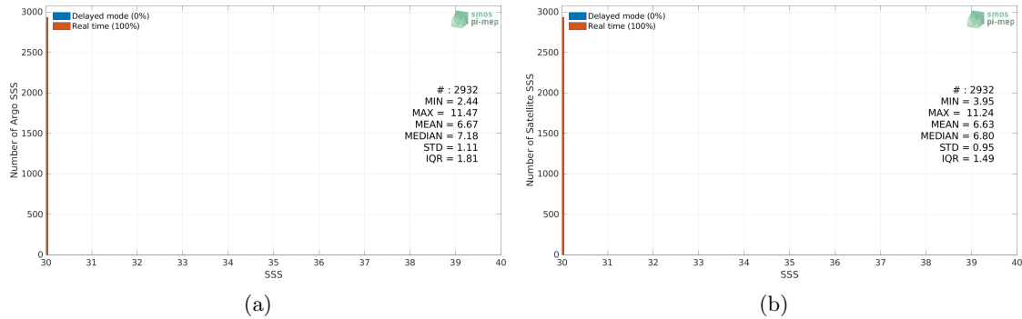
Figure 2: Histograms of SSS from Argo (a) and SMOS SSS L3 v8 - 9 Days (CATDS-CECOS-LOCEAN) (b) considering all match-up pairs per bins of 0.1 over the Baltic Sea Pi-MEP region and for the full satellite product period.
