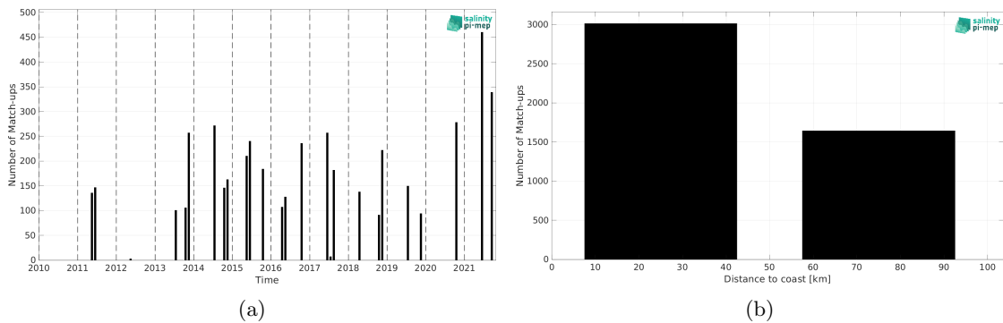
Figure 1: Number of match-ups between TSG (LEGOS-DM) and SMOS SSS L3 v8 - 18 Days (CATDS-CEC-LOCEAN) SSS as a function of time (a) and as function of the distance to coast (b) over the Baltic Sea Pi-MEP region and for the full satellite product period.
