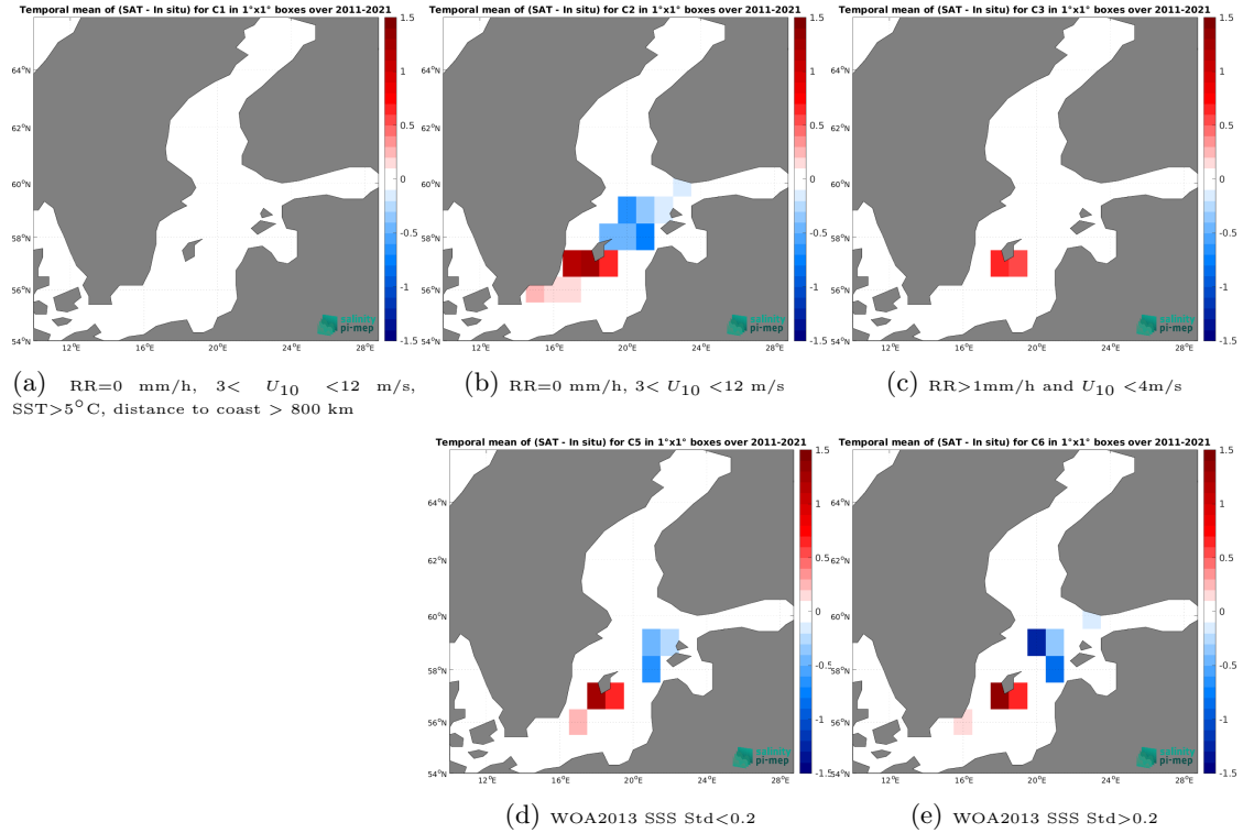
Figure 12: Temporal mean gridded over spatial boxes of size 1^{\circ}\times 1^{\circ} of \Delta\text{SSS} (SMOS SSS L3 v8 - 18 Days (CATDS-CEC-LOCEAN) - TSG (LEGOS-DM)) for 5 different subdatasets corresponding to: \text{RR}=0 mm/h, 3 < U_{10} < 12 m/s, \text{SST} > 5^{\circ}\text{C} , distance to coast > 800 km (a), \text{RR}=0 mm/h, 3 < U_{10} < 12 m/s (b), \text{RR} > 1\text{mm/h} and U_{10} < 4\text{m/s} (c), WOA2013 SSS Std < 0.2 (d), WOA2013 SSS Std > 0.2 (e).
