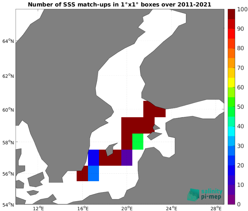
Figure 4: Number of SSS match-ups between TSG (LEGOS-DM) SSS and the SMOS SSS L3 v8 - 18 Days (CATDS-CEC-LOCEAN) SSS product for the Baltic Sea Pi-MEP region over 1^\circ \times 1^\circ boxes and for the full satellite product period.
