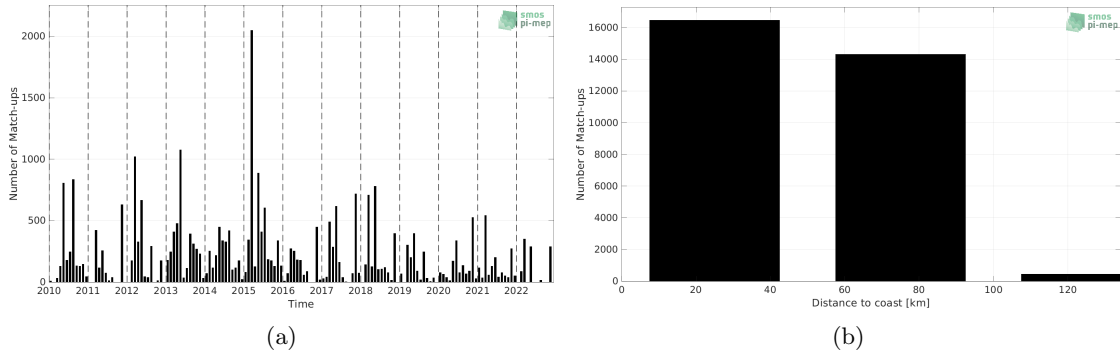
Figure 1: Number of match-ups between ICES and SMOS SSS L3 v8 - 18 Days (CATDS-CECOS-LOCEAN) SSS as a function of time (a) and as function of the distance to coast (b) over the Baltic Sea Pi-MEP region and for the full satellite product period.
