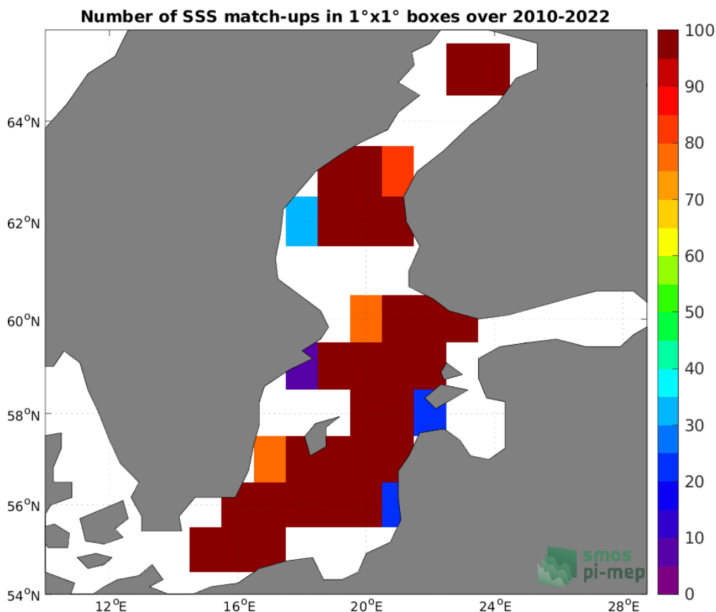
Figure 4: Number of SSS match-ups between ICES SSS and the SMOS SSS L3 v8 - 18 Days (CATDS-CECOS-LOCEAN) SSS product for the Baltic Sea Pi-MEP region over 1^\circ \times 1^\circ boxes and for the full satellite product period.
