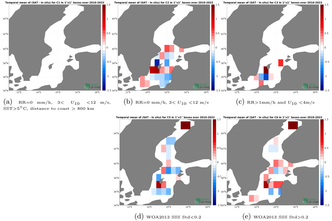
Figure 12: Temporal mean gridded over spatial boxes of size 1^{\circ}\times 1^{\circ} of \Delta\text{SSS} (SMOS SSS L3 v8 - 18 Days (CATDS-CECOS-LOCEAN) - ICES) for 5 different subdatasets corresponding to: \text{RR}=0 mm/h, 3 < U_{10} < 12 m/s, \text{SST} > 5^{\circ}\text{C} , distance to coast > 800 km (a), \text{RR}=0 mm/h, 3 < U_{10} < 12 m/s (b), \text{RR} > 1\text{mm/h} and U_{10} < 4\text{m/s} (c), WOA2013 SSS Std < 0.2 (d), WOA2013 SSS Std > 0.2 (e).
