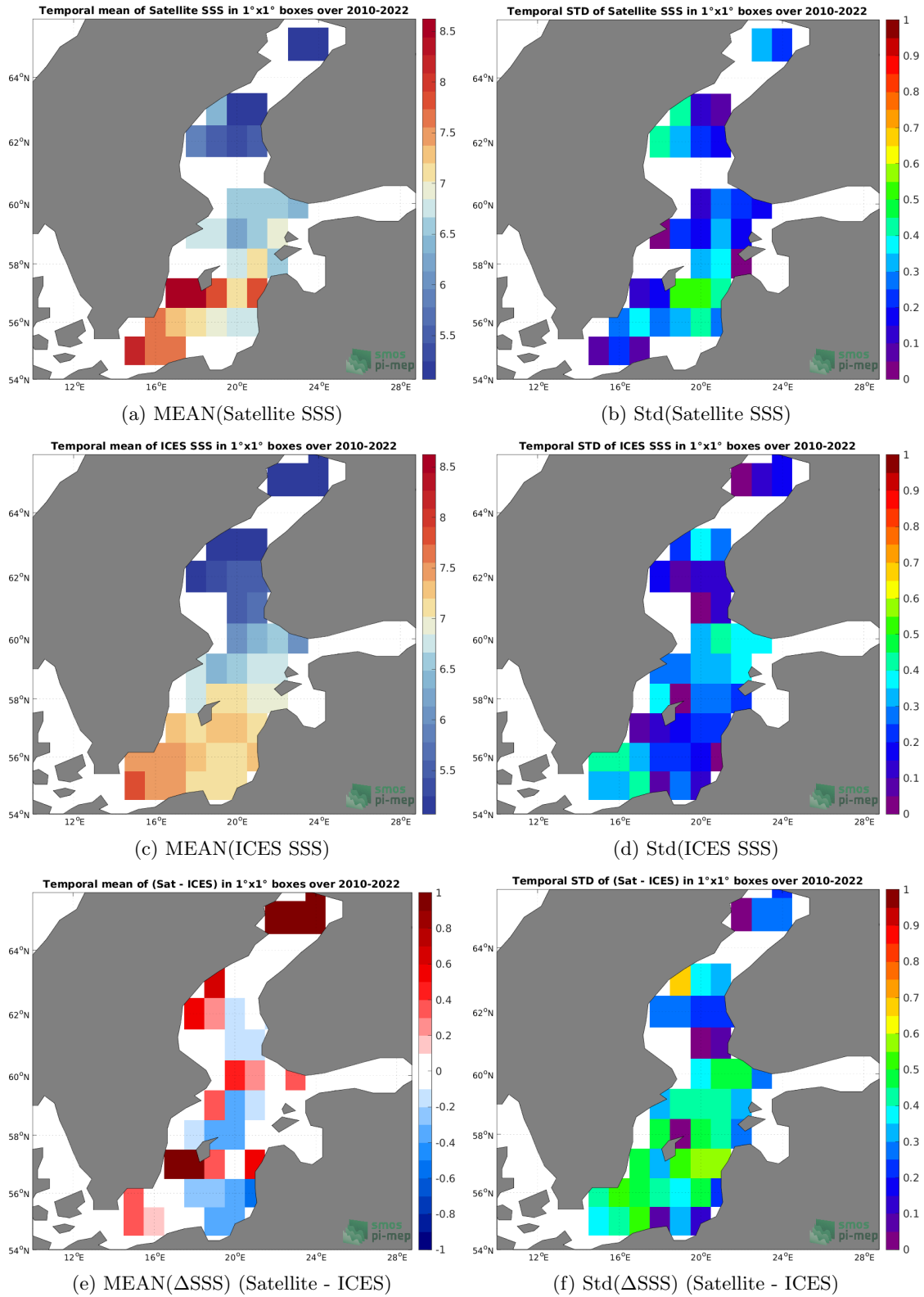
Figure 6: Temporal mean (left) and Std (right) of SSS from SMOS SSS L3 v8 - 18 Days (CATDS-CECOS-LOCEAN) (top), ICES (middle), and of \Delta SSS (Satellite - ICES). Only match-up pairs are used to generate these maps.
