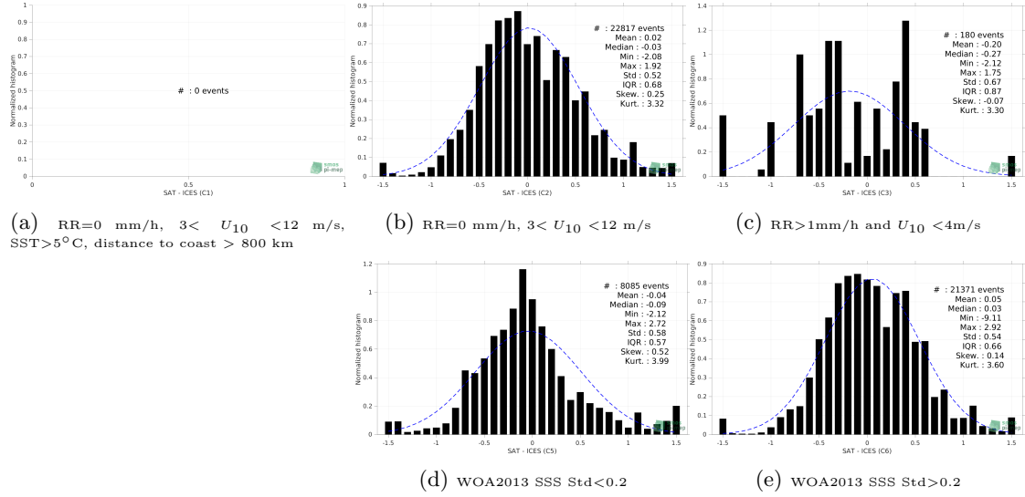
Figure 13: Normalized histogram of \Delta SSS (SMOS SSS L3 v8 - 18 Days (CATDS-CECOS-LOCEAN) - ICES) for 5 different subdatasets corresponding to: RR=0 mm/h, 3 < U_{10} < 12 m/s, SST > 5°C, distance to coast > 800 km (a), RR=0 mm/h, 3 < U_{10} < 12 m/s (b), RR > 1mm/h and U_{10} < 4 m/s (c), WOA2013 SSS Std < 0.2 (d), WOA2013 SSS Std > 0.2 (e).
