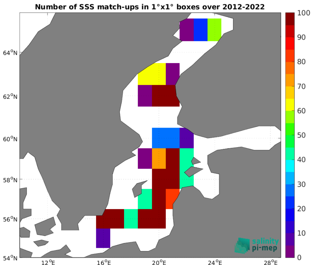
Figure 4: Number of SSS match-ups between Argo SSS and the SMOS SSS L3 v8 - 18 Days (CATDS-CEC-LOCEAN) SSS product for the Baltic Sea Pi-MEP region over 1°×1° boxes and for the full satellite product period.
