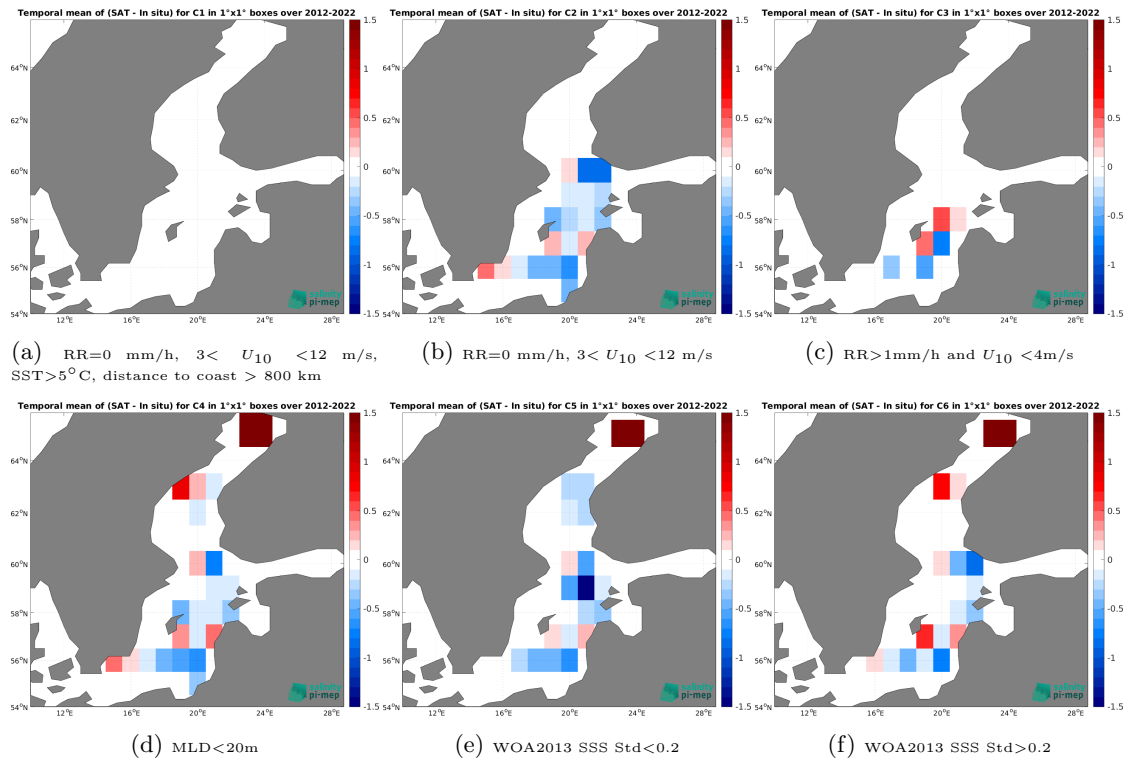
Figure 12: Temporal mean gridded over spatial boxes of size 1^{\circ}\times 1^{\circ} of \Delta\text{SSS} (SMOS SSS L3 v8 - 18 Days (CATDS-CEC-LOCEAN) - Argo) for 6 different subdatasets corresponding to:RR=0 mm/h, 3 < U_{10} < 12 m/s, SST >5^{\circ}\text{C} , distance to coast > 800 km (a), RR=0 mm/h, 3 < U_{10} < 12 m/s (b), RR >1\text{mm/h} and U_{10} < 4\text{m/s} (c),MLD <20\text{m} (d),WOA2013 SSS Std <0.2 (e),WOA2013 SSS Std >0.2 (f).
