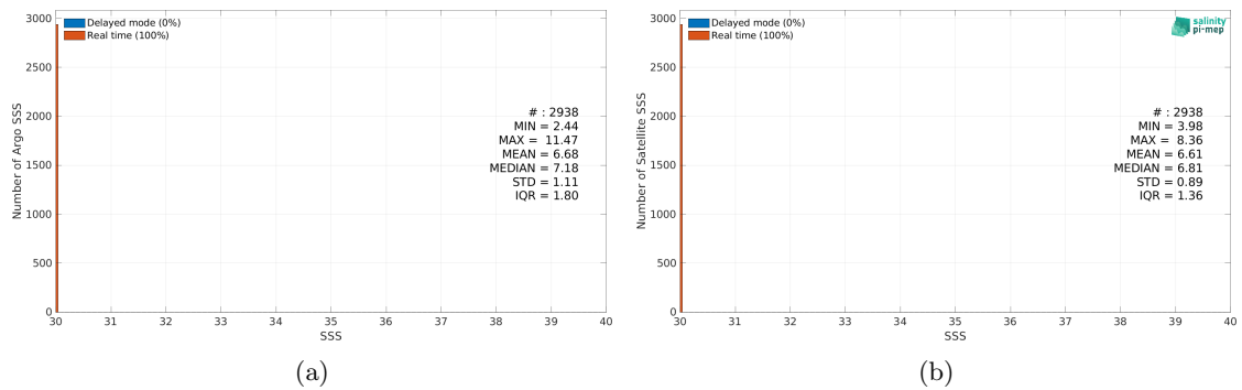
Figure 2: Histograms of SSS from Argo (a) and SMOS SSS L3 v8 - 18 Days (CATDS-CEC-LOCEAN) (b) considering all match-up pairs per bins of 0.1 over the Baltic Sea Pi-MEP region and for the full satellite product period.
