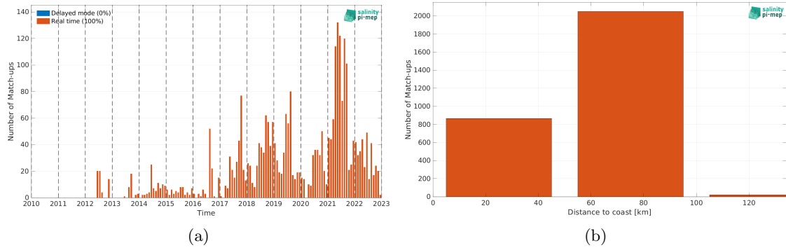
Figure 1: Number of match-ups between Argo and SMOS SSS L3 v8 - 18 Days (CATDS-CEC-LOCEAN) SSS as a function of time (a) and as function of the distance to coast (b) over the Baltic Sea Pi-MEP region and for the full satellite product period.
