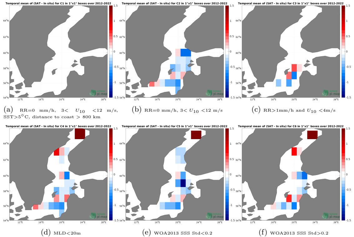
Figure 12: Temporal mean gridded over spatial boxes of size 1^{\circ}\times 1^{\circ} of \Delta\text{SSS} (SMOS SSS L3 v8 - 18 Days (CATDS-CECOS-LOCEAN) - Argo) for 6 different subdatasets corresponding to:RR=0 mm/h, 3 < U_{10} < 12 m/s, SST >5^{\circ}\text{C} , distance to coast > 800 km (a), RR=0 mm/h, 3 < U_{10} < 12 m/s (b), RR >1 mm/h and U_{10} < 4 m/s (c),MLD <20 m (d),WOA2013 SSS Std <0.2 (e),WOA2013 SSS Std >0.2 (f).
