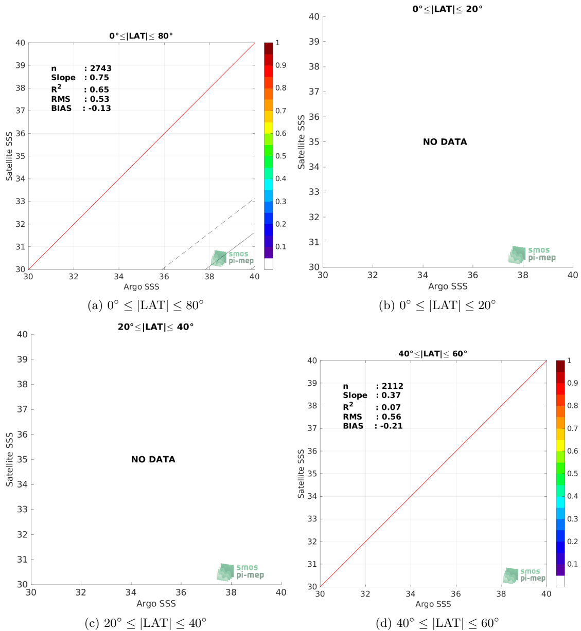
Figure 9: Contour maps of the concentration of SMOS SSS L3 v8 - 18 Days (CATDS-CECOS-LOCEAN) SSS (y-axis) versus Argo SSS (x-axis) at match-up pairs for different latitude bands. For each plot, the red line shows x=y . The black thin and dashed lines indicate a linear fit through the data cloud and the \pm 95\% confidence levels, respectively. The number match-up pairs n , the slope and R^2 coefficient of the linear fit, the root mean square (RMS) and the mean bias between satellite and in situ data are indicated for each latitude band in each plots.
