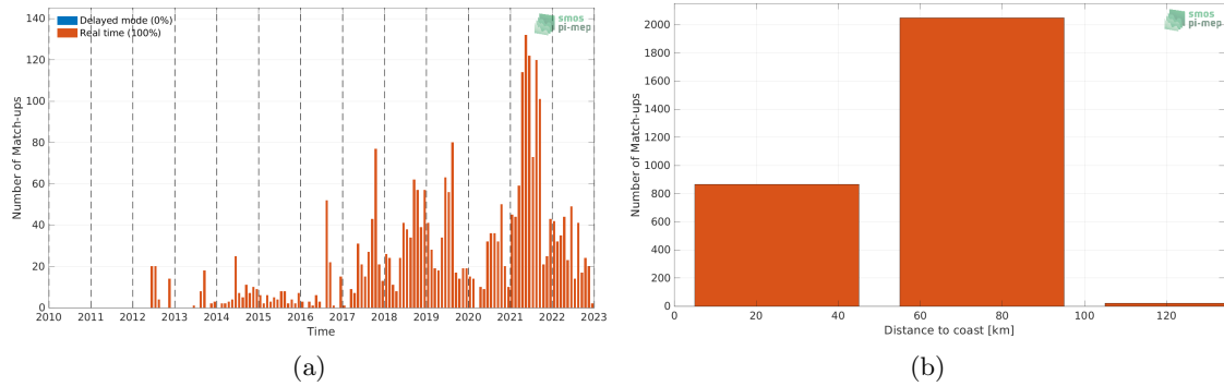
Figure 1: Number of match-ups between Argo and SMOS SSS L3 v8 - 18 Days (CATDS-CECOS-LOCEAN) SSS as a function of time (a) and as function of the distance to coast (b) over the Baltic Sea Pi-MEP region and for the full satellite product period.
