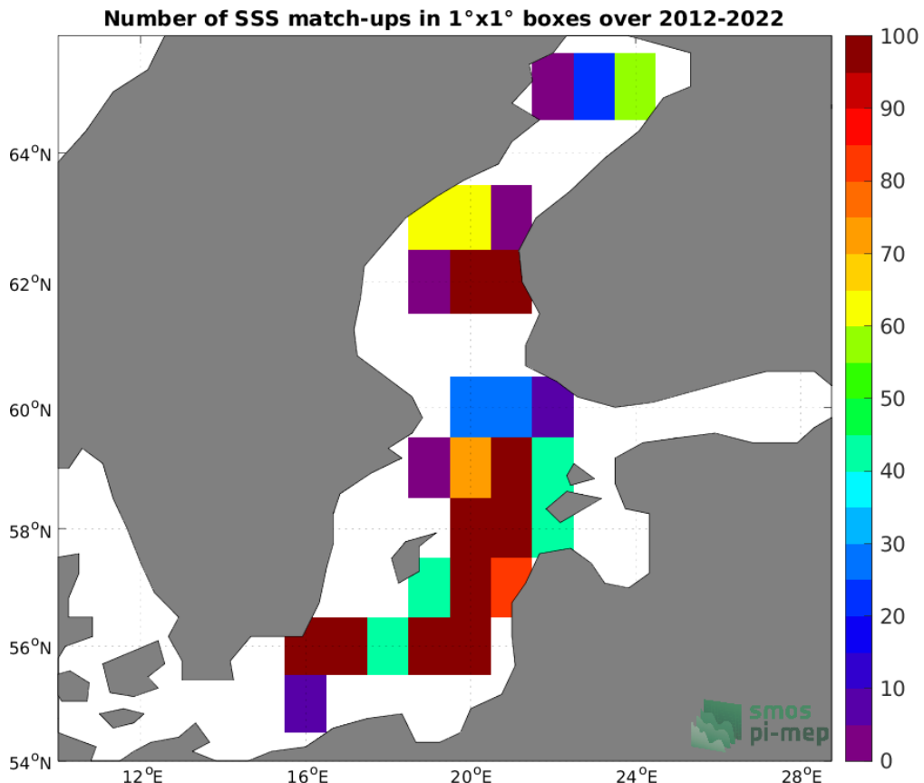
Figure 4: Number of SSS match-ups between Argo SSS and the SMOS SSS L3 v8 - 18 Days (CATDS-CECOS-LOCEAN) SSS product for the Baltic Sea Pi-MEP region over 1°x1° boxes and for the full satellite product period.
