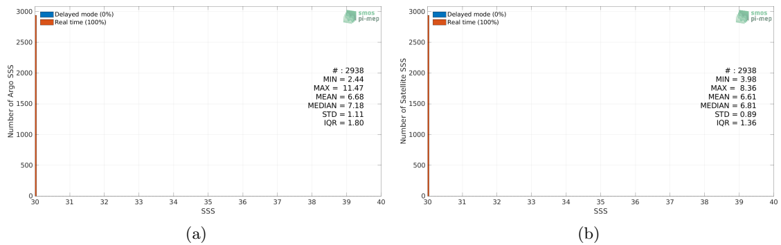
Figure 2: Histograms of SSS from Argo (a) and SMOS SSS L3 v8 - 18 Days (CATDS-CECOS-LOCEAN) (b) considering all match-up pairs per bins of 0.1 over the Baltic Sea Pi-MEP region and for the full satellite product period.
