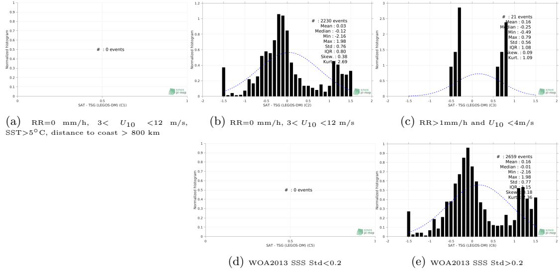
Figure 13: Normalized histogram of \Delta\text{SSS} (SMOS SSS L3 v7 - 9 Days (CATDS-CECOS-LOCEAN) - TSG (LEGOS-DM)) for 5 different subdatasets corresponding to: RR=0 mm/h, 3 < U_{10} < 12 m/s, SST > 5^\circ\text{C} , distance to coast > 800 km (a), RR=0 mm/h, 3 < U_{10} < 12 m/s (b), RR > 1\text{mm/h} and U_{10} < 4\text{m/s} (c), WOA2013 SSS Std < 0.2 (d), WOA2013 SSS Std > 0.2 (e).
