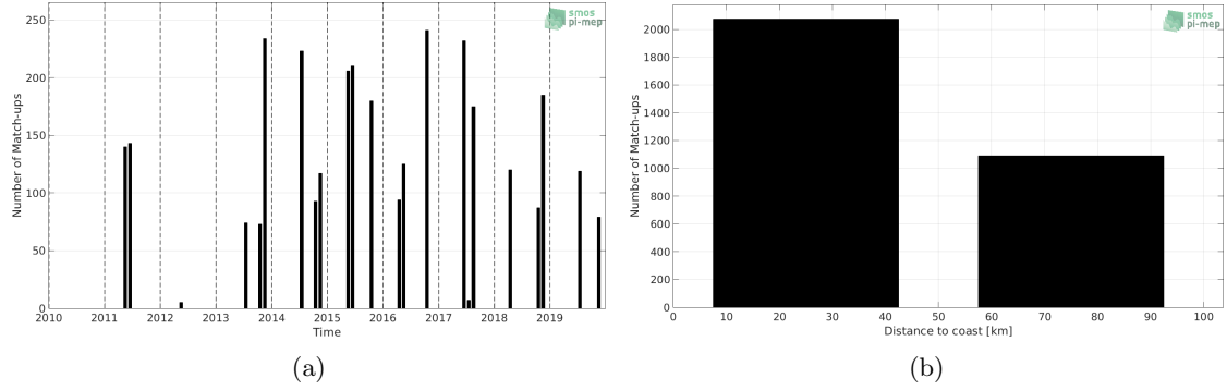
Figure 1: Number of match-ups between TSG (LEGOS-DM) and SMOS SSS L3 v7 - 9 Days (CATDS-CECOS-LOCEAN) SSS as a function of time (a) and as function of the distance to coast (b) over the Baltic Sea Pi-MEP region and for the full satellite product period.
