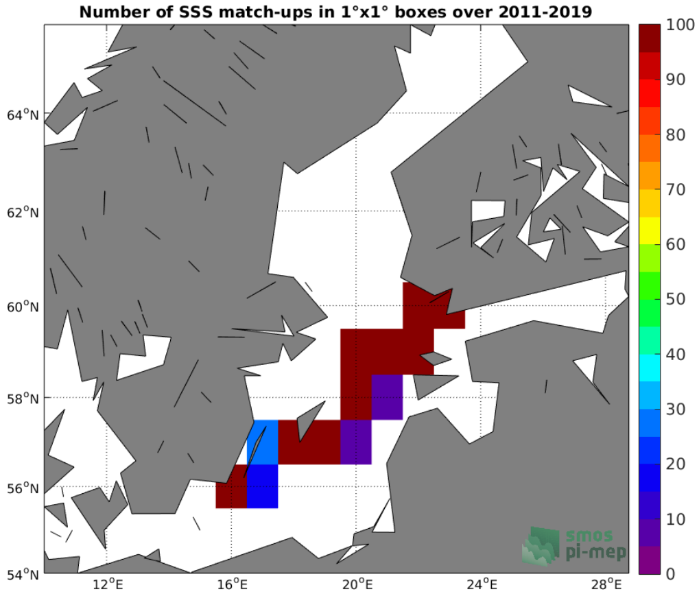
Figure 4: Number of SSS match-ups between TSG (LEGOS-DM) SSS and the SMOS SSS L3 v7 - 9 Days (CATDS-CECOS-LOCEAN) SSS product for the Baltic Sea Pi-MEP region over 1°x1° boxes and for the full satellite product period.
