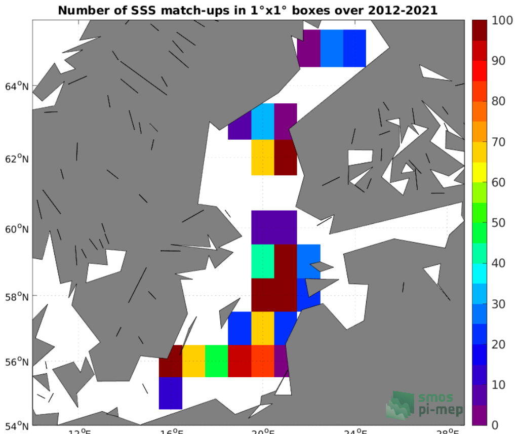
Figure 4: Number of SSS match-ups between Argo SSS and the SMOS SSS L3 v7 - 9 Days (CATDS-CECOS-LOCEAN) SSS product for the Baltic Sea Pi-MEP region over 1°x1° boxes and for the full satellite product period.
