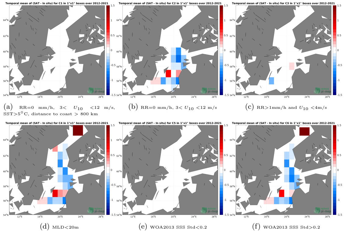
Figure 12: Temporal mean gridded over spatial boxes of size 1^{\circ}\times 1^{\circ} of \Delta\text{SSS} (SMOS SSS L3 v7 - 9 Days (CATDS-CECOS-LOCEAN) - Argo) for 6 different subdatasets corresponding to:RR=0 mm/h, 3 < U_{10} < 12 m/s, SST >5^{\circ}\text{C} , distance to coast > 800 km (a), RR=0 mm/h, 3 < U_{10} < 12 m/s (b), RR >1\text{mm/h} and U_{10} < 4\text{m/s} (c),MLD <20\text{m} (d),WOA2013 SSS Std <0.2 (e),WOA2013 SSS Std >0.2 (f).
