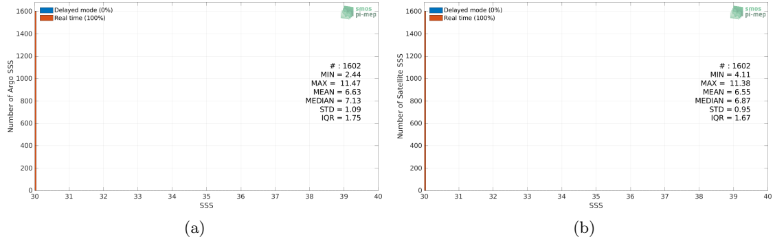
Figure 2: Histograms of SSS from Argo (a) and SMOS SSS L3 v7 - 9 Days (CATDS-CECOS-LOCEAN) (b) considering all match-up pairs per bins of 0.1 over the Baltic Sea Pi-MEP region and for the full satellite product period.
