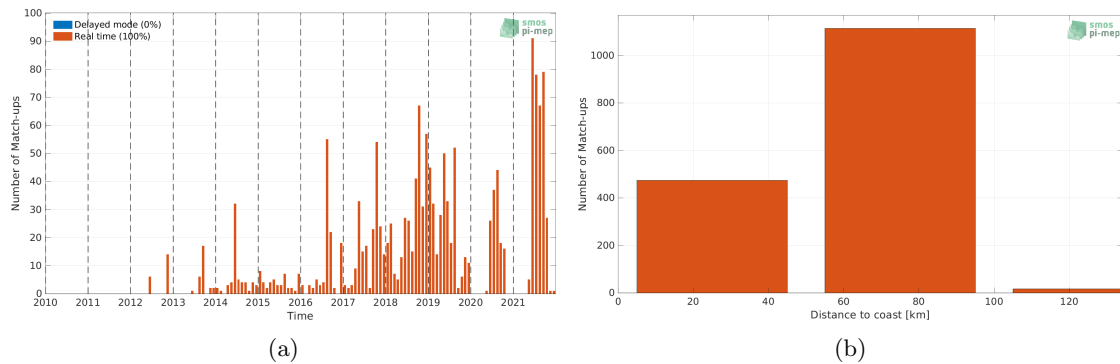
Figure 1: Number of match-ups between Argo and SMOS SSS L3 v7 - 9 Days (CATDS-CECOS-LOCEAN) SSS as a function of time (a) and as function of the distance to coast (b) over the Baltic Sea Pi-MEP region and for the full satellite product period.
