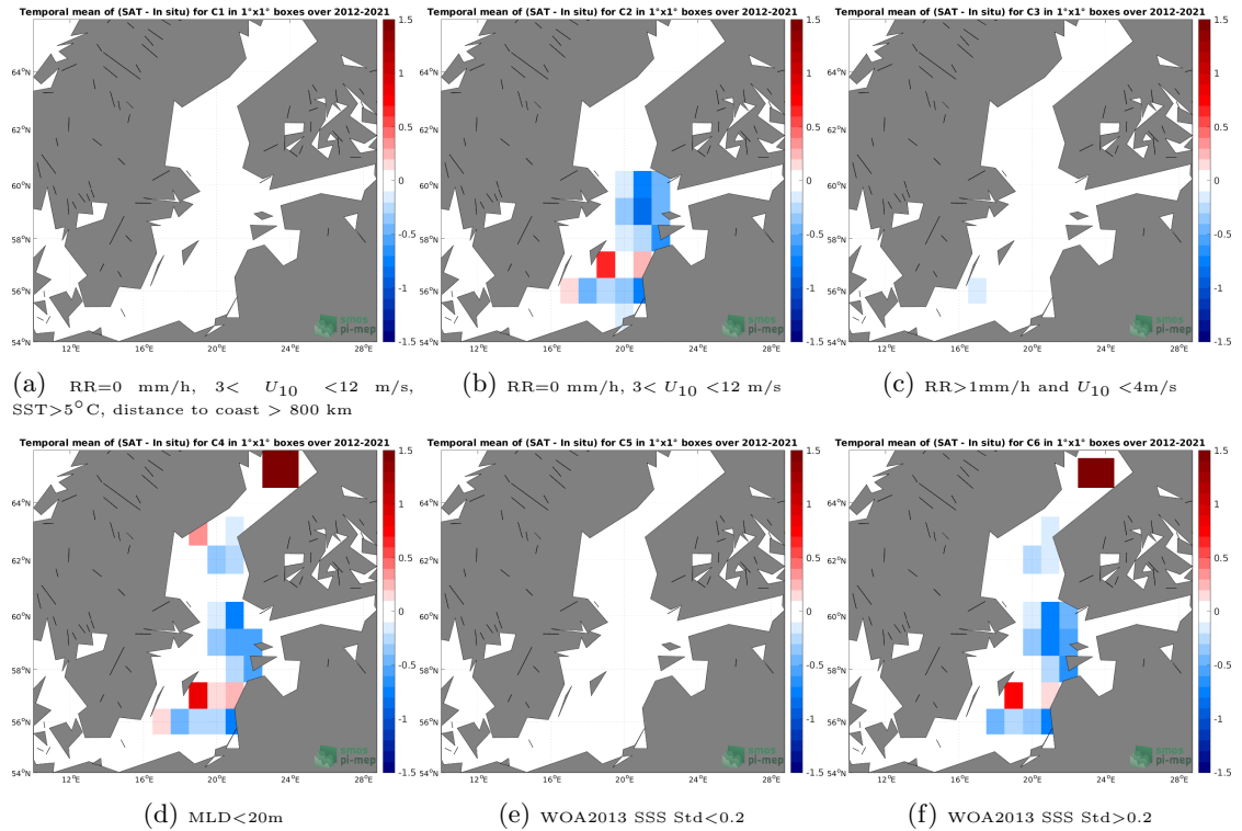
Figure 12: Temporal mean gridded over spatial boxes of size 1^{\circ}\times 1^{\circ} of \Delta\text{SSS} (SMOS SSS L3 v7 - 18 Days (CATDS-CECOS-LOCEAN) - Argo) for 6 different subdatasets corresponding to:RR=0 mm/h, 3 < U_{10} < 12 m/s, SST >5^{\circ}\text{C} , distance to coast > 800 km (a), RR=0 mm/h, 3 < U_{10} < 12 m/s (b), RR >1\text{mm/h} and U_{10} < 4\text{m/s} (c),MLD <20\text{m} (d),WOA2013 SSS Std <0.2 (e),WOA2013 SSS Std >0.2 (f).
