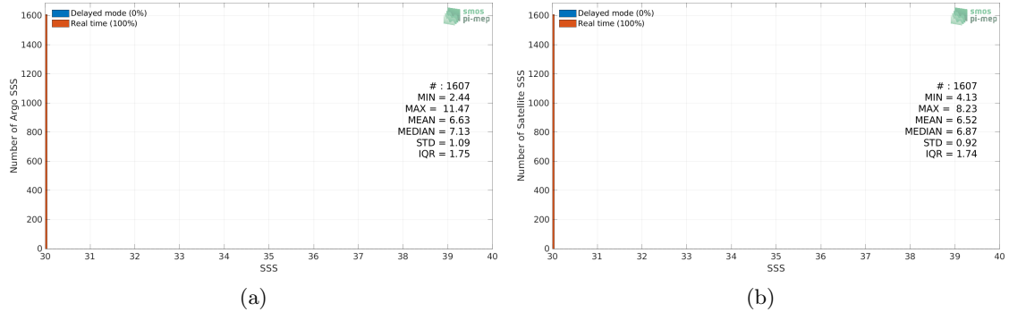
Figure 2: Histograms of SSS from Argo (a) and SMOS SSS L3 v7 - 18 Days (CATDS-CECOS-LOCEAN) (b) considering all match-up pairs per bins of 0.1 over the Baltic Sea Pi-MEP region and for the full satellite product period.
