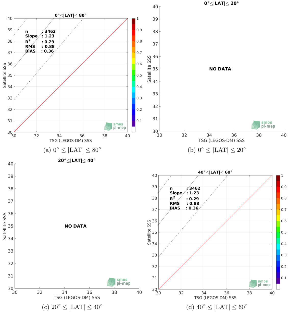
Figure 9: Contour maps of the concentration of SMOS SSS L3 v5 - 9 Days (CATDS-CECOS-LOCEAN) SSS (y-axis) versus TSG (LEGOS-DM) SSS (x-axis) at match-up pairs for different latitude bands. For each plot, the red line shows x=y . The black thin and dashed lines indicate a linear fit through the data cloud and the \pm 95\% confidence levels, respectively. The number match-up pairs n , the slope and R^2 coefficient of the linear fit, the root mean square (RMS) and the mean bias between satellite and in situ data are indicated for each latitude band in each plots.
