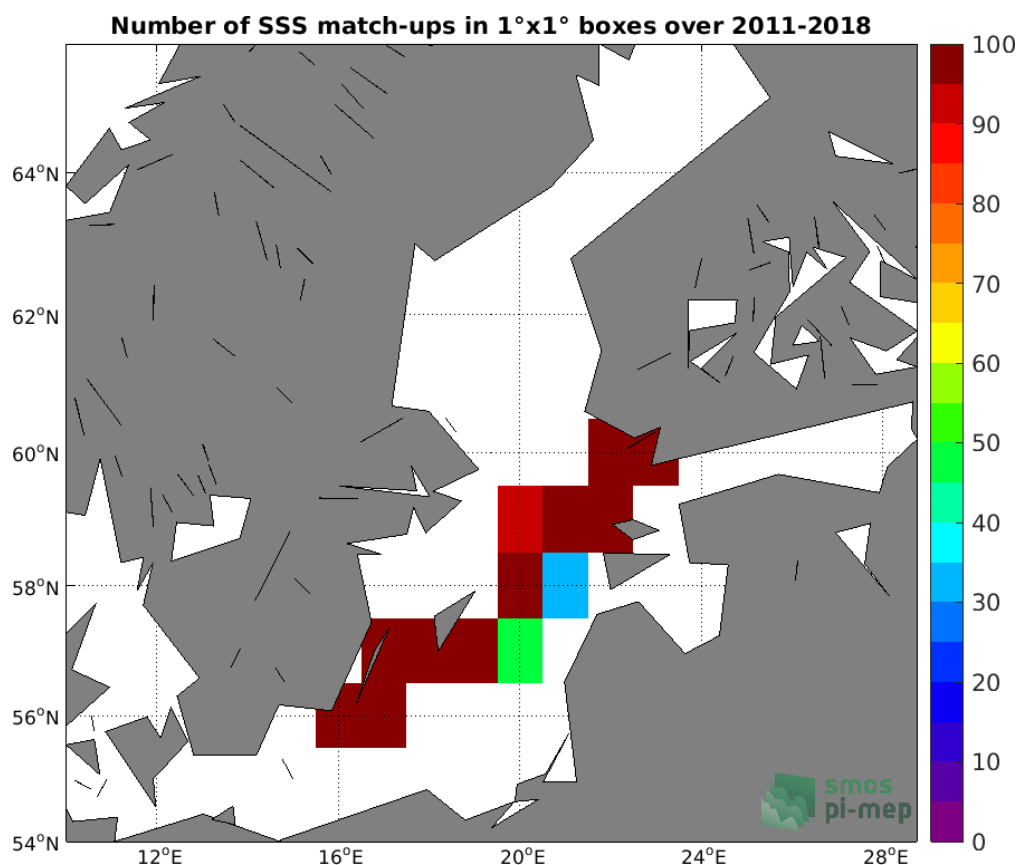
Figure 4: Number of SSS match-ups between TSG (LEGOS-DM) SSS and the SMOS SSS L3 v5 - 9 Days (CATDS-CECOS-LOCEAN) SSS product for the Baltic Sea Pi-MEP region over 1°x1° boxes and for the full satellite product period.
