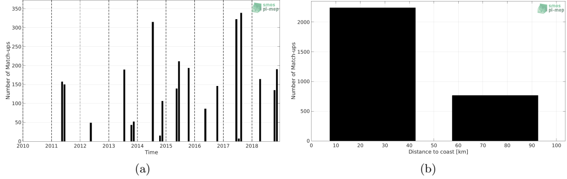
Figure 1: Number of match-ups between TSG (LEGOS-DM) and SMOS SSS L3 v5 - 9 Days (CATDS-CECOS-LOCEAN) SSS as a function of time (a) and as function of the distance to coast (b) over the Baltic Sea Pi-MEP region and for the full satellite product period.
