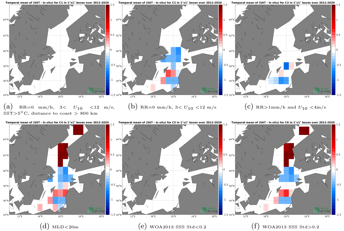
Figure 12: Temporal mean gridded over spatial boxes of size 1^{\circ} \times 1^{\circ} of \Delta\text{SSS} (SMOS SSS L3 v5 - 9 Days (CATDS-CECOS-LOCEAN) - Argo) for 6 different subdatasets corresponding to: RR=0 mm/h, 3 < U_{10} < 12 m/s, SST >5^{\circ}\text{C} , distance to coast > 800 km (a), RR=0 mm/h, 3 < U_{10} < 12 m/s (b), RR >1\text{mm/h} and U_{10} < 4\text{m/s} (c), MLD <20\text{m} (d), WOA2013 SSS Std <0.2 (e), WOA2013 SSS Std >0.2 (f).
