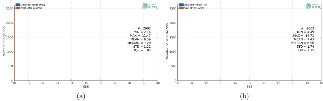
Figure 2: Histograms of SSS from Argo (a) and SMOS SSS L3 v5 - 9 Days (CATDS-CECOS-LOCEAN) (b) considering all match-up pairs per bins of 0.1 over the Baltic Sea Pi-MEP region and for the full satellite product period.
