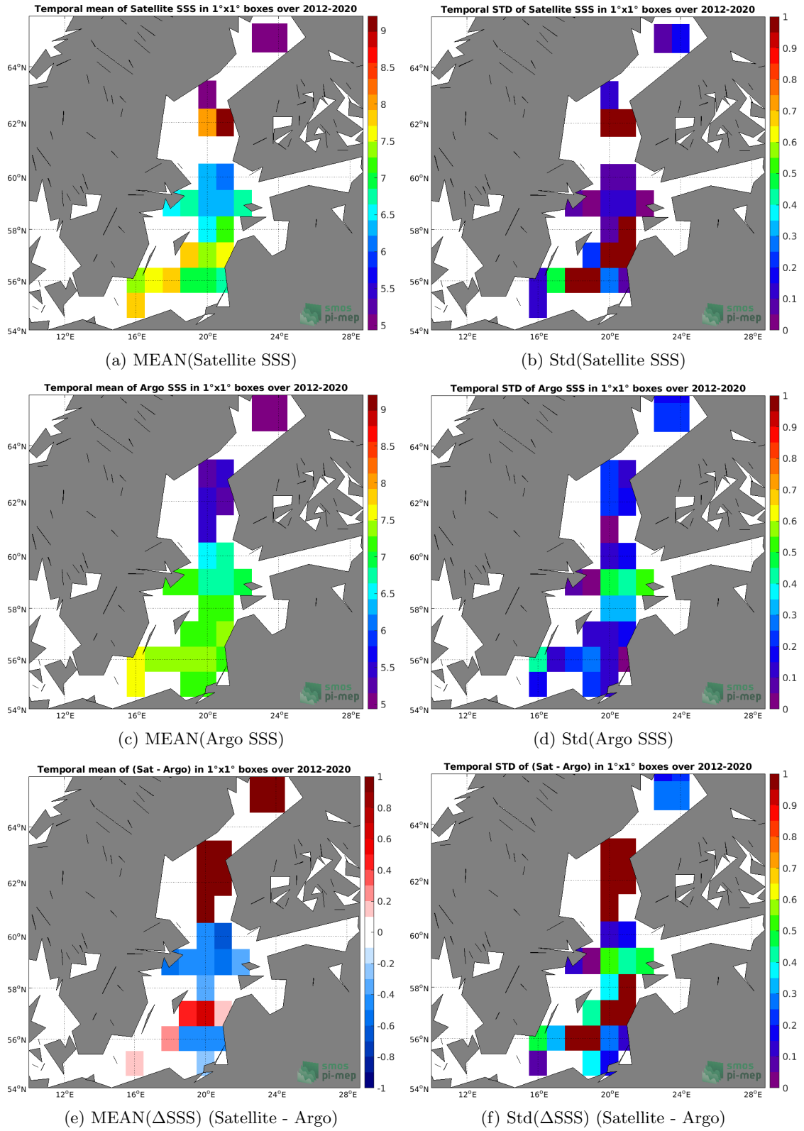
Figure 6: Temporal mean (left) and Std (right) of SSS from SMOS SSS L3 v5 - 9 Days (CATDS-CECOS-LOCEAN) (top), Argo (middle), and of \Delta SSS (Satellite - Argo). Only match-up pairs are used to generate these maps.
