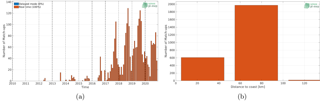
Figure 1: Number of match-ups between Argo and SMOS SSS L3 v5 - 9 Days (CATDS-CECOS-LOCEAN) SSS as a function of time (a) and as function of the distance to coast (b) over the Baltic Sea Pi-MEP region and for the full satellite product period.
