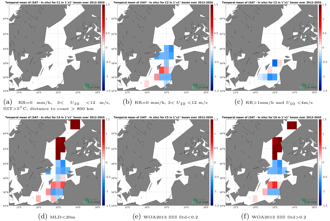
Figure 12: Temporal mean gridded over spatial boxes of size 1^{\circ}\times 1^{\circ} of \Delta\text{SSS} (SMOS SSS L3 v5 - 9 Days (CATDS-CECOS-LOCEAN) - Argo) for 6 different subdatasets corresponding to:RR=0 mm/h, 3 < U_{10} < 12 m/s, SST >5^{\circ}\text{C} , distance to coast > 800 km (a), RR=0 mm/h, 3 < U_{10} < 12 m/s (b), RR >1\text{mm/h} and U_{10} < 4\text{m/s} (c),MLD <20\text{m} (d),WOA2013 SSS Std <0.2 (e),WOA2013 SSS Std >0.2 (f).
