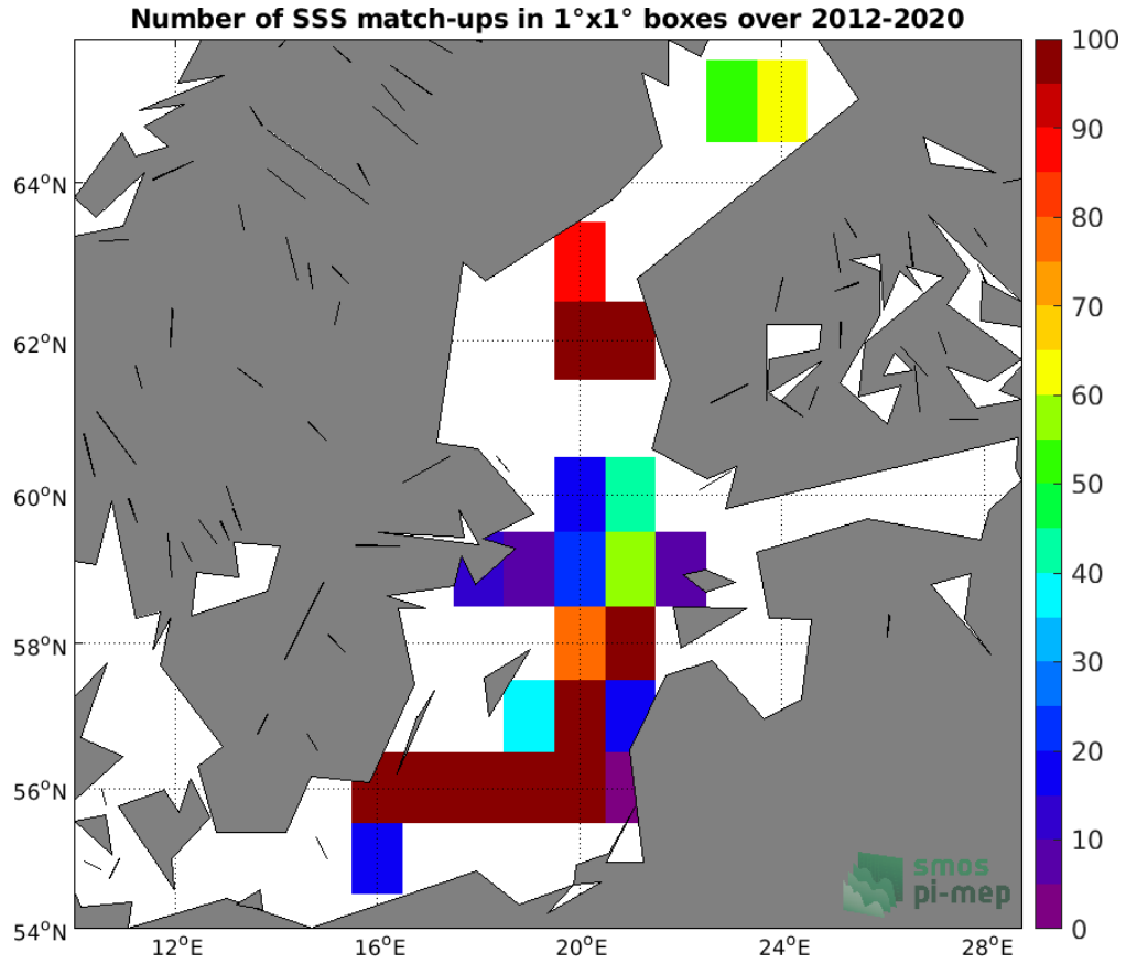
Figure 4: Number of SSS match-ups between Argo SSS and the SMOS SSS L3 v5 - 9 Days (CATDS-CECOS-LOCEAN) SSS product for the Baltic Sea Pi-MEP region over 1°x1° boxes and for the full satellite product period.
