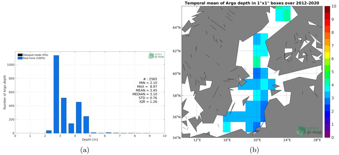
Figure 3: Histograms of the depth of the upper level SSS measurements from Argo in the Match-up DataBase for the Baltic Sea Pi-MEP region (a) and temporal mean spatial distribution of pressure of the in situ SSS data over 1°x1° boxes and for the full satellite product period (b).
