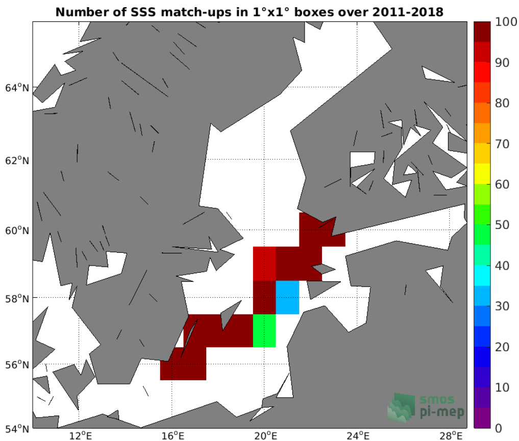
Figure 4: Number of SSS match-ups between TSG (LEGOS-DM) SSS and the SMOS SSS L3 v5 - 18 Days (CATDS-CECOS-LOCEAN) SSS product for the Baltic Sea Pi-MEP region over 1°x1° boxes and for the full satellite product period.
