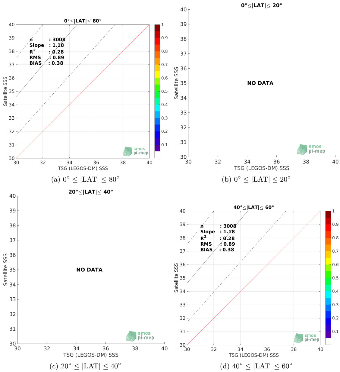
Figure 9: Contour maps of the concentration of SMOS SSS L3 v5 - 18 Days (CATDS-CECOS-LOCEAN) SSS ( y -axis) versus TSG (LEGOS-DM) SSS ( x -axis) at match-up pairs for different latitude bands. For each plot, the red line shows x=y . The black thin and dashed lines indicate a linear fit through the data cloud and the \pm 95\% confidence levels, respectively. The number match-up pairs n , the slope and R^2 coefficient of the linear fit, the root mean square (RMS) and the mean bias between satellite and in situ data are indicated for each latitude band in each plots.
