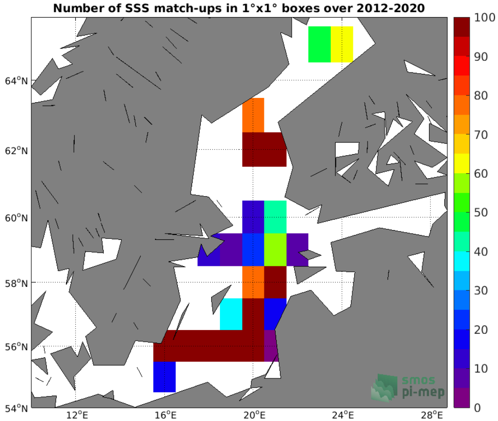
Figure 4: Number of SSS match-ups between Argo SSS and the SMOS SSS L3 v5 - 18 Days (CATDS-CECOS-LOCEAN) SSS product for the Baltic Sea Pi-MEP region over 1°x1° boxes and for the full satellite product period.
