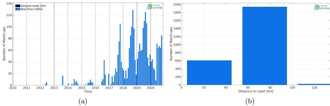
Figure 1: Number of match-ups between Argo and SMOS SSS L3 v5 - 18 Days (CATDS-CECOS-LOCEAN) SSS as a function of time (a) and as function of the distance to coast (b) over the Baltic Sea Pi-MEP region and for the full satellite product period.
