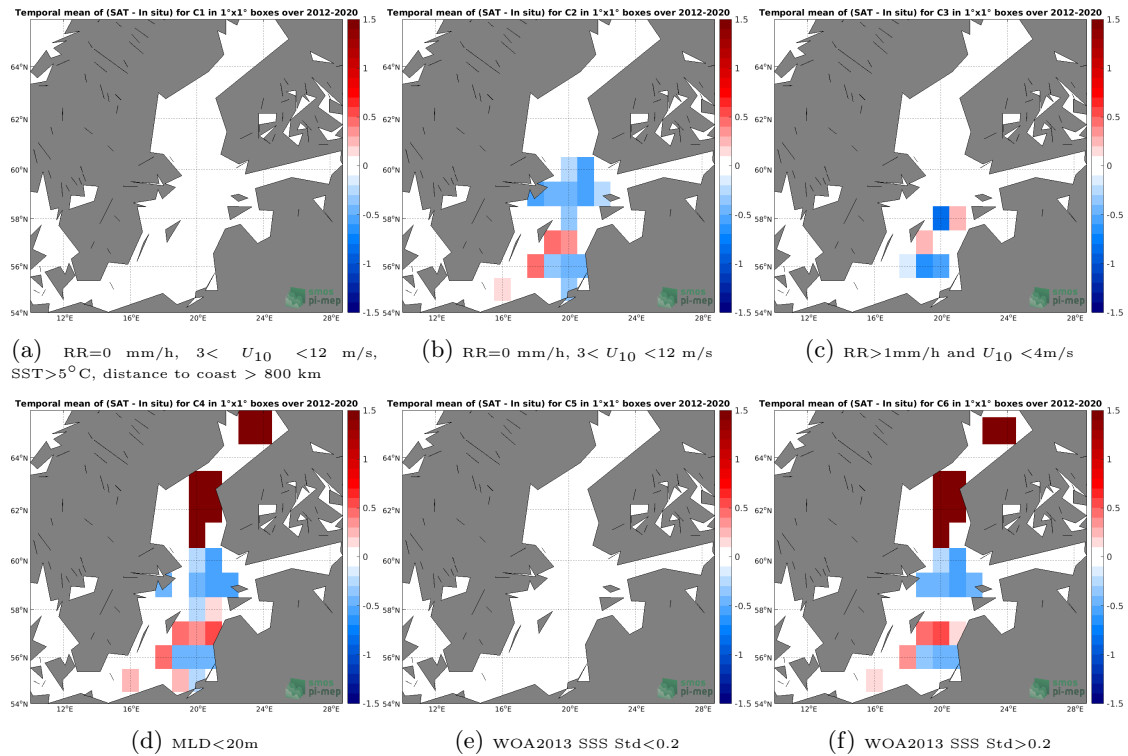
Figure 12: Temporal mean gridded over spatial boxes of size 1^{\circ}\times 1^{\circ} of \Delta\text{SSS} (SMOS SSS L3 v5 - 18 Days (CATDS-CECOS-LOCEAN) - Argo) for 6 different subdatasets corresponding to:RR=0 mm/h, 3 < U_{10} < 12 m/s, SST >5^{\circ}\text{C} , distance to coast > 800 km (a), RR=0 mm/h, 3 < U_{10} < 12 m/s (b), RR >1 mm/h and U_{10} < 4 m/s (c),MLD <20 m (d),WOA2013 SSS Std <0.2 (e),WOA2013 SSS Std >0.2 (f).
