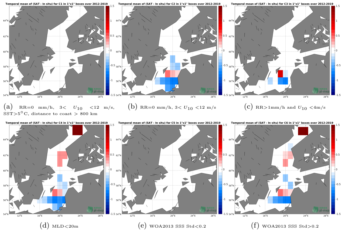
Figure 12: Temporal mean gridded over spatial boxes of size 1^{\circ}\times 1^{\circ} of \Delta\text{SSS} (SMOS-L3-CATDS-CECOS-LOCEAN-V4-9DAYS-25KM - Argo) for 6 different subdatasets corresponding to:RR=0 mm/h, 3 < U_{10} < 12 m/s, SST >5^{\circ}\text{C} , distance to coast > 800 km (a), RR=0 mm/h, 3 < U_{10} < 12 m/s (b), RR >1\text{mm/h} and U_{10} < 4\text{m/s} (c),MLD <20\text{m} (d),WOA2013 SSS Std <0.2 (e),WOA2013 SSS Std >0.2 (f).
