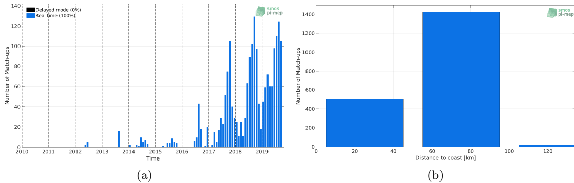
Figure 1: Number of match-ups between Argo and SMOS-L3-CATDS-CECOS-LOCEAN-V4-9DAYS-25KM SSS as a function of time (a) and as function of the distance to coast (b) over the Baltic Sea Pi-MEP region and for the full satellite product period.
