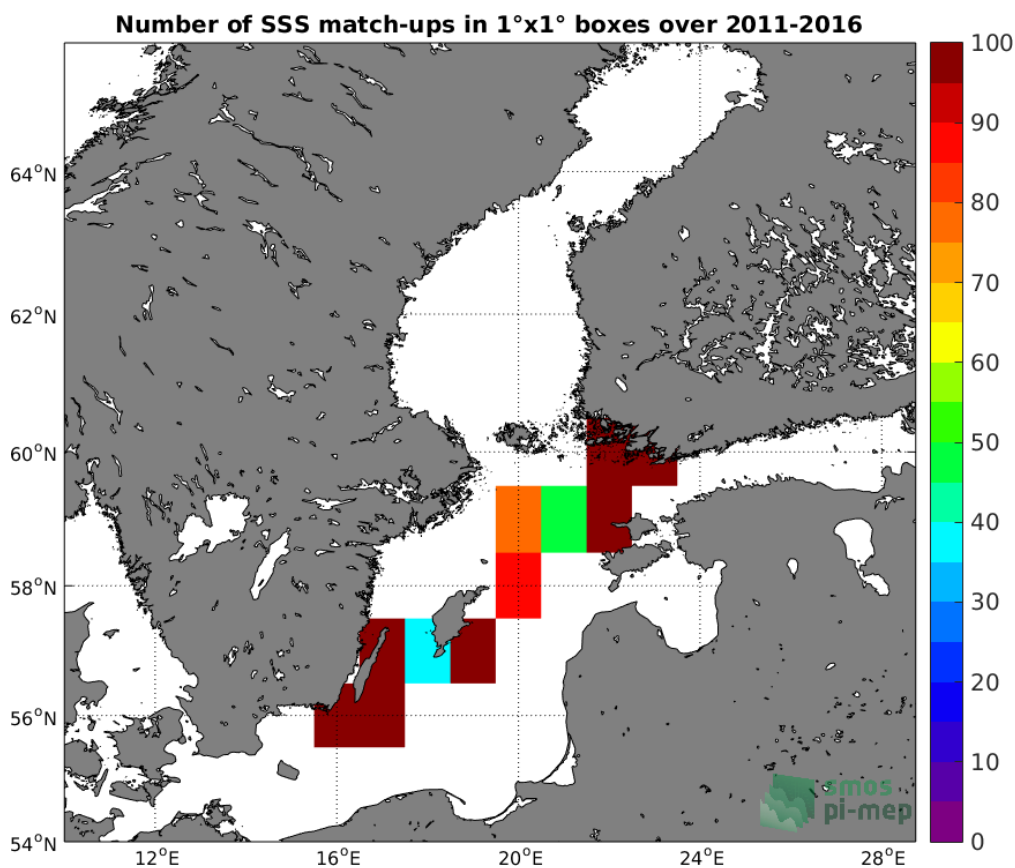
Figure 4: Number of SSS match-ups between TSG-LEGOS-DM SSS and the SMOS-L3-CATDS-CECOS-LOCEAN-V3-9DAYS-25KM SSS product for the Baltic Sea Pi-MEP region over 1°x1° boxes and for the full satellite product period.
