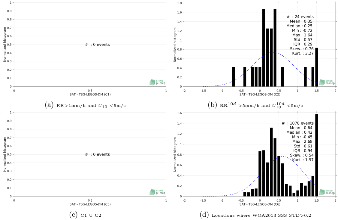
Figure 13: Normalized histogram of \Delta\text{SSS} (SMOS-L3-CATDS-CECOS-LOCEAN-V3-9DAYS-25KM - TSG-LEGOS-DM) for 6 different subdatasets corresponding to: RR > 1\text{mm/h} and U_{10} < 5\text{m/s} (a), RR^{10d} > 5\text{mm/h} and U_{10}^{10d} < 5\text{m/s} (b), C1 \cup C2 (c), Locations where WOA2013 SSS STD > 0.2 (d).
