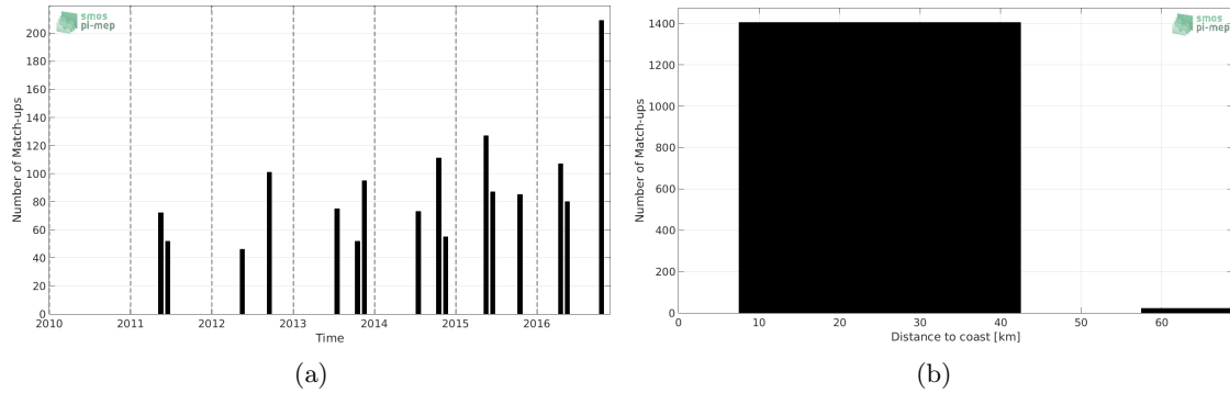
Figure 1: Number of match-ups between TSG-LEGOS-DM and SMOS-L3-CATDS-CECOS-LOCEAN-V3-9DAYS-25KM SSS as a function of time (a) and as function of the distance to coast (b) over the Baltic Sea Pi-MEP region and for the full satellite product period.
