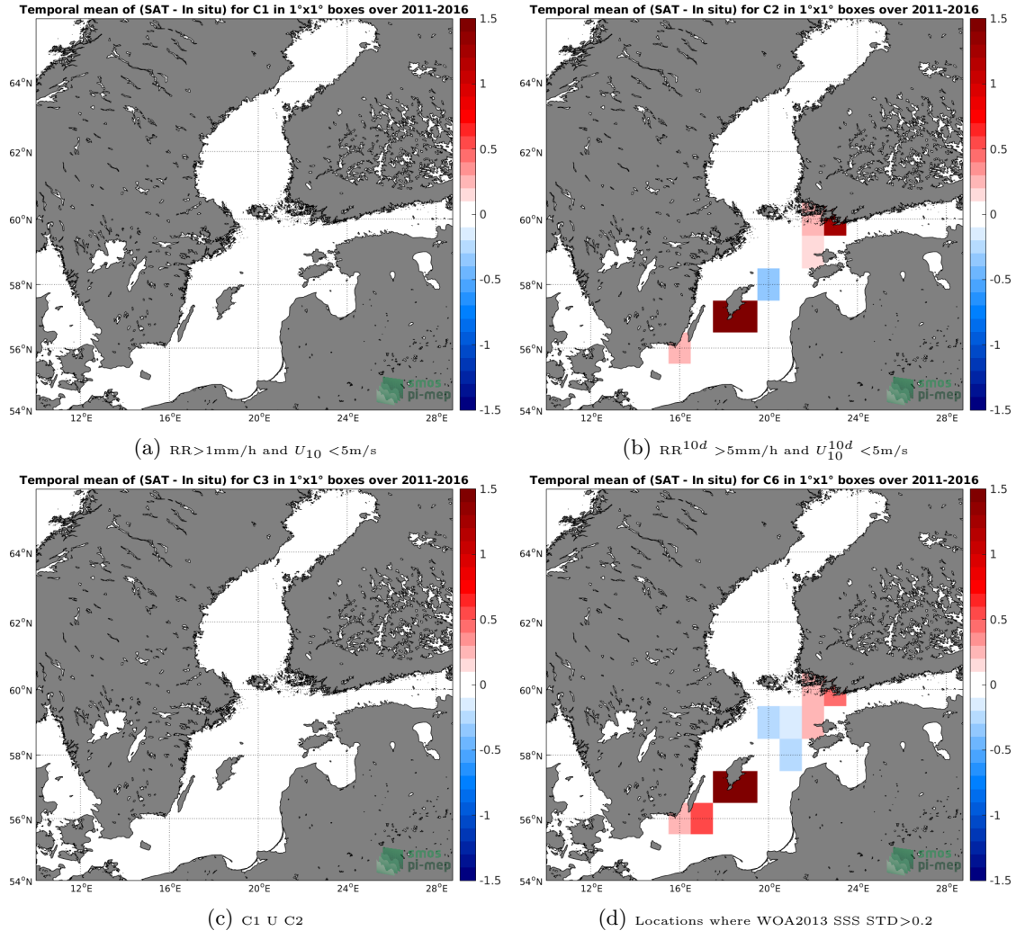
Figure 12: Temporal mean gridded over spatial boxes of size 1^\circ \times 1^\circ of \Delta SSS (SMOS-L3-CATDS-CECOS-LOCEAN-V3-9DAYS-25KM - TSG-LEGOS-DM) for 4 different subdatasets corresponding to: RR > 1\text{mm/h} and U_{10} < 5\text{m/s} (a), RR^{10d} > 5\text{mm/h} and U_{10}^{10d} < 5\text{m/s} (b), C1 U C2 (c), Locations where WOA2013 SSS STD > 0.2 (d).
