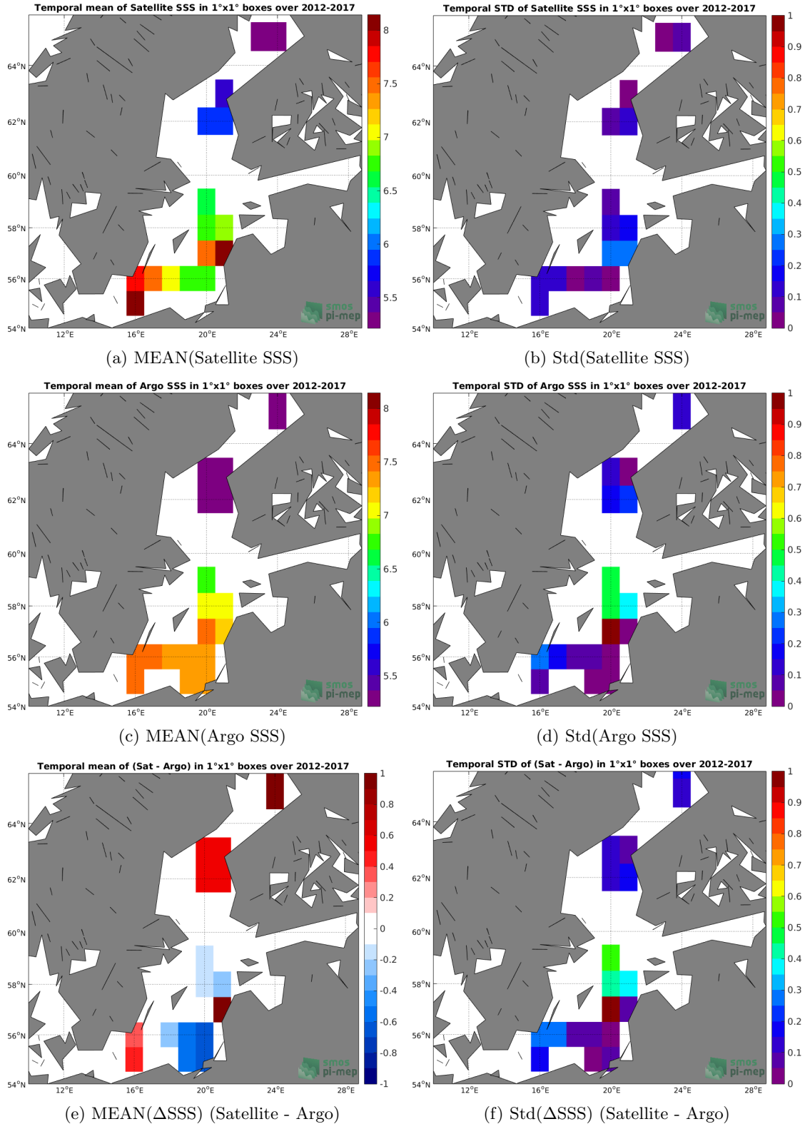
Figure 6: Temporal mean (left) and Std (right) of SSS from SMOS-L3-CATDS-CECOS-LOCEAN-V3-9DAYS-25KM (top), Argo (middle), and of \Delta SSS (Satellite - Argo). Only match-up pairs are used to generate these maps.
