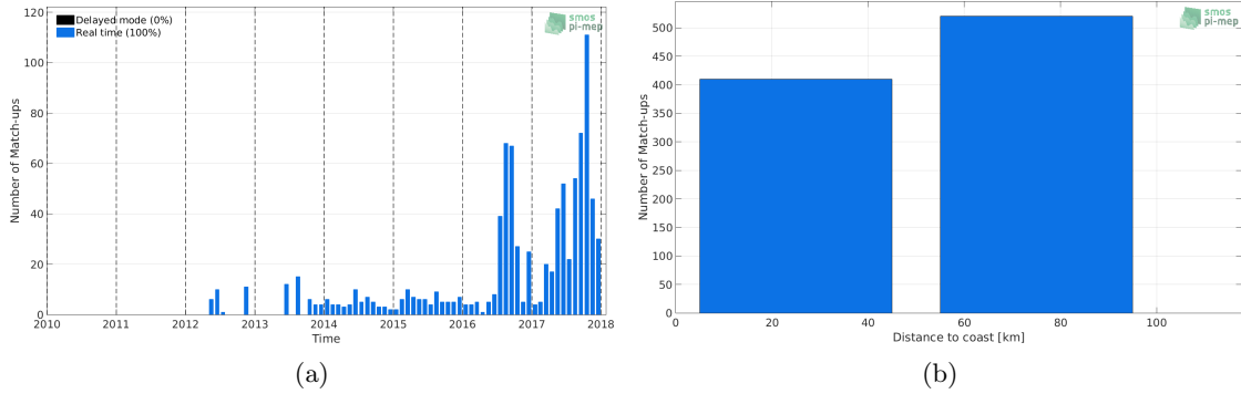
Figure 1: Number of match-ups between Argo and SMOS-L3-CATDS-CECOS-LOCEAN-V3-9DAYS-25KM SSS as a function of time (a) and as function of the distance to coast (b) over the Baltic Sea Pi-MEP region and for the full satellite product period.
