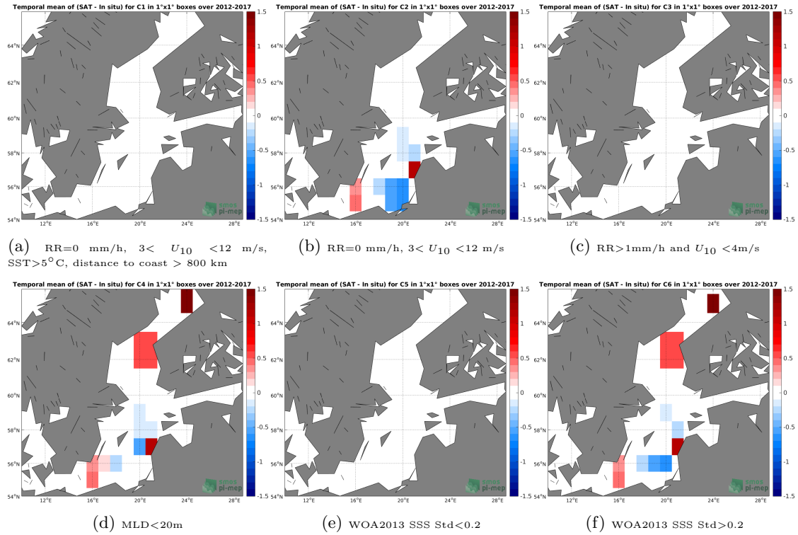
Figure 12: Temporal mean gridded over spatial boxes of size 1^\circ \times 1^\circ of \Delta SSS (SMOS-L3-CATDS-CECOS-LOCEAN-V3-9DAYS-25KM - Argo) for 6 different subdatasets corresponding to: RR=0 mm/h, 3 < U_{10} < 12 m/s, SST >5^\circ\text{C} , distance to coast > 800 km (a), RR=0 mm/h, 3 < U_{10} < 12 m/s (b), RR >1 mm/h and U_{10} < 4 m/s (c),MLD <20 m (d),WOA2013 SSS Std <0.2 (e),WOA2013 SSS Std >0.2 (f).
