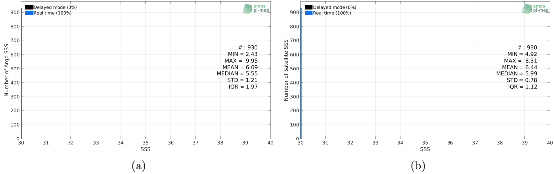
Figure 2: Histograms of SSS from Argo (a) and SMOS-L3-CATDS-CECOS-LOCEAN-V3-9DAYS-25KM (b) considering all match-up pairs per bins of 0.1 over the Baltic Sea Pi-MEP region and for the full satellite product period.
