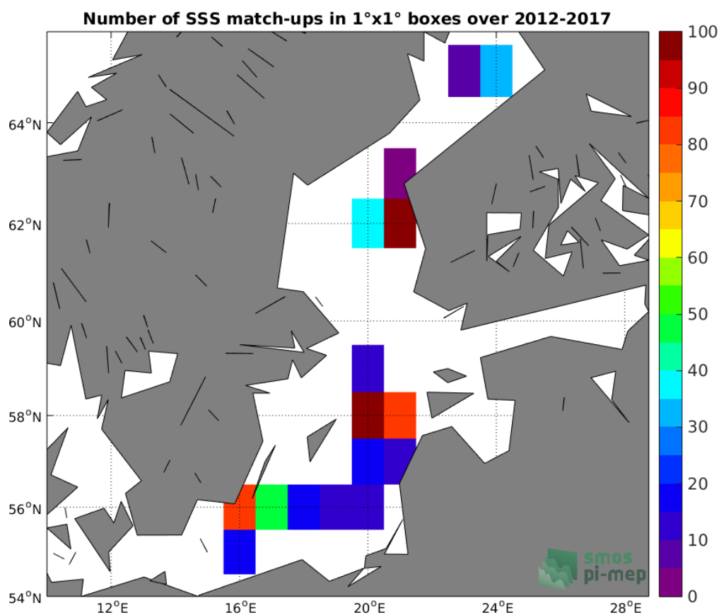
Figure 4: Number of SSS match-ups between Argo SSS and the SMOS-L3-CATDS-CECOS-LOCEAN-V3-9DAYS-25KM SSS product for the Baltic Sea Pi-MEP region over 1°x1° boxes and for the full satellite product period.
