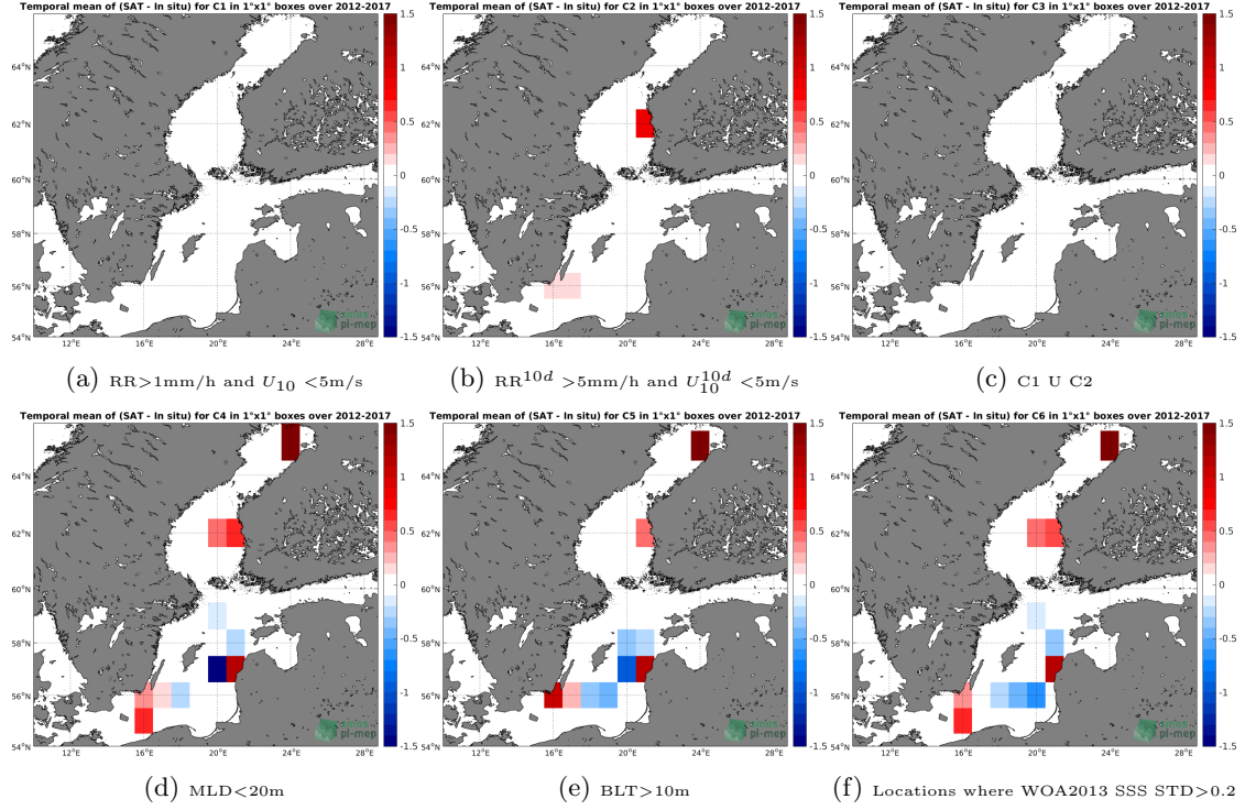
Figure 12: Temporal mean gridded over spatial boxes of size 1^\circ \times 1^\circ of \Delta\text{SSS} (SMOS-L3-CATDS-CECOS-LOCEAN-V3-9DAYS-25KM - Argo) for 6 different subdatasets corresponding to: \text{RR} > 1\text{mm/h} and U_{10} < 5\text{m/s} (a), \text{RR}^{10d} > 5\text{mm/h} and U_{10}^{10d} < 5\text{m/s} (b), C1 U C2 (c), \text{MLD} < 20\text{m} (d), \text{BLT} > 10\text{m} (e), Locations where WOA2013 SSS STD > 0.2 (f).
